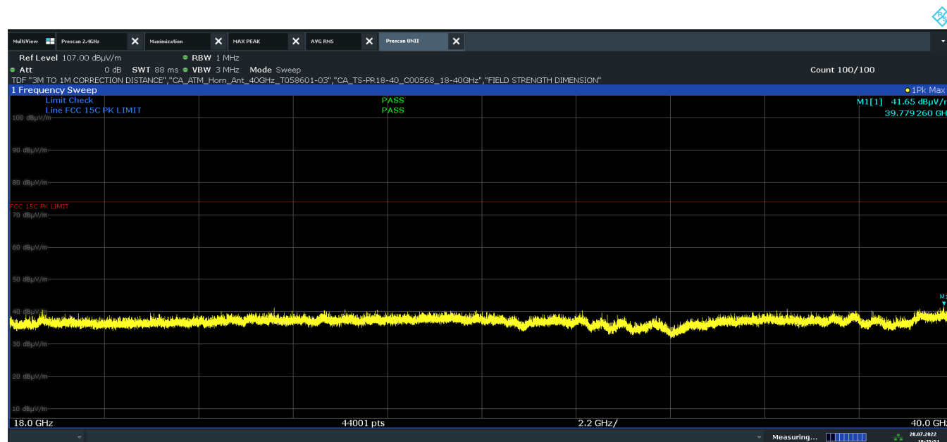
Plot 7-21. Radiated Spurious Emissions Above 18GHz (BDR GFSK – 5844MHz Pol. H)
