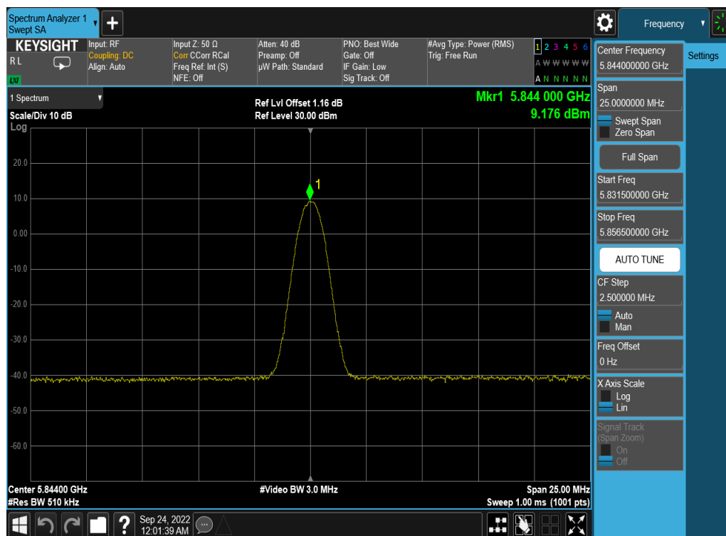
Plot 7-12. PSD (BDR GFSK – 5844MHz)
