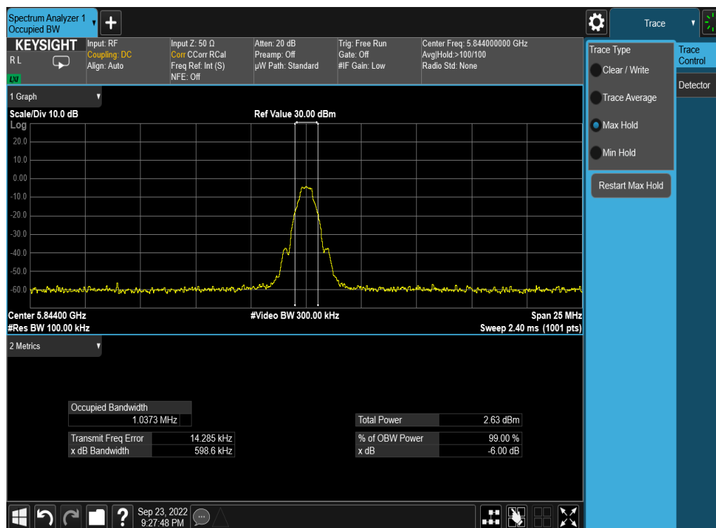
Plot 7-6. 6dB BW & 99% OBW (BDR, 5844MHz)
