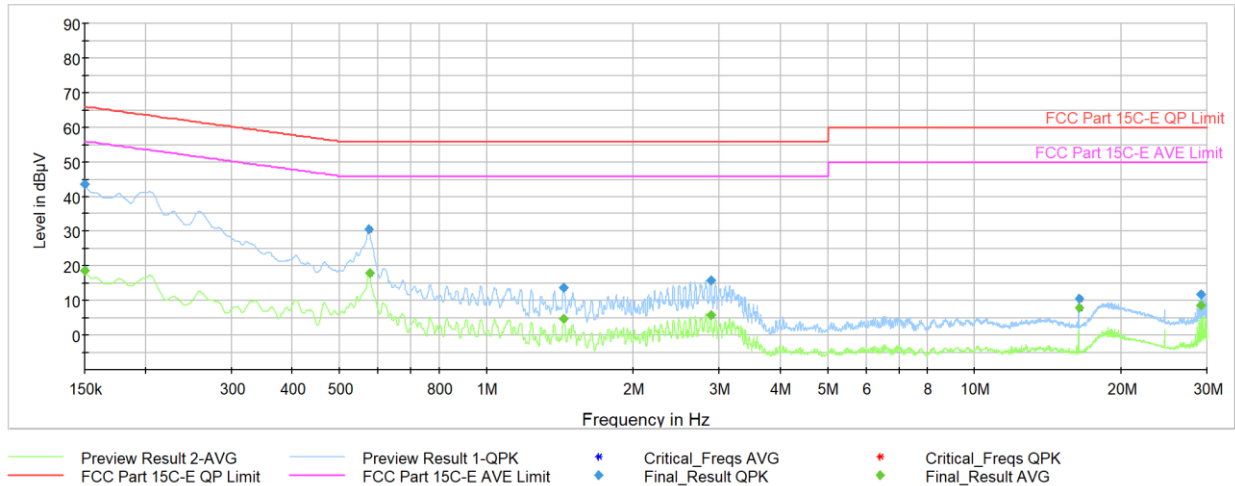
Plot 7-29. AC Line Conducted Plot (BDR GFSK – 5157MHz) (N) with host PC and lightning cable
