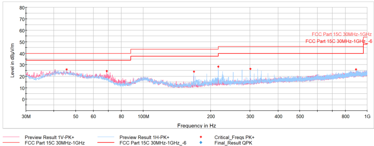
Plot 7-26. Radiated Spurious Emissions Below 1GHz (BDR GFSK – 5157MHz), with AC/DC Adapter and lightning cable
