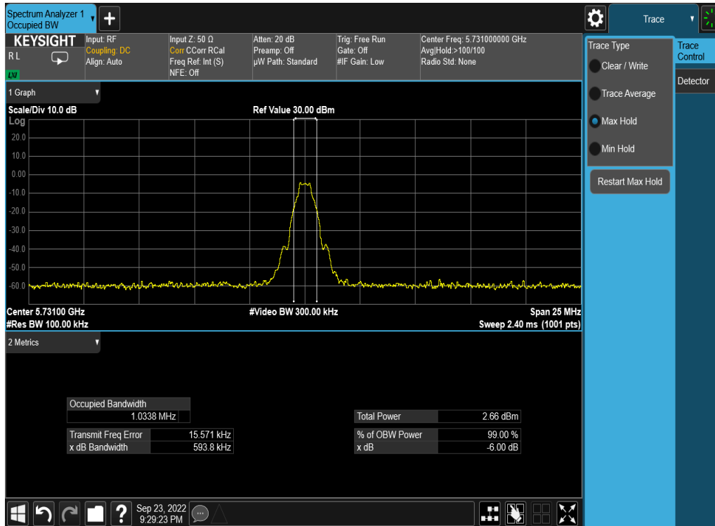
Plot 7-4. 6dB BW & 99% OBW (BDR, 5731MHz)
