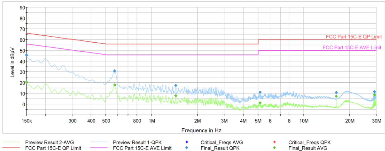
Plot 7-28. AC Line Conducted Plot (BDR GFSK – 5157MHz) (L1) with host PC and lightning cable
