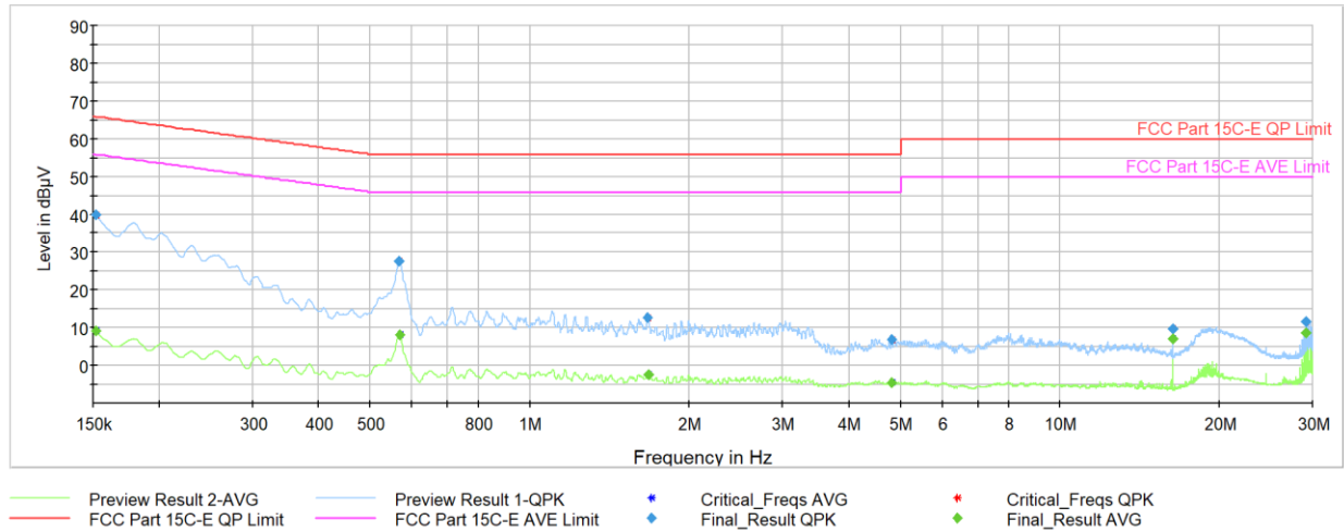
Plot 7-30. AC Line Conducted Plot (BDR GFSK – 5844MHz) (L1) with host PC and lightning cable
