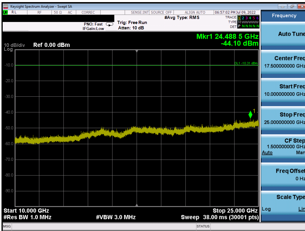
Plot 7-36. Conducted Spurious Plot (Bluetooth (HDRp4), 4 Mbps – Ch. 38)
