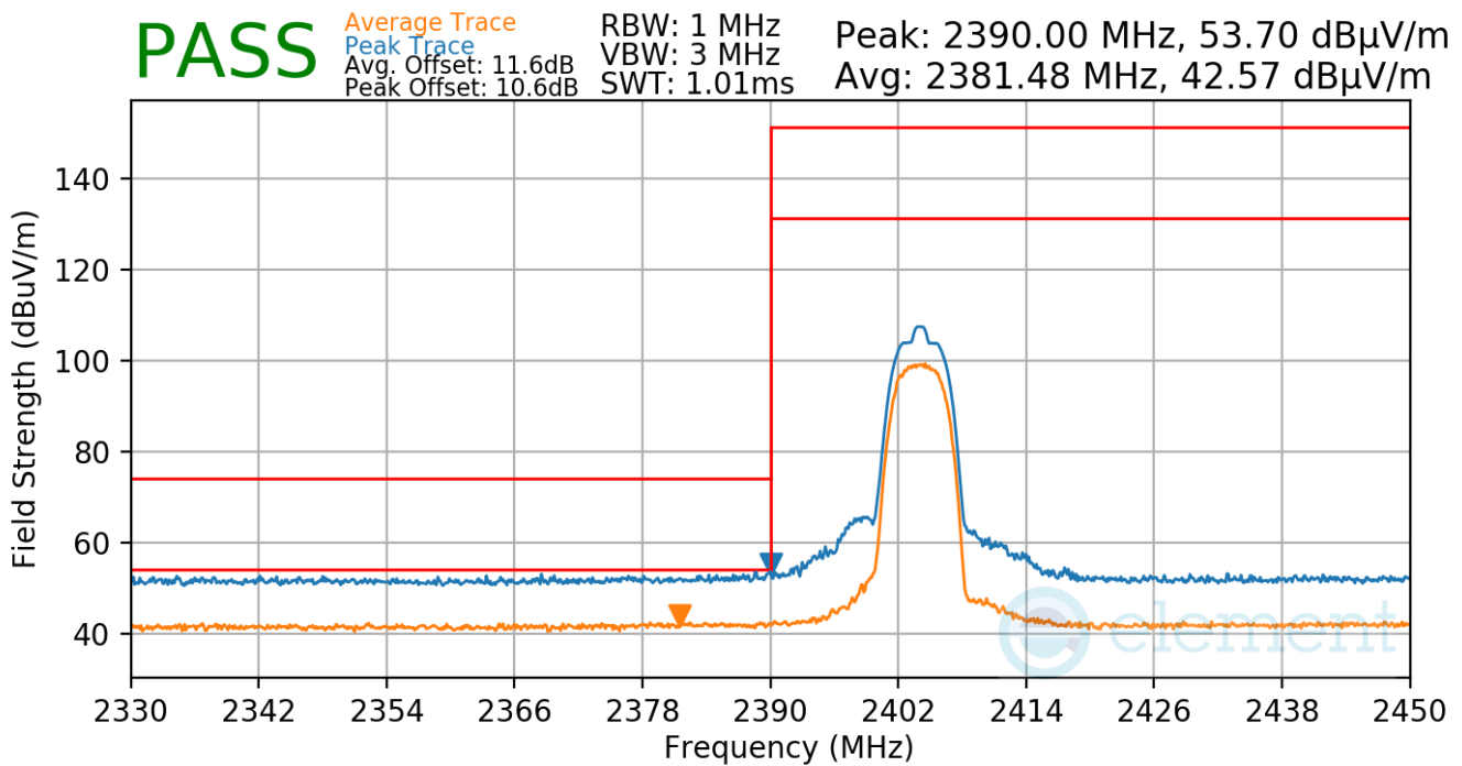
Plot 7-45. Radiated Restricted Lower Band Edge Measurement
