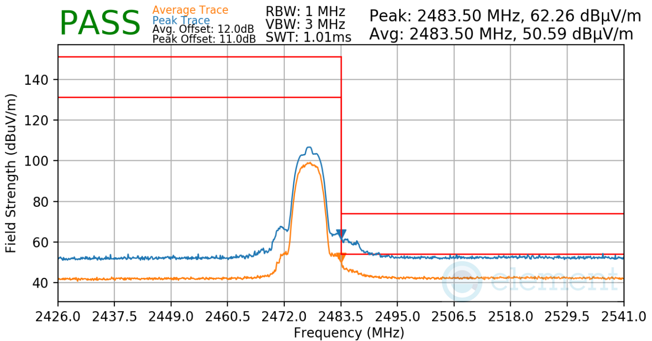
Plot 7-49. Radiated Restricted Upper Band Edge Measurement
