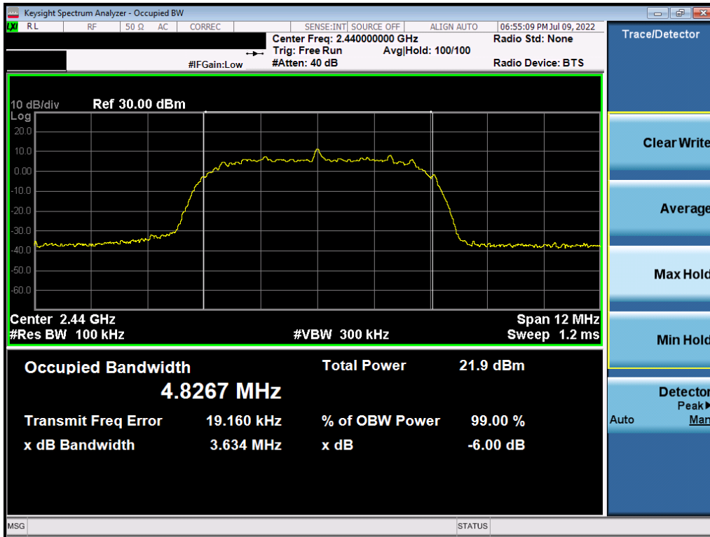
Plot 7-11. 6dB BW & 99% OBW Plot (Bluetooth (HDRp8), 8Mbps – Ch. 38)
