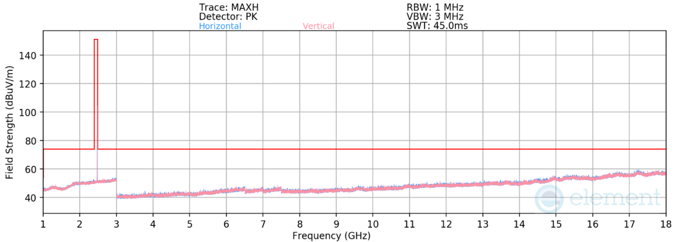
Plot 7-41. Radiated Spurious Emissions 1-18GHz (4Mbps, HDR4 – Ch. 75)
