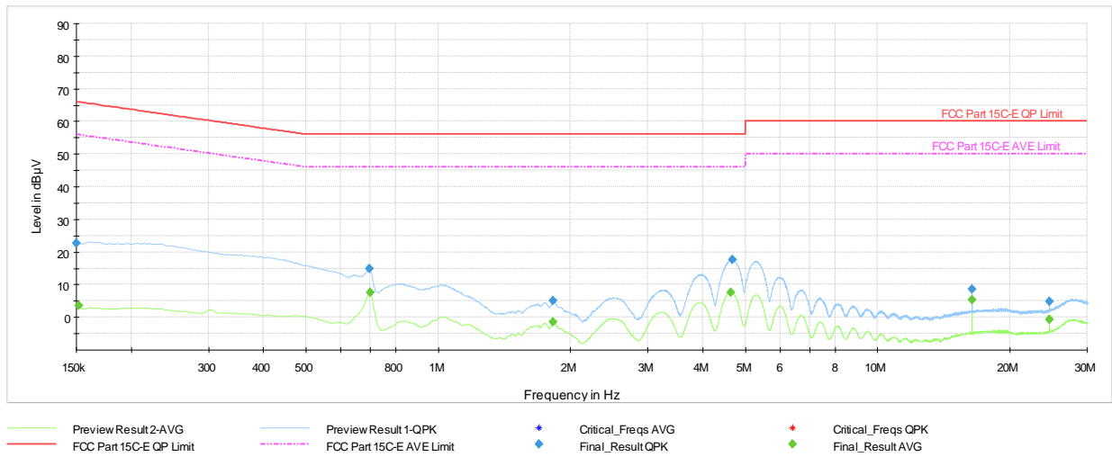
Plot 7-55. AC Line Conducted Plot with Bluetooth HDR (N, 4Mbps - Ch.75 with AC/DC Adapter)
