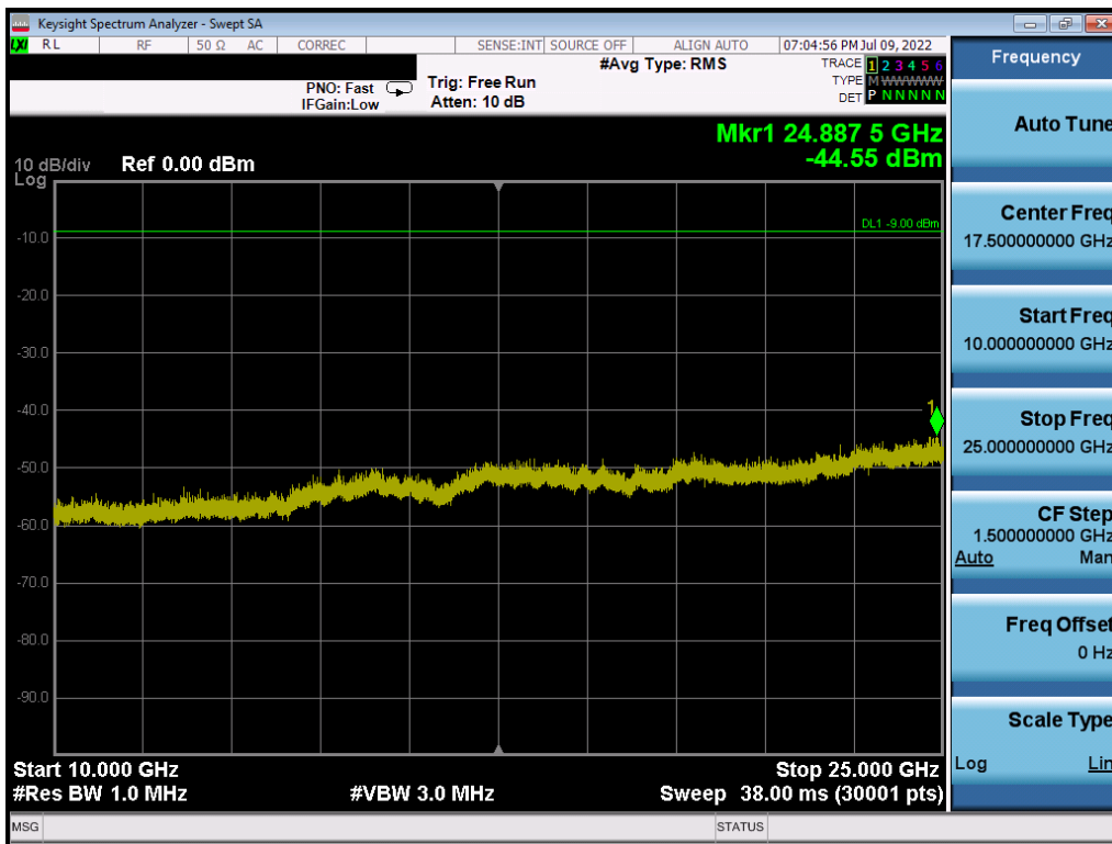
Plot 7-38. Conducted Spurious Plot (Bluetooth (HDRp4), 4 Mbps – Ch. 75)
