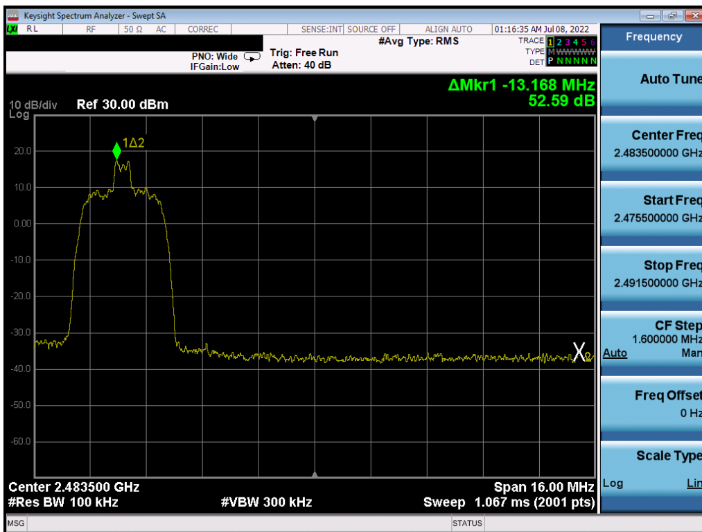
Plot 7-26. Band Edge Plot (Bluetooth (HDR4) – Ch. 75)
