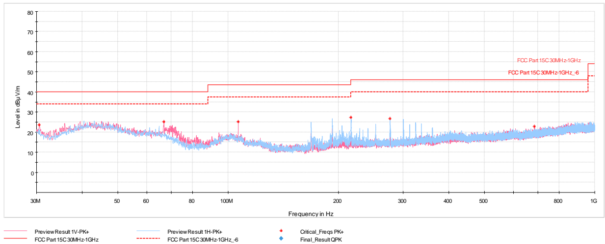
Plot 7-53. Radiated Spurious Emissions Below 1GHz (4Mbps – Ch.75 with AC/DC Adapter)
