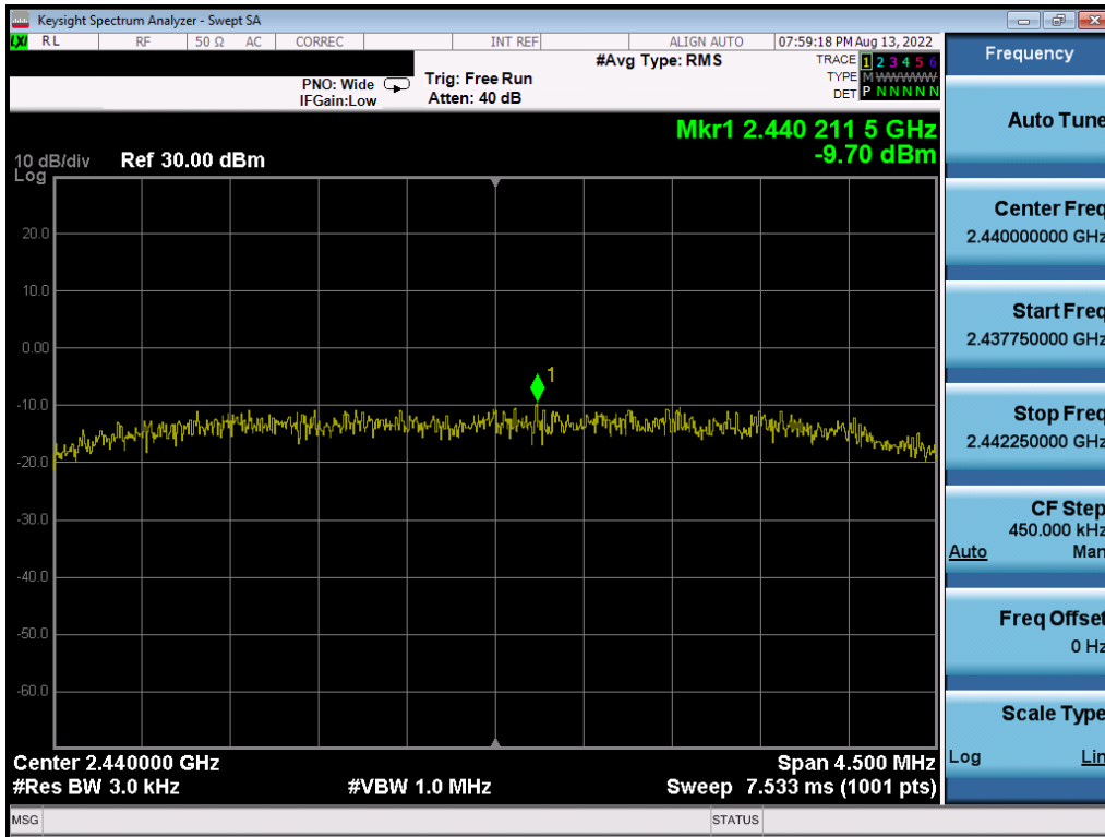
Plot 7-23. Power Spectral Density Plot (Bluetooth (HDRp8), 8Mbps – Ch. 38)
