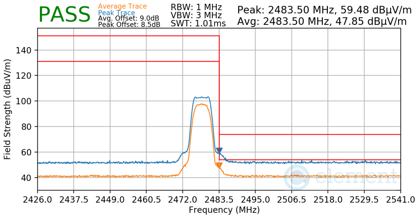
Plot 7-52. Radiated Restricted Upper Band Edge Measurement
