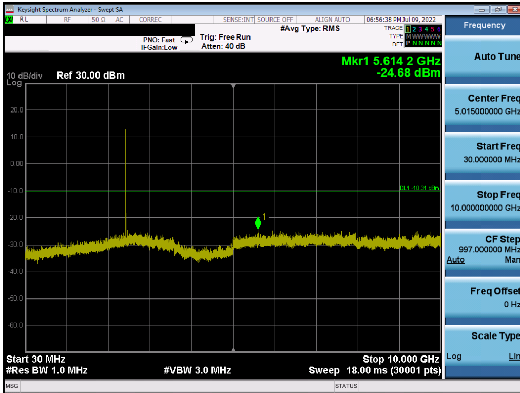
Plot 7-35. Conducted Spurious Plot (Bluetooth (HDRp4), 4 Mbps – Ch. 38)
