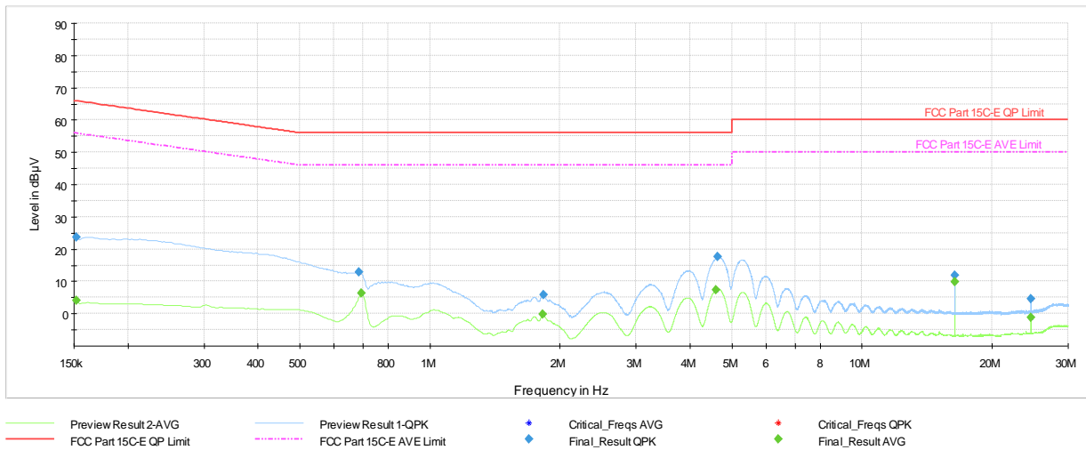
Plot 7-54. AC Line Conducted Plot with Bluetooth HDR (L1, 4Mbps - Ch.75 with AC/DC Adapter)
