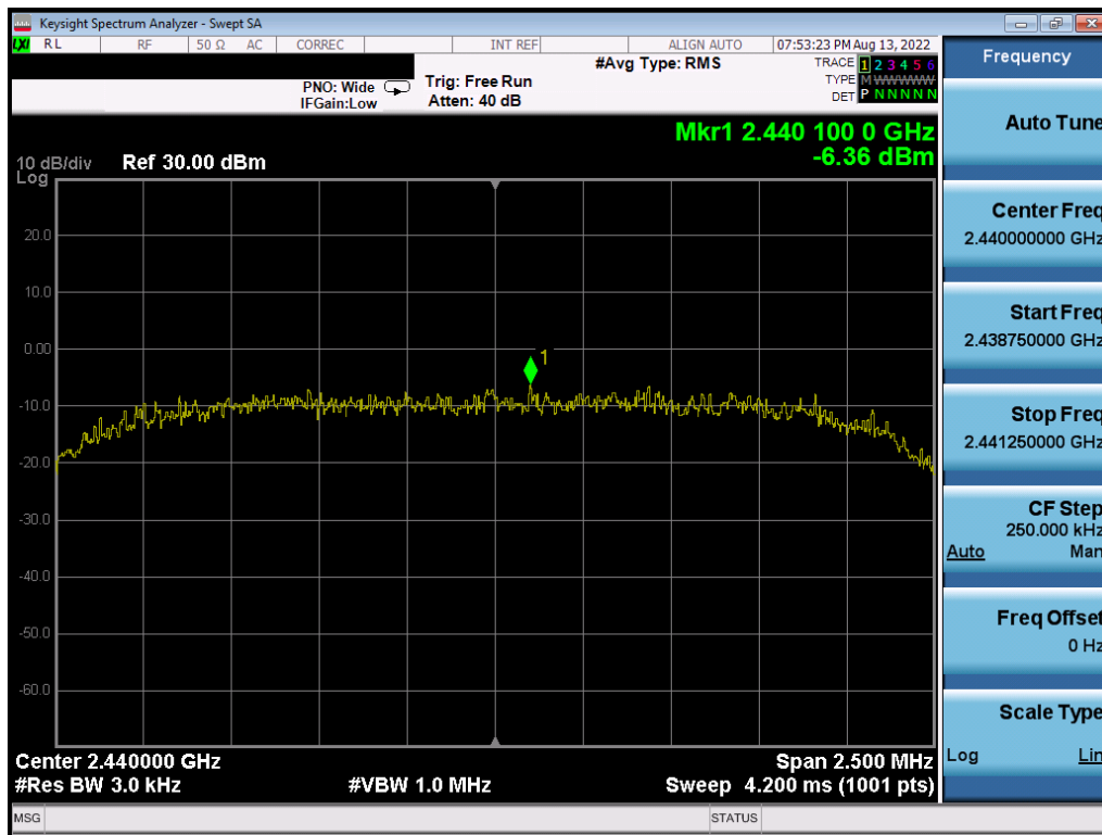
Plot 7-20. Power Spectral Density Plot (Bluetooth (HDRp4), 4Mbps – Ch. 38)
