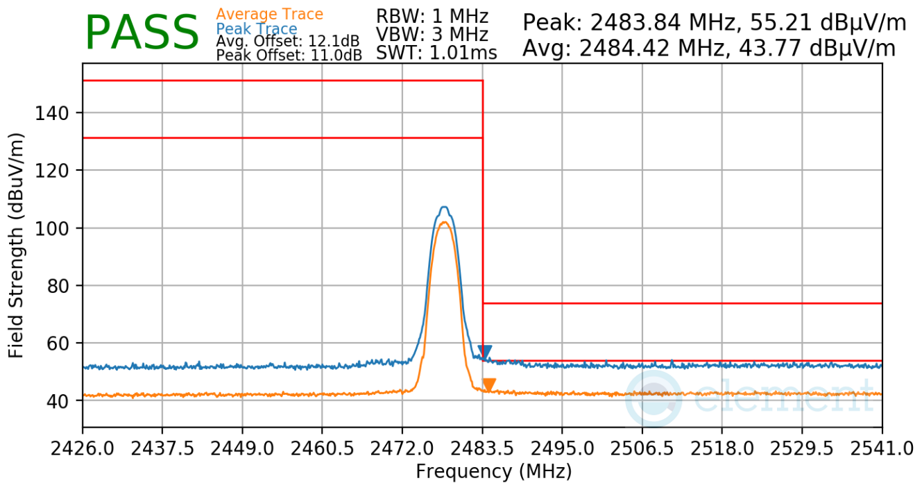
Plot 7-48. Radiated Restricted Upper Band Edge Measurement
