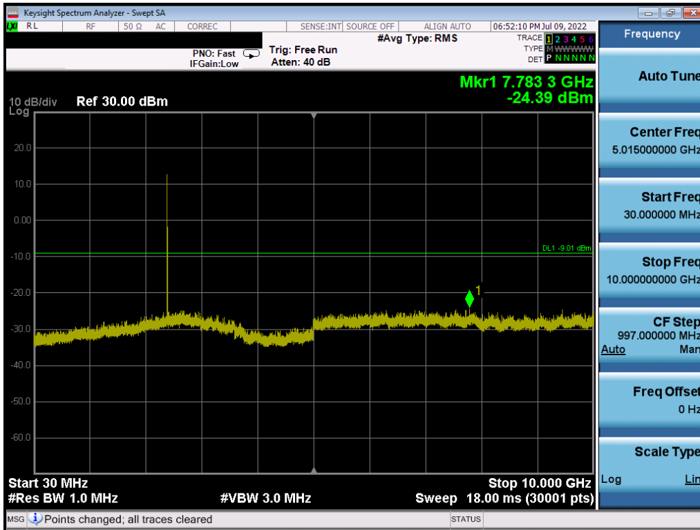
Plot 7-33. Conducted Spurious Plot (Bluetooth (HDRp4), 4 Mbps – Ch. 1)
