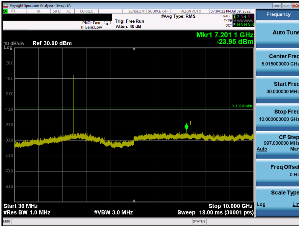
Plot 7-37. Conducted Spurious Plot (Bluetooth (HDRp4), 4 Mbps – Ch. 75)
