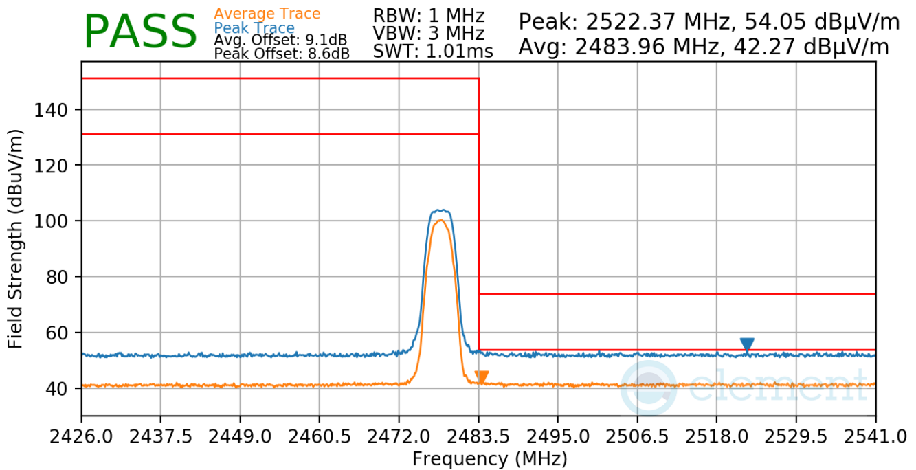
Plot 7-51. Radiated Restricted Upper Band Edge Measurement
