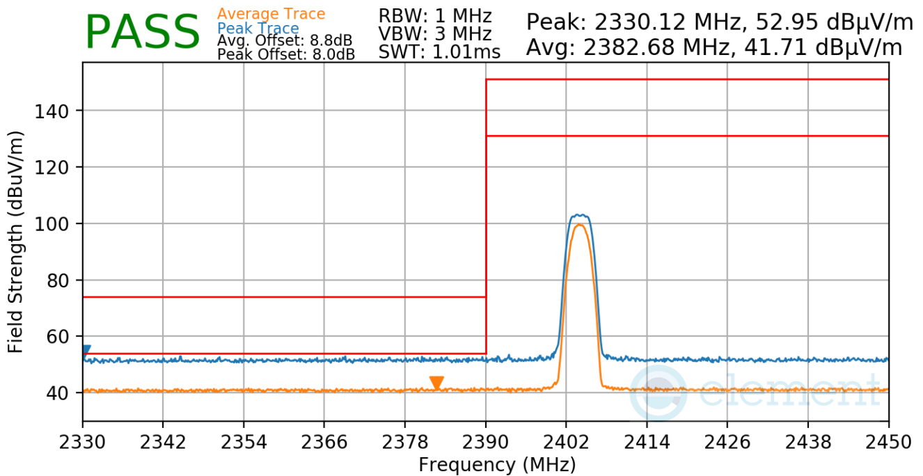
Plot 7-46. Radiated Restricted Lower Band Edge Measurement
