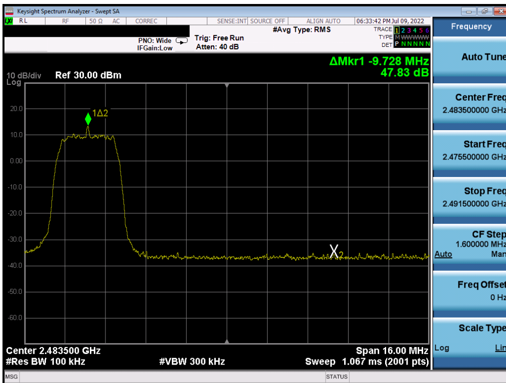
Plot 7-30. Band Edge Plot (Bluetooth (HDRp4) – Ch. 75)
