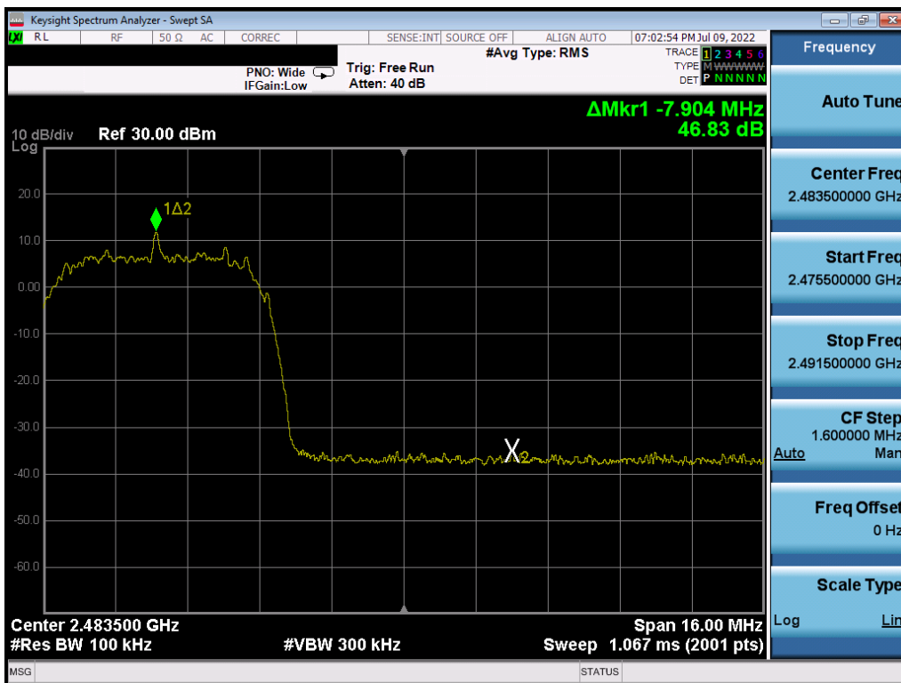
Plot 7-32. Band Edge Plot (Bluetooth (HDRp8) – Ch. 75)
