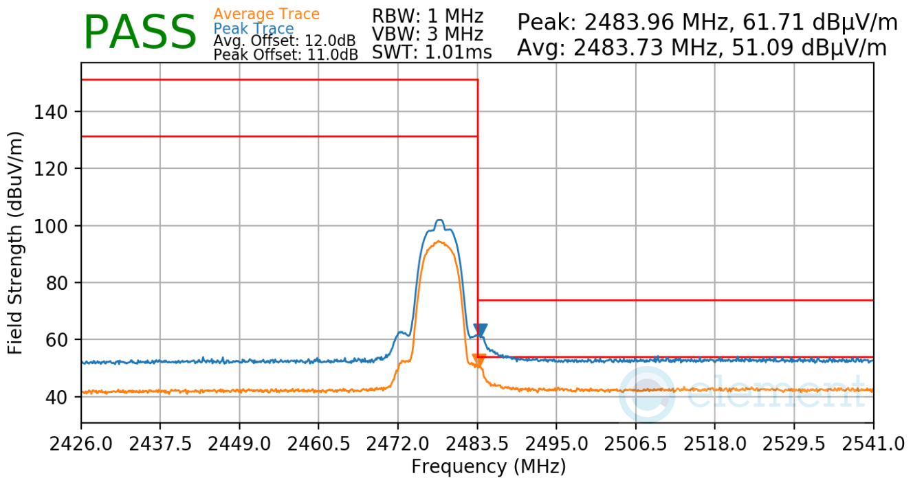
Plot 7-50. Radiated Restricted Upper Band Edge Measurement
