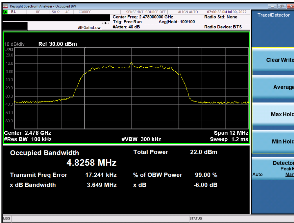
Plot 7-12. 6dB BW & 99% OBW Plot (Bluetooth (HDRp8), 8Mbps – Ch. 75)
