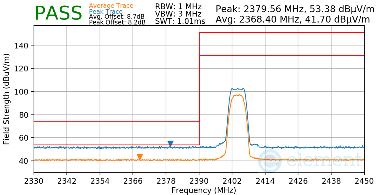
Plot 7-47. Radiated Restricted Lower Band Edge Measurement
