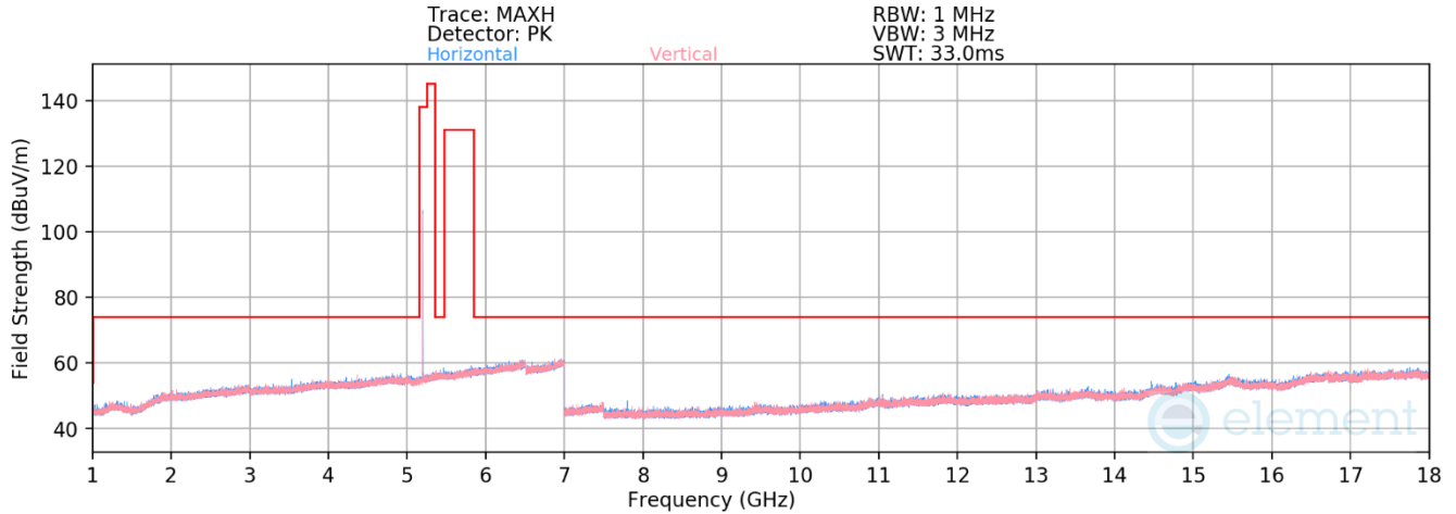
Plot 7-14. Radiated Spurious Emissions Above 1GHz (BDR GFSK – 5201MHz)
