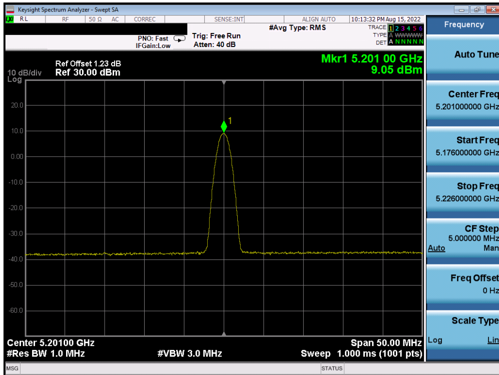
Plot 7-8. PSD (BDR GFSK – 5201MHz)
