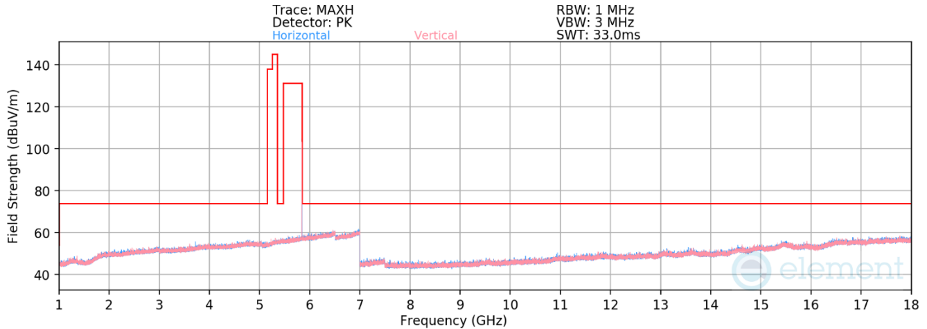
Plot 7-20. Radiated Spurious Emissions Above 1GHz (BDR GFSK – 5844MHz)
