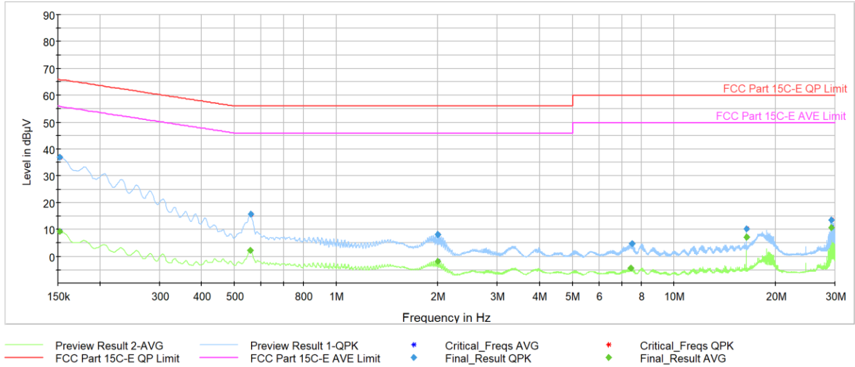
Plot 7-28. AC Line Conducted Plot (BDR GFSK – 5157MHz) (L1) with host PC and lightning cable
