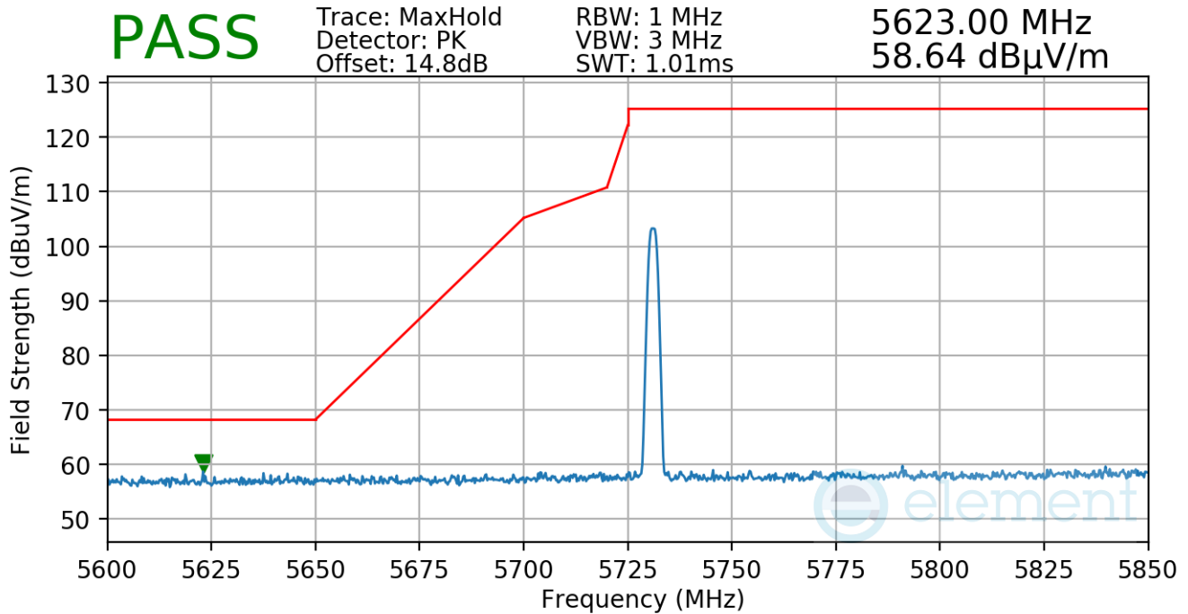
Plot 7-24. Radiated Lower Band Edge Measurement
