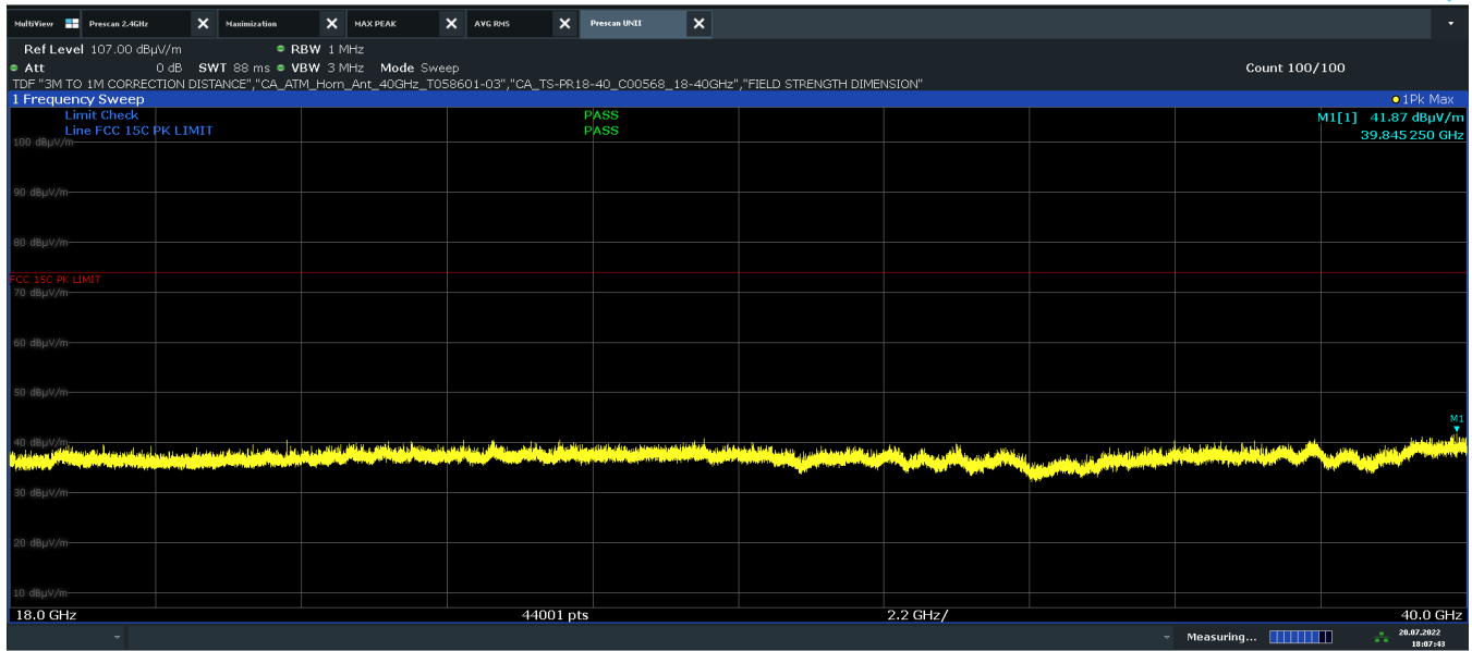
Plot 7-22. Radiated Spurious Emissions Above 18GHz (BDR GFSK – 5844MHz Pol. V)
