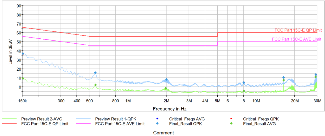
Plot 7-30. AC Line Conducted Plot (BDR GFSK – 5844MHz) (L1) with host PC and lightning cable
