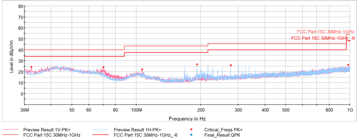
Plot 7-27. Radiated Spurious Emissions Below 1GHz (BDR GFSK – 5844MHz), with AC/DC Adapter and lightning cable
