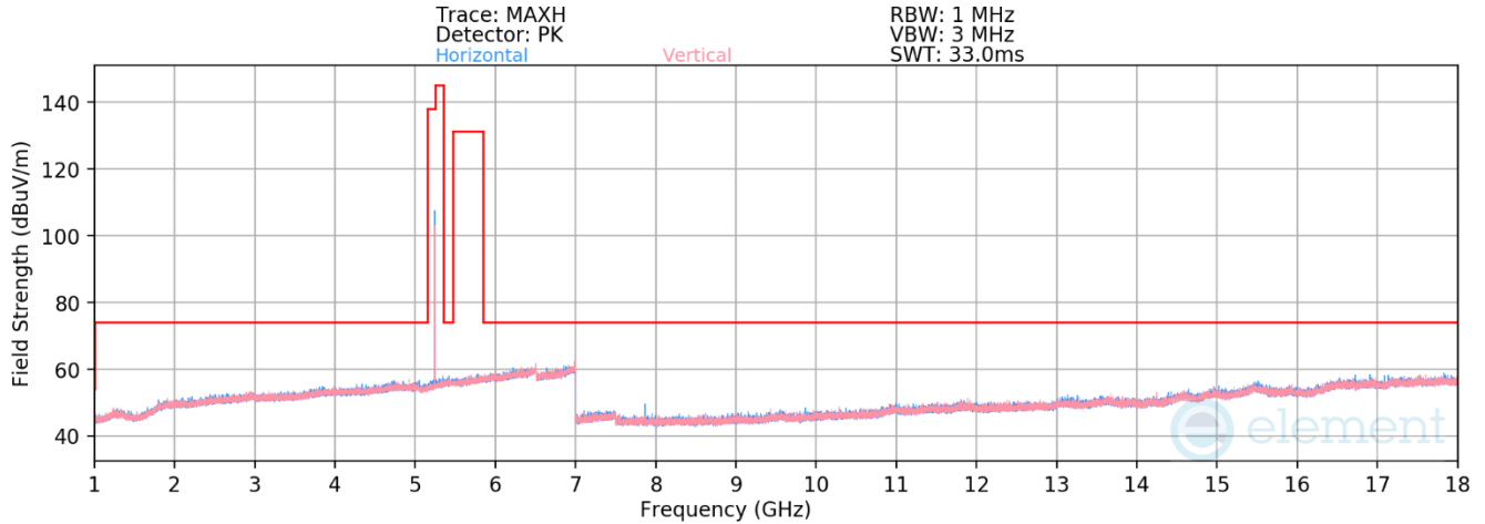
Plot 7-15. Radiated Spurious Emissions Above 1GHz (BDR GFSK – 5245MHz)
