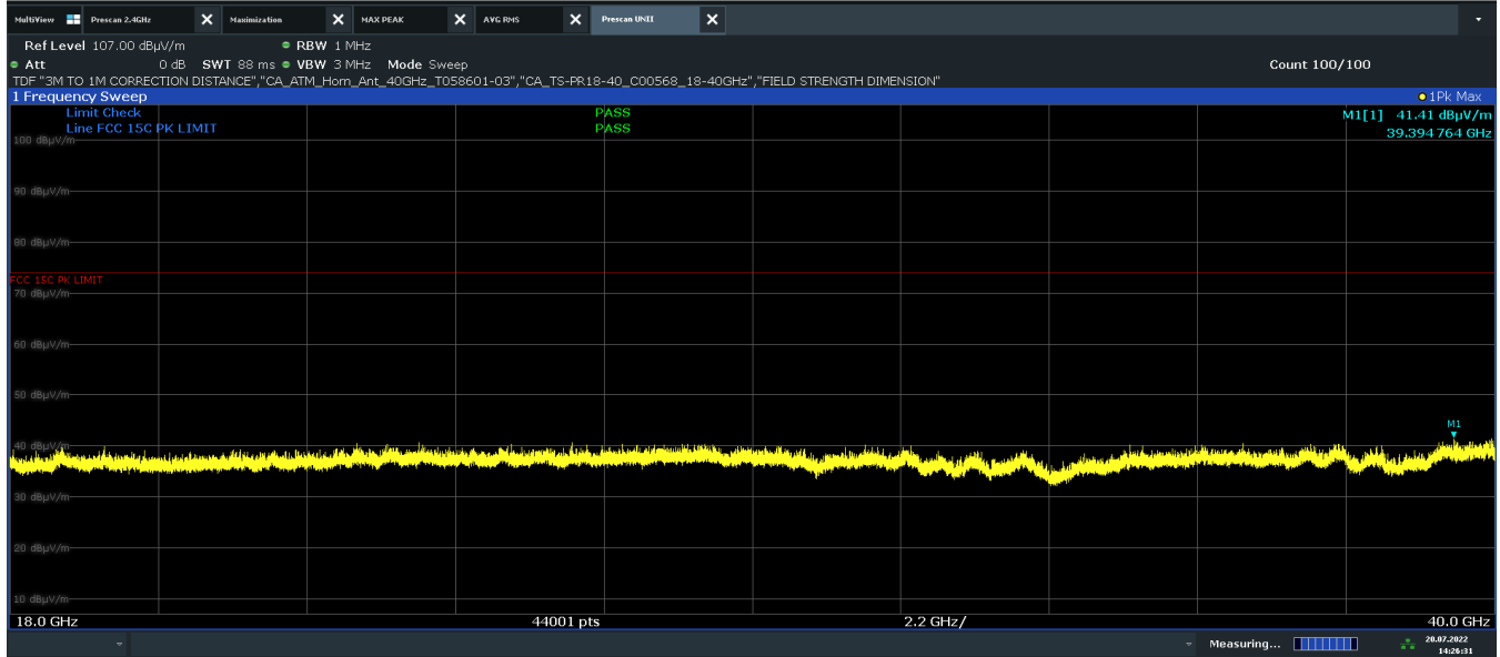
Plot 7-16. Radiated Spurious Emissions Above 18GHz (BDR GFSK – 5157MHz Pol. H)
