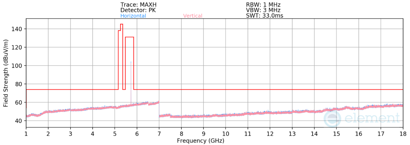
Plot 7-18. Radiated Spurious Emissions Above 1GHz (BDR GFSK – 5731MHz)
