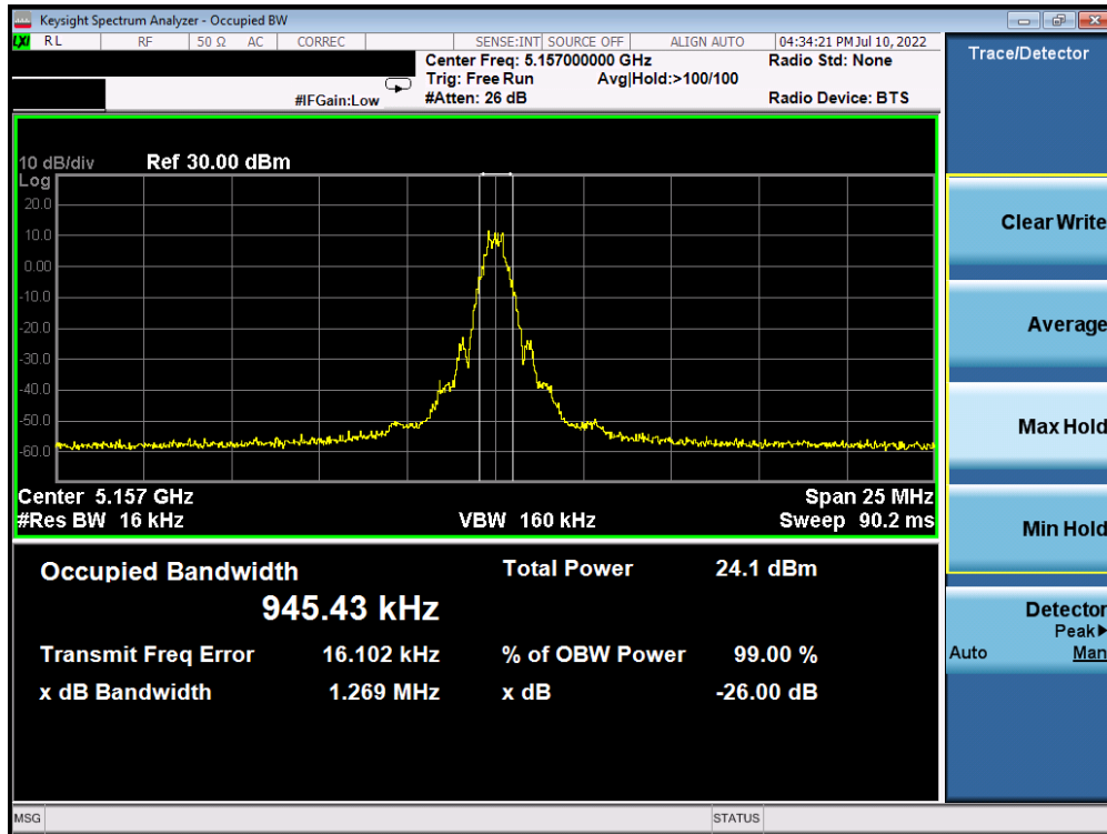
Plot 7-1. 26dB BW & 99% OBW (BDR GFSK – 5157MHz)
