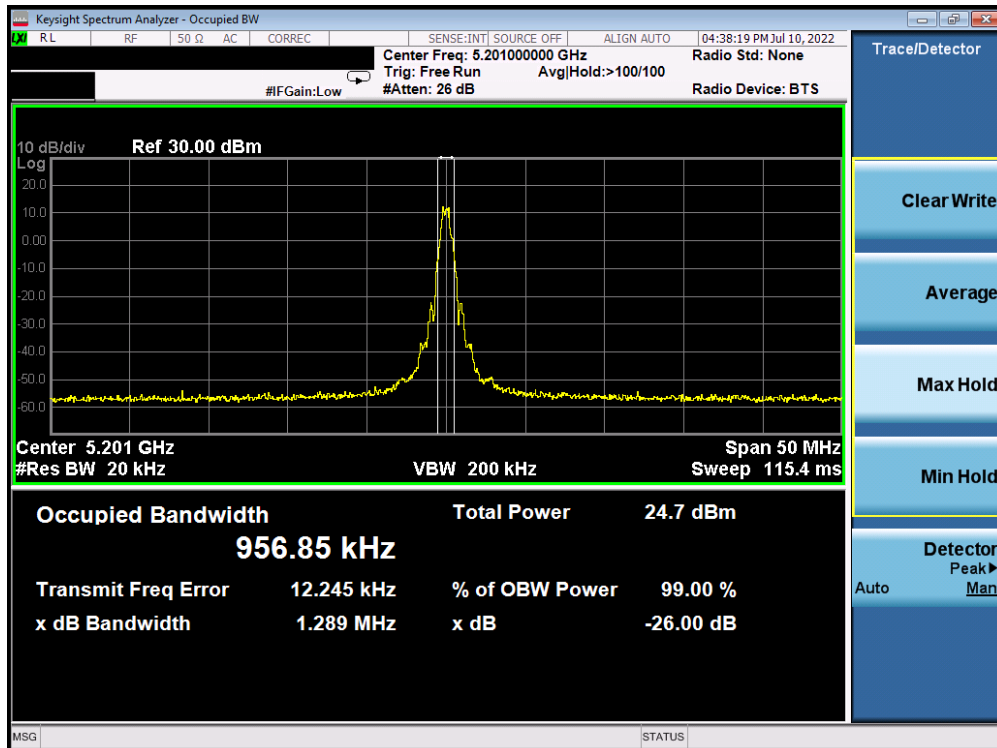
Plot 7-2. 26dB BW & 99% OBW (BDR GFSK – 5201MHz)
