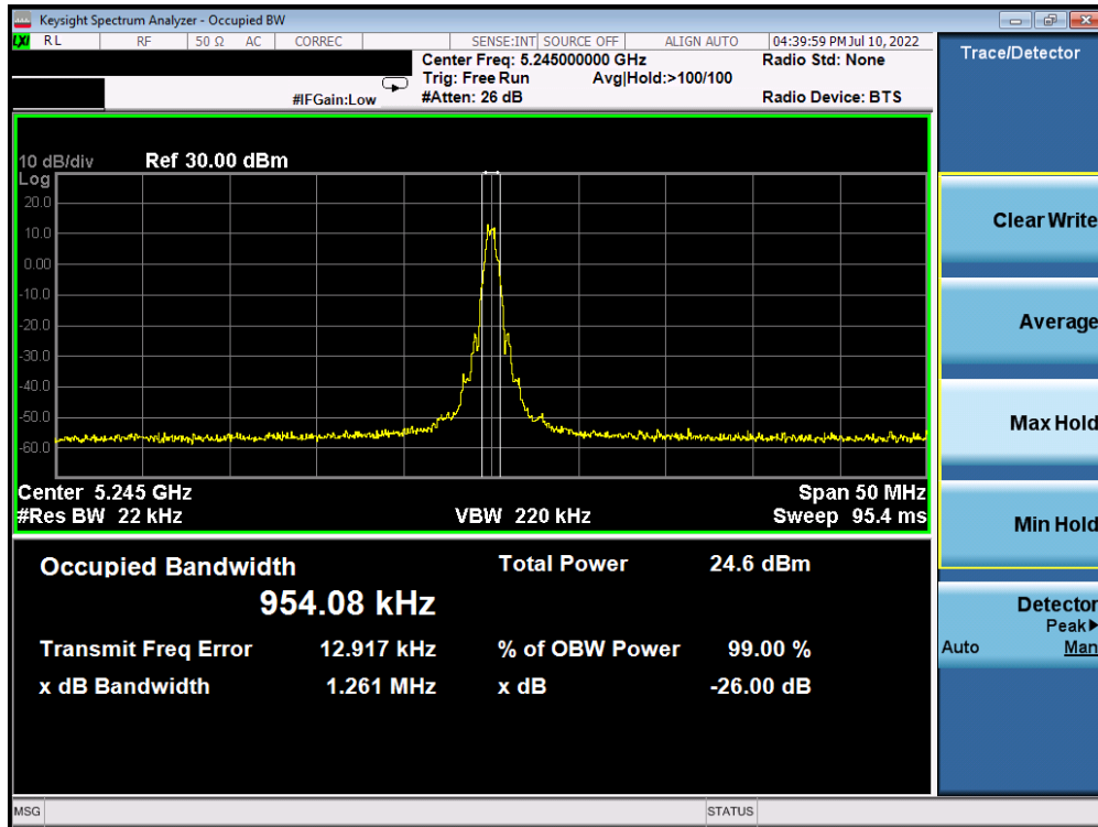
Plot 7-3. 26dB BW & 99% OBW (BDR GFSK – 5245MHz)
