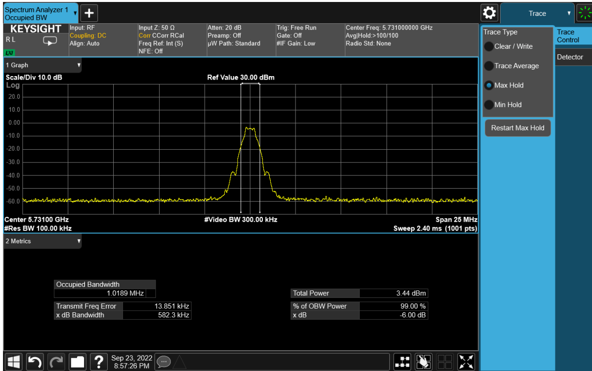
Plot 7-4. 6dB BW & 99% OBW (BDR GFSK – 5731MHz)
