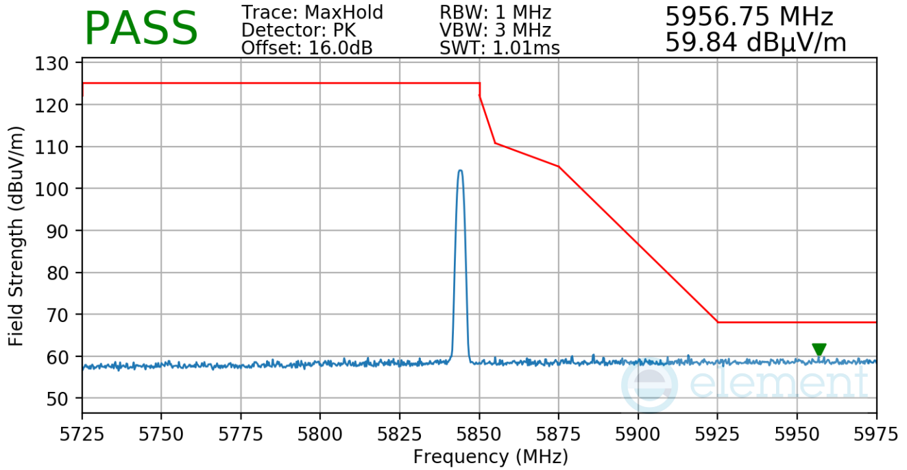
Plot 7-25. Radiated Upper Band Edge Measurement
