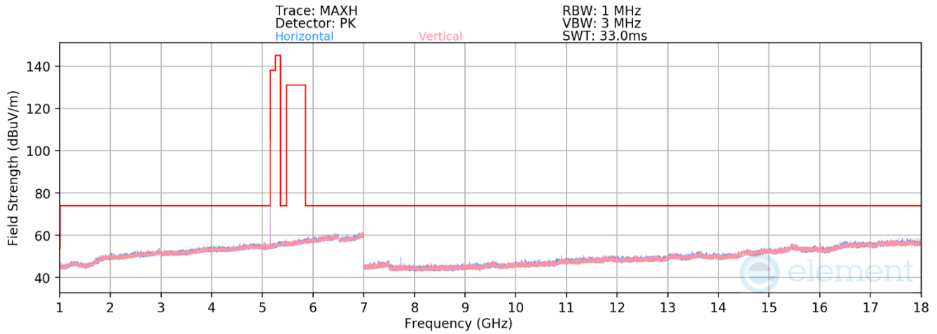
Plot 7-13. Radiated Spurious Emissions Above 1GHz (BDR GFSK – 5157MHz)
