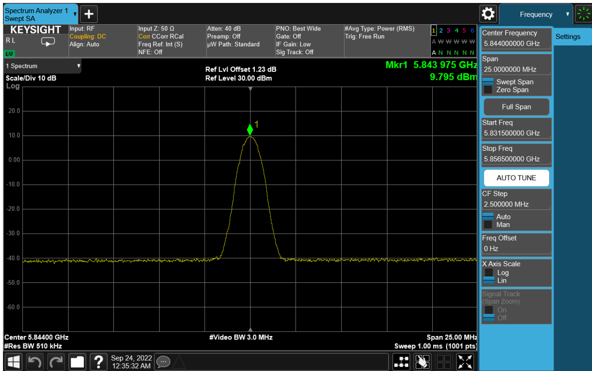
Plot 7-12. PSD (BDR GFSK – 5844MHz)
