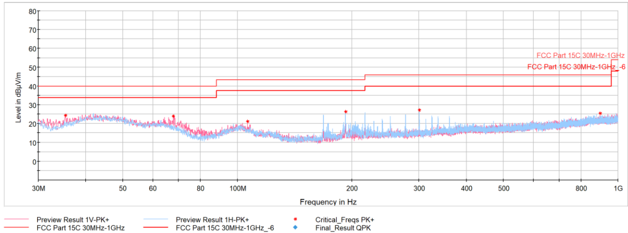
Plot 7-26. Radiated Spurious Emissions Below 1GHz (BDR GFSK – 5157MHz), with AC/DC Adapter and lightning cable
