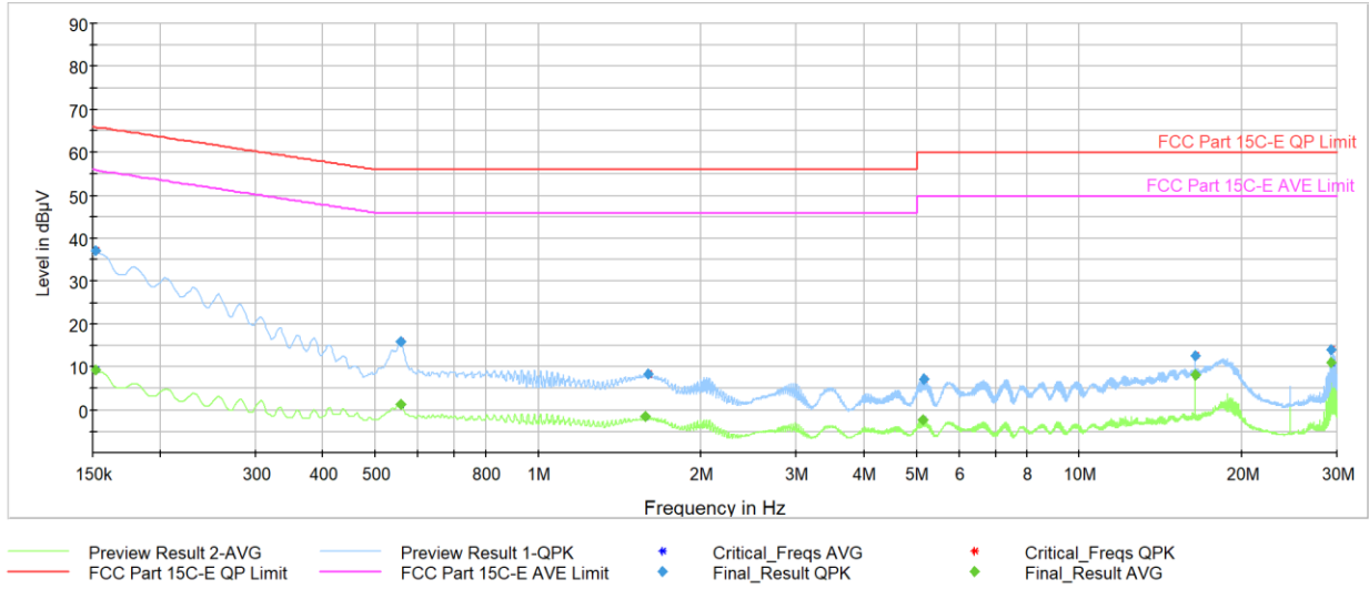
Plot 7-29. AC Line Conducted Plot (BDR GFSK – 5157MHz) (N) with host PC and lightning cable
