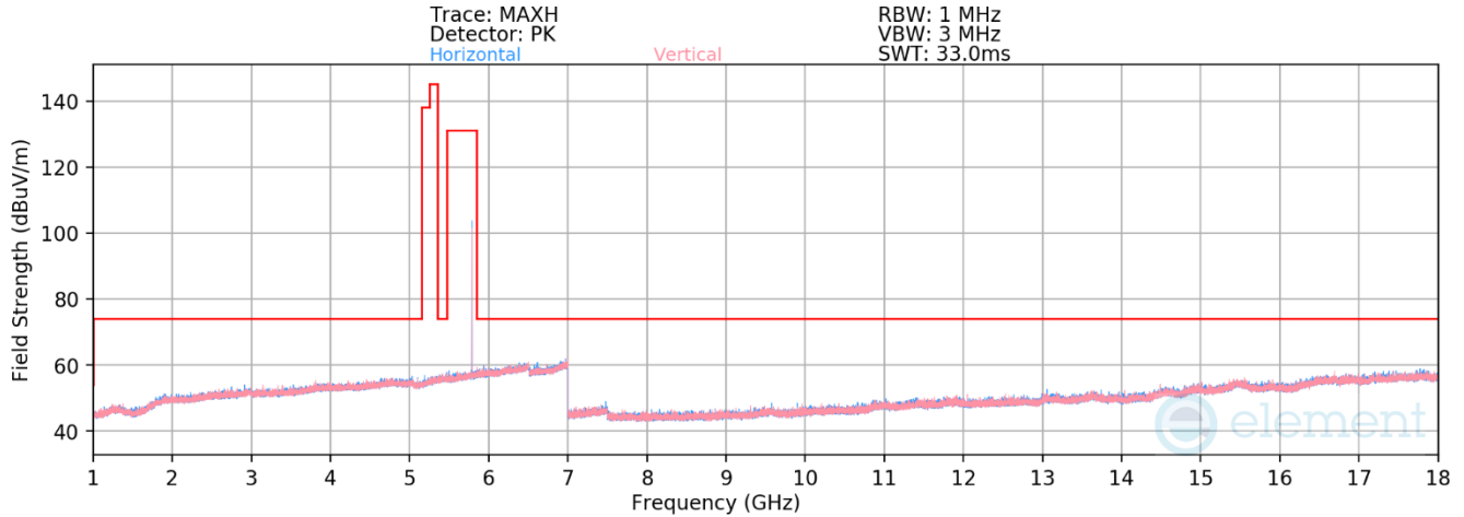
Plot 7-19. Radiated Spurious Emissions Above 1GHz (BDR GFSK – 5788MHz)
