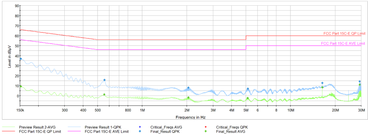
Plot 7-31. AC Line Conducted Plot (BDR GFSK – 5844MHz) (N) with host PC and lightning cable
