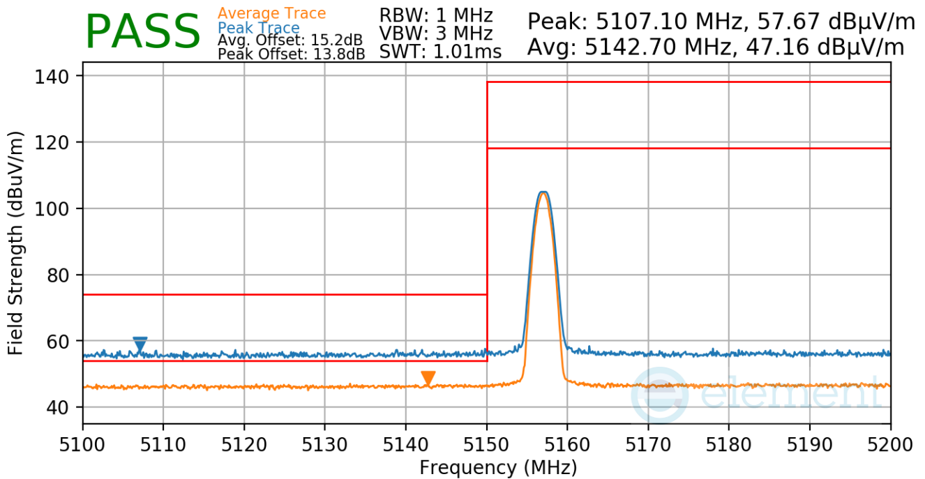
Plot 7-23. Radiated Lower Band Edge Measurement
