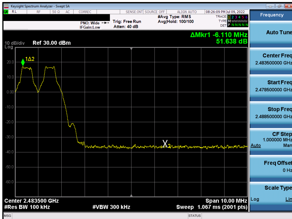
Plot 7-10. Band Edge Plot (Bluetooth with Hopping Enabled, GFSK, 2.4GHz)
