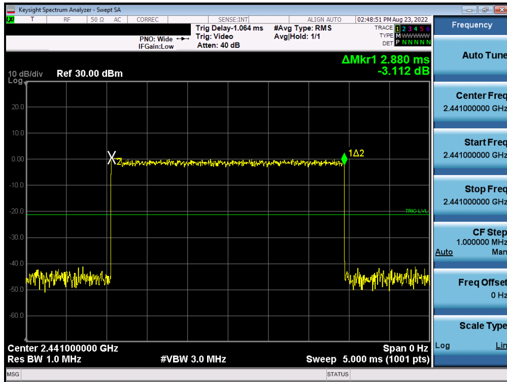
Plot 7-18. Time of Occupancy Plot (Bluetooth, 8DPSK, 2.4GHz)
