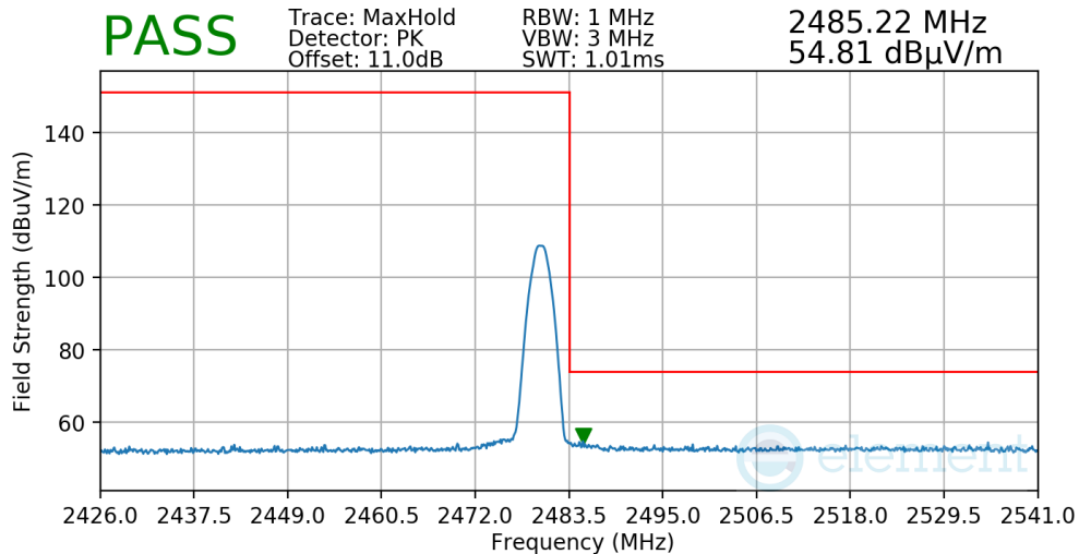
Plot 7-37. Radiated Restricted Upper Band Edge Measurement
