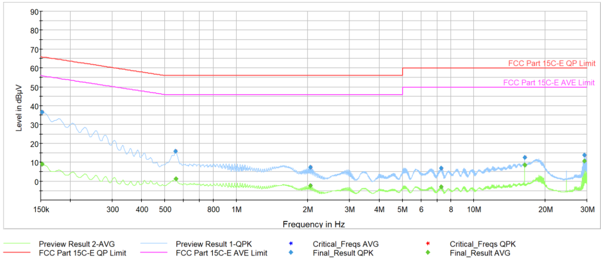
Plot 7-40. AC Line-Conducted Plot (N, GFSK – 2441MHz, with host PC and lightning cable)
