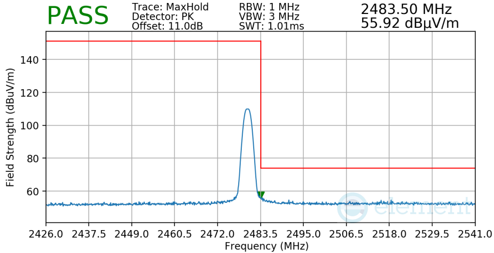
Plot 7-36. Radiated Restricted Upper Band Edge Measurement
