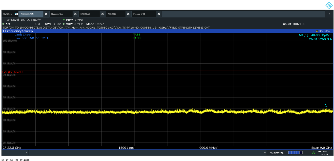
Plot 7-33. Radiated Spurious Emissions above 18GHz (BT GFSK - 2441MHz, Pol. V)
