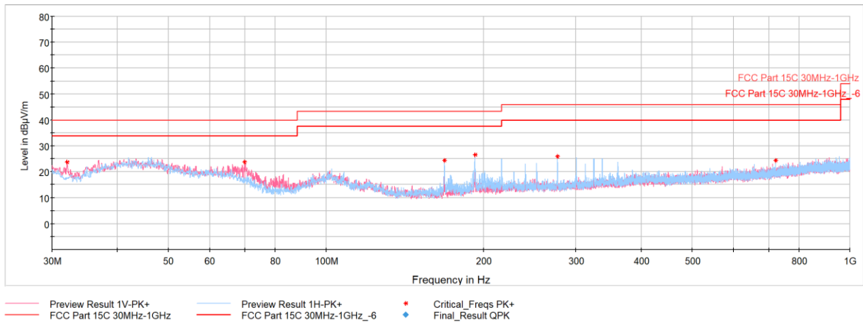
Plot 7-38. Radiated Spurious Emissions Below 1GHz (GFSK – 2441MHz) with AC/DC Adapter and lightning cable
