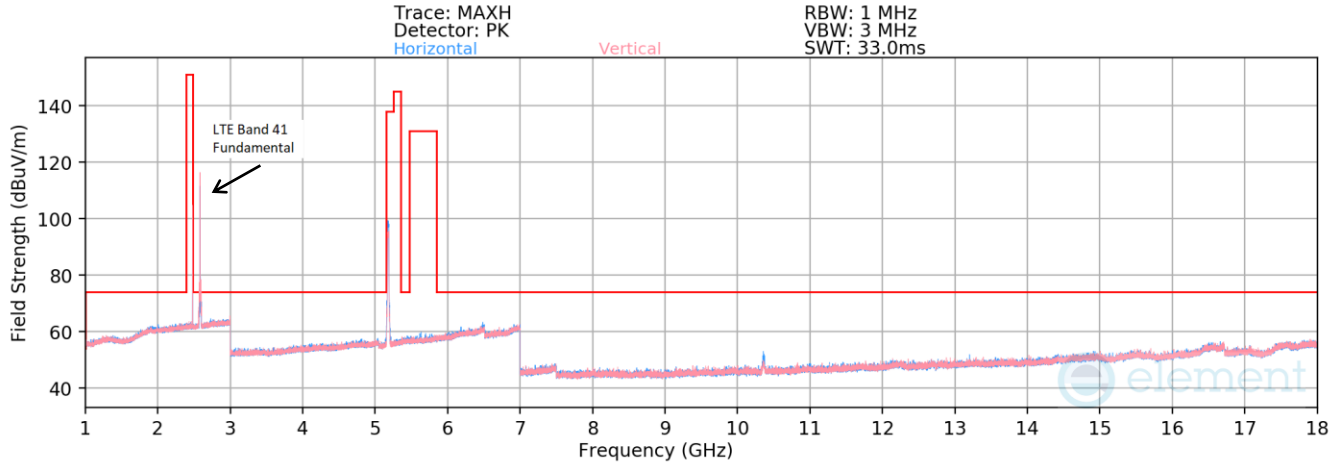
Plot 7-34. Radiated Spurious Emissions 1 - 18GHz – Simultaneous Transmission
