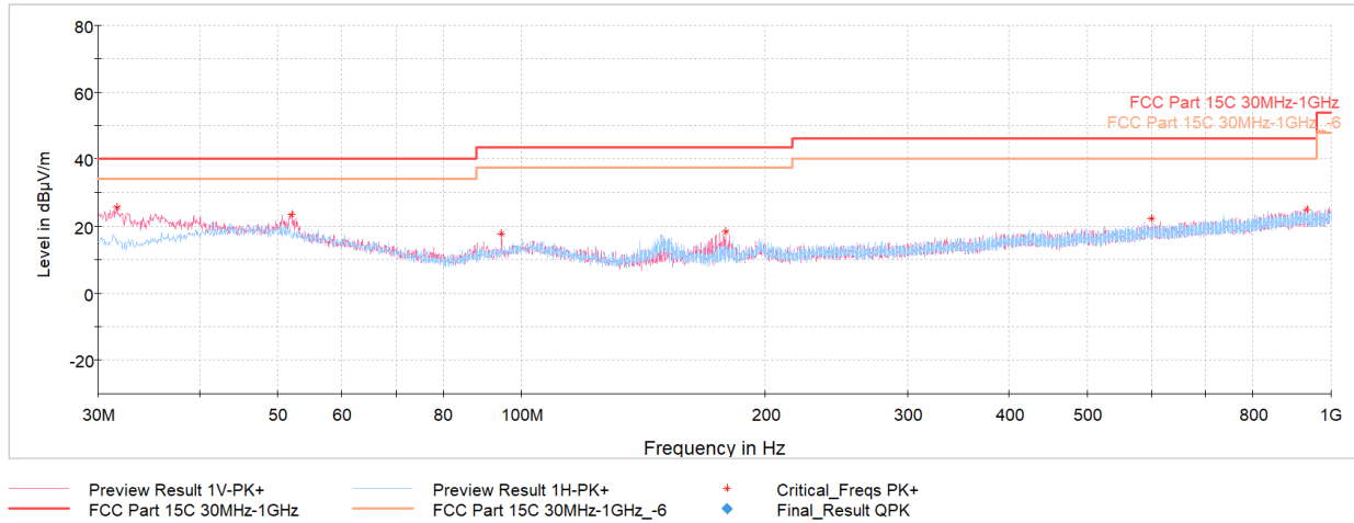
Plot 7-41. Radiated Spurious Emissions Below 1GHz GFSK ePA – Ch.0, with AC/DC Adapter + Magnetic Charger)
