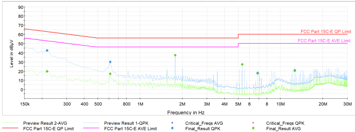
Plot 7-43. AC Line-Conducted Test Plot (L1, GFSK ePA – Ch.0, with AC/DC Adapter + Laptop Charger)
