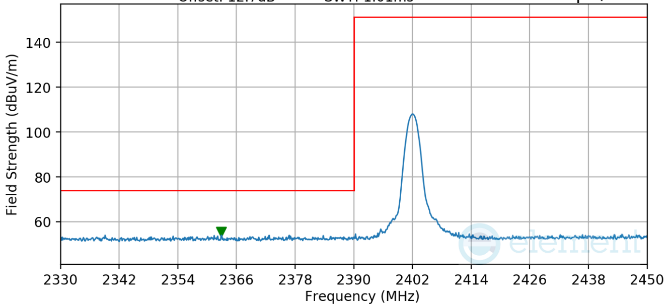
Plot 7-38. Radiated Restricted Lower Band Edge Measurement
