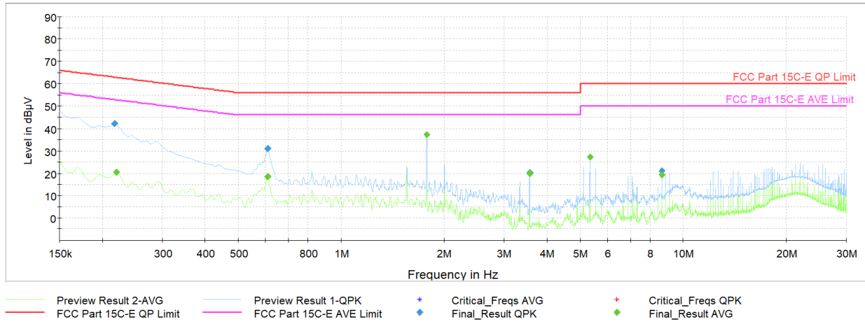
Plot 7-44. AC Line-Conducted Test Plot (N, GFSK ePA – Ch.0, with AC/DC Adapter + Laptop Charger)
