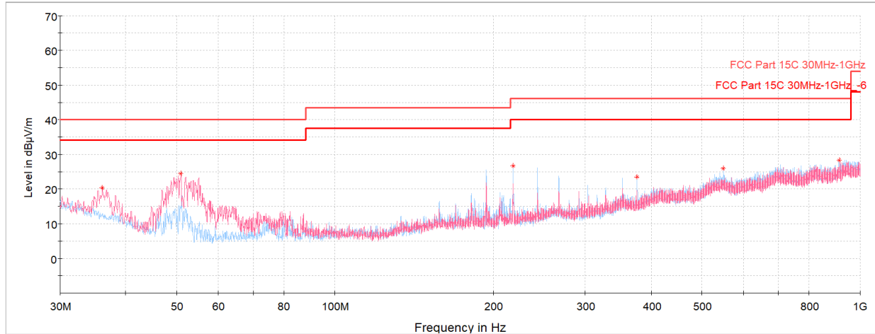
Plot 7-42. Radiated Spurious Emissions below 1GHz – Simultaneous Transmission
