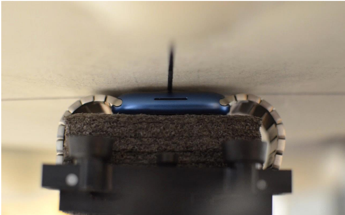
SAR Test Setup Photo 11 – Aluminum with Metal Links Wristband, Extremity, Back Side at 0.0 cm
