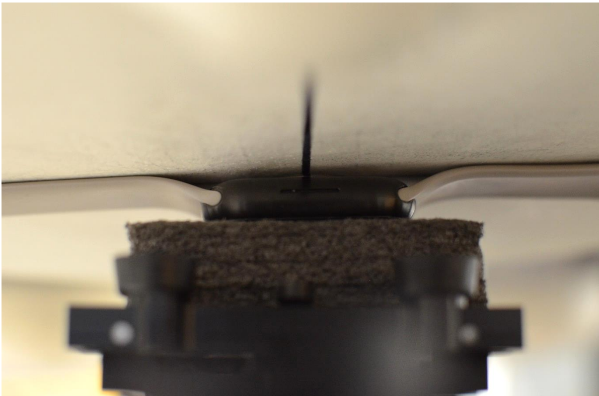
SAR Test Setup Photo 16 – Titanium with Sport Wristband, Extremity, Back Side at 0.0 cm
