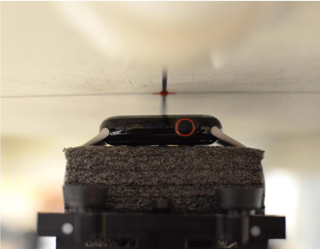
SAR Test Setup Photo 4 – Stainless Steel with Sport Wristband, Head, Front Side at 1.0 cm
