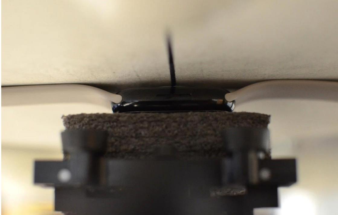
SAR Test Setup Photo 13 – Stainless Steel with Sport Wristband, Extremity, Back Side at 0.0 cm
