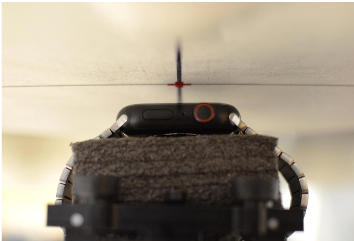
SAR Test Setup Photo 8 – Titanium with Metal Links Wristband, Head, Front Side at 1.0 cm
