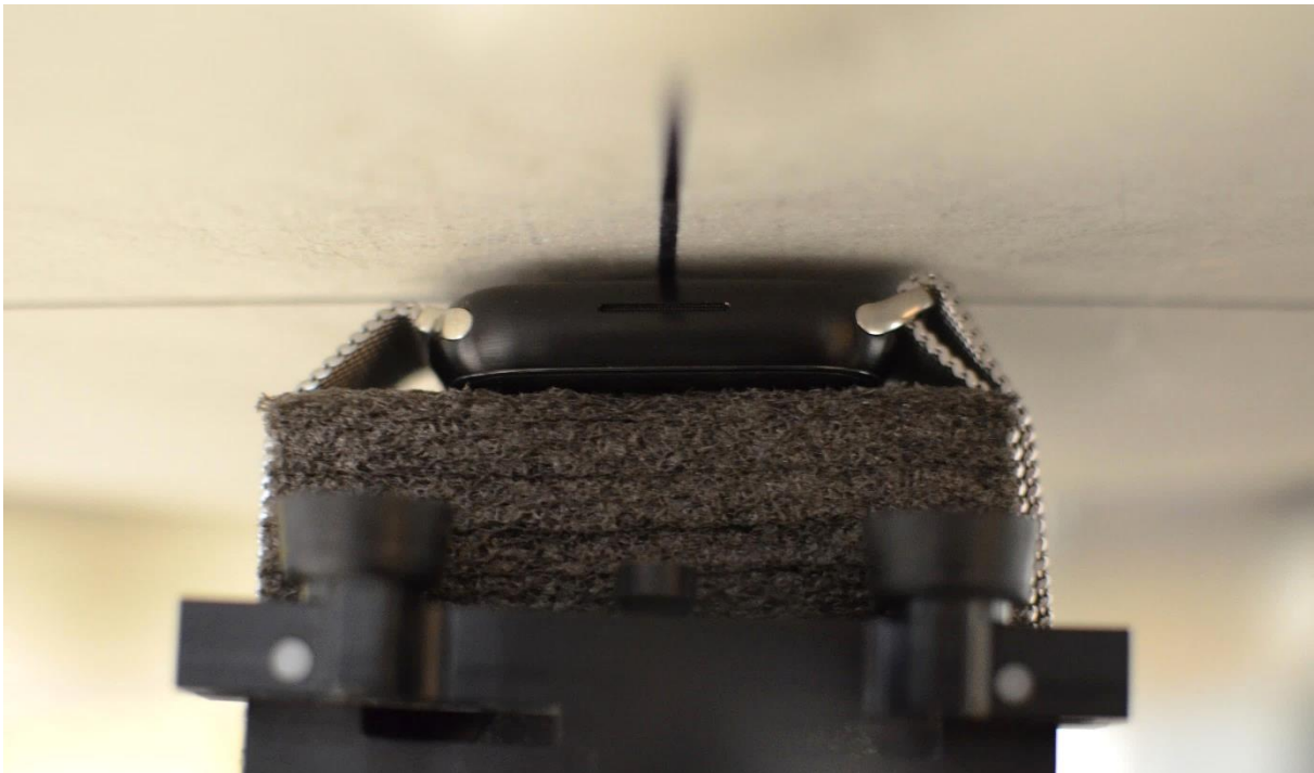
SAR Test Setup Photo 18 – Titanium with Metal Loop Wristband, Extremity, Back Side at 0.0 cm
