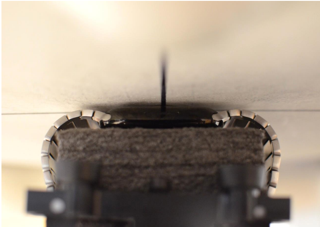
SAR Test Setup Photo 14 – Stainless Steel with Metal Links Wristband, Extremity, Back Side at 0.0 cm
