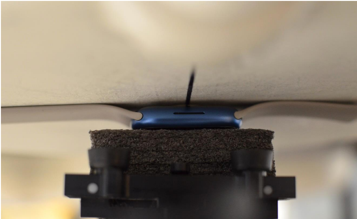
SAR Test Setup Photo 10 – Aluminum with Sport Wristband, Extremity, Back Side at 0.0 cm
