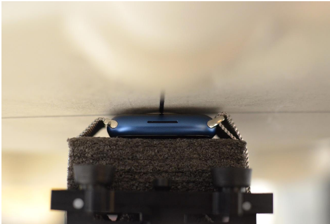
SAR Test Setup Photo 12 – Aluminum with Metal Loop Wristband, Extremity, Back Side at 0.0 cm
