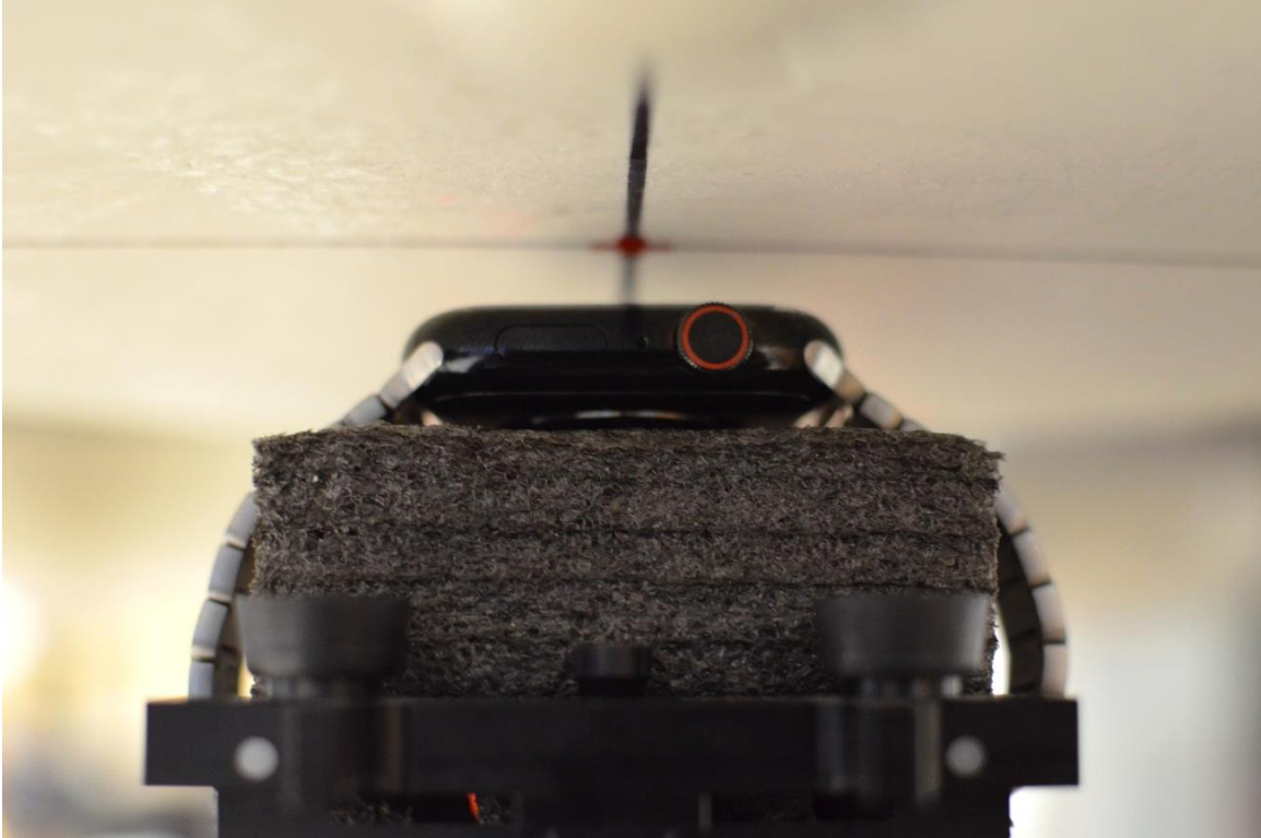
SAR Test Setup Photo 5 – Stainless Steel with Metal Links Wristband, Head, Front Side at 1.0 cm
