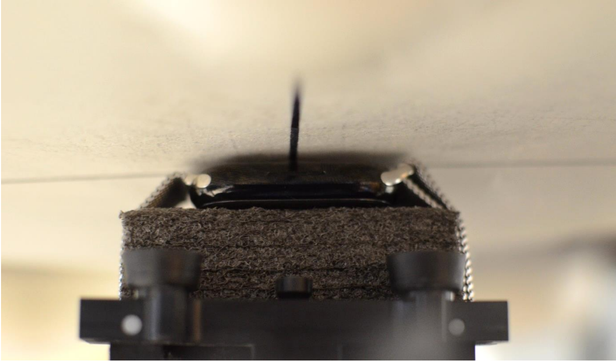
SAR Test Setup Photo 15 – Stainless Steel with Metal Loop Wristband, Extremity, Back Side at 0.0 cm
