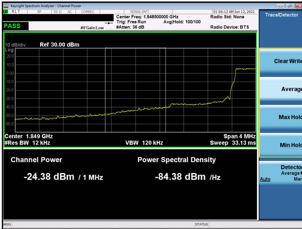
Plot 7-57. Extended Lower Band Edge Plot (LTE Band 25 – 1.4MHz QPSK – Full RB Configuration)
