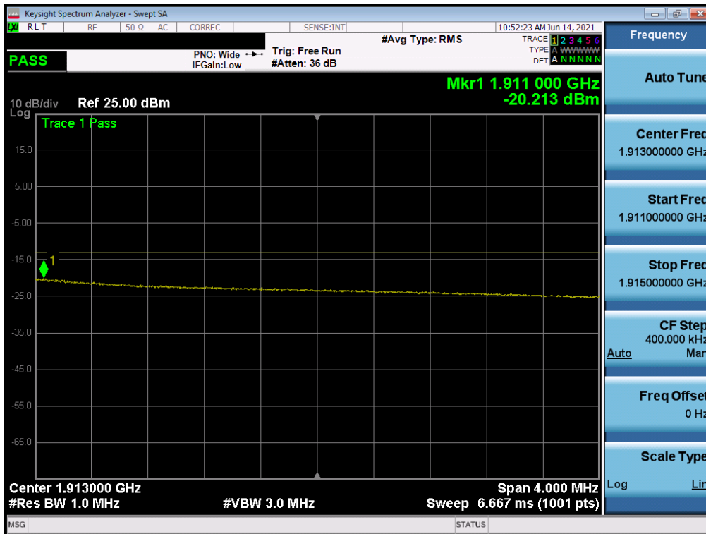
Plot 7-55. Extended Upper Band Edge Plot (LTE Band 2 – 20MHz QPSK – Full RB Configuration)
