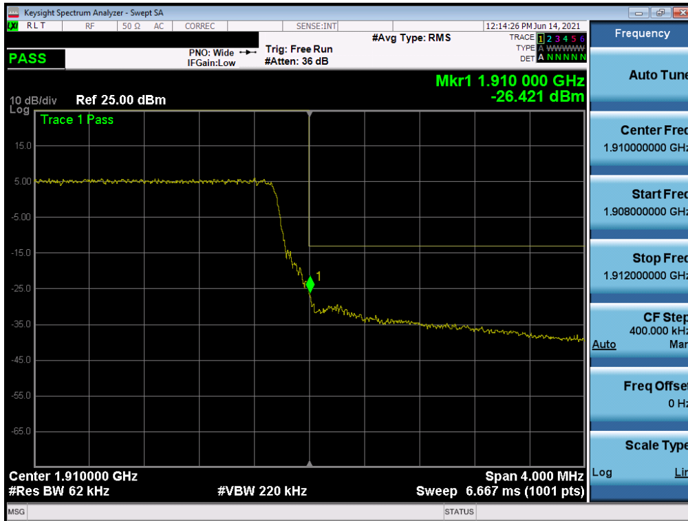
Plot 7-42. Upper Band Edge Plot (LTE Band 2 – 5MHz QPSK – Full RB Configuration)
