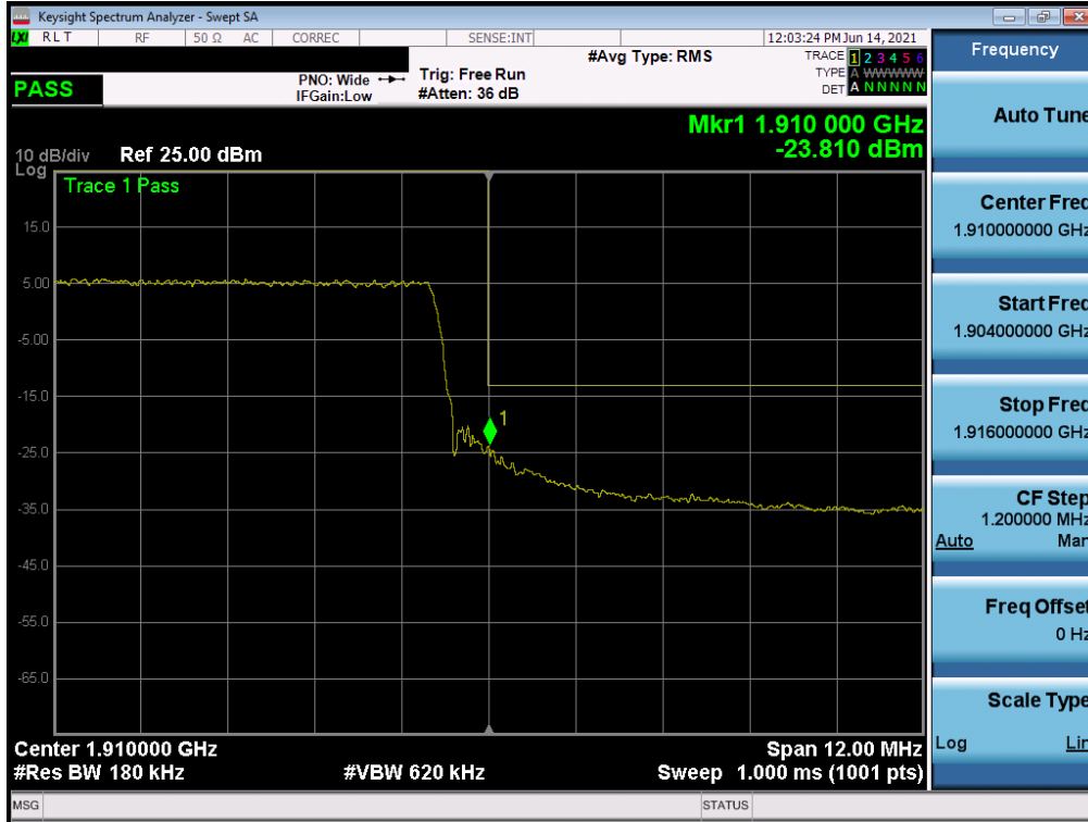
Plot 7-50. Upper Band Edge Plot (LTE Band 2 – 15MHz QPSK – Full RB Configuration)
