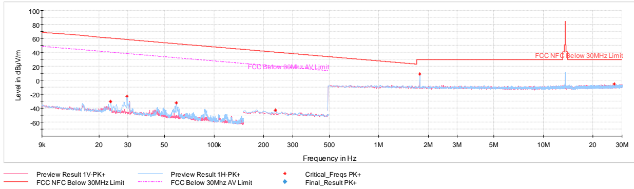
Plot 7-9. Radiated Spurious Emissions 9kHz – 30MHz (Reader 10% ASK 1 out of 256, with AC/DC Adapter and Magnetic Charger)
