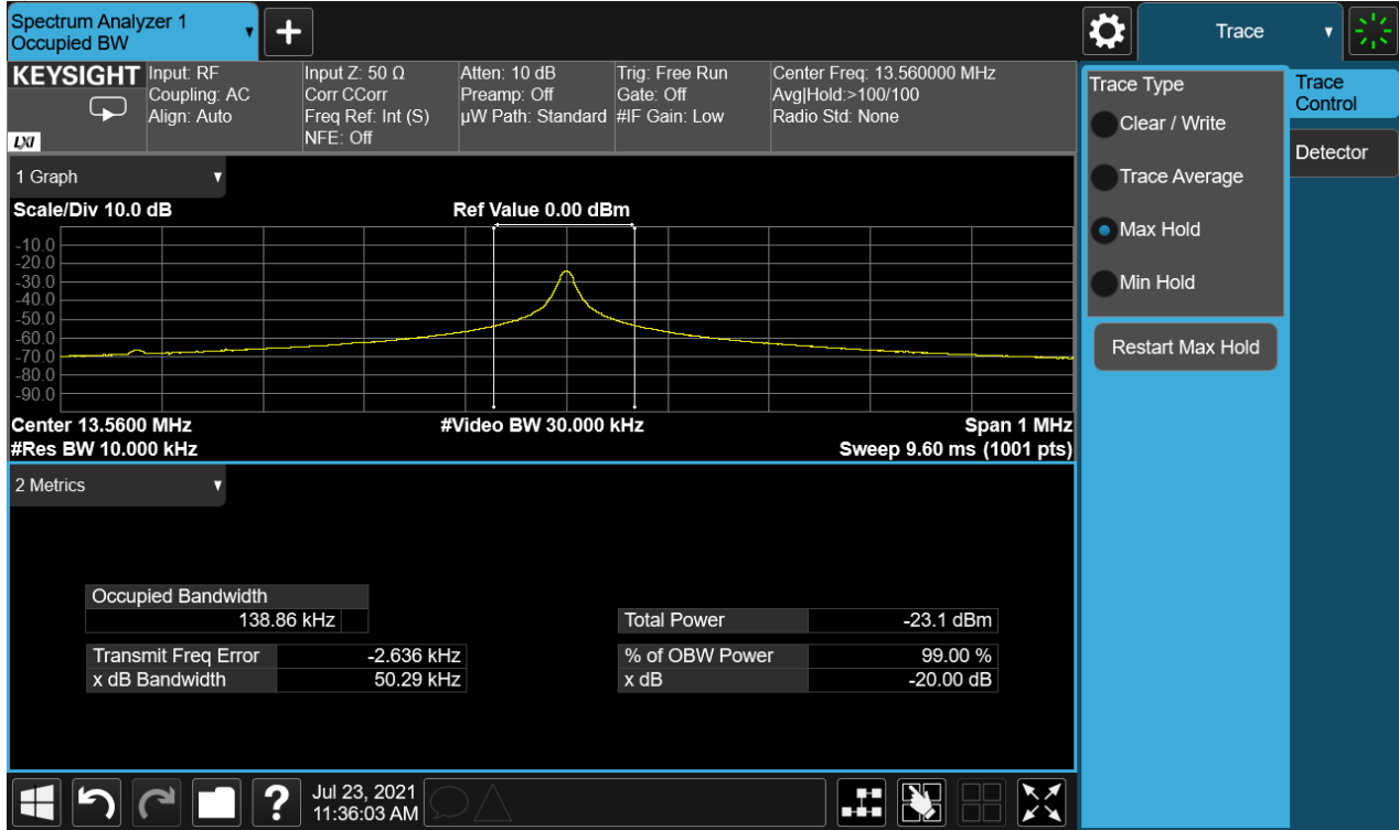
Plot 7-2. 20dB and 99% Bandwidth Plot (CE B 848kbps)
