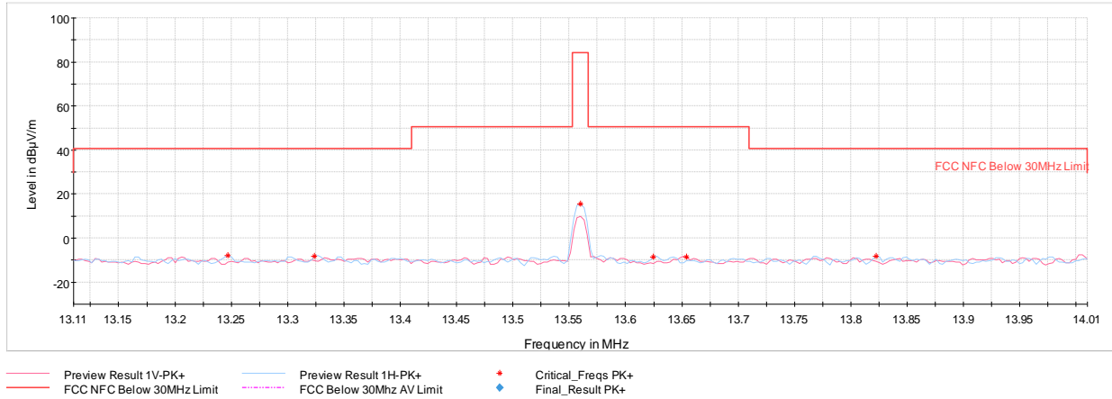
Plot 7-6. In Band Radiated Spurious Emissions (CE A 848kbps, with AC/DC Adapter and Magnetic Charger)
