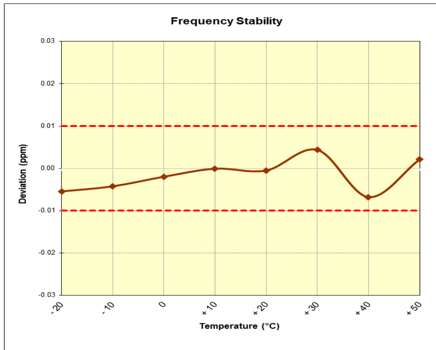
Figure 7-4. Frequency Stability Plot (Reader 10% ASK 1 out of 256)
