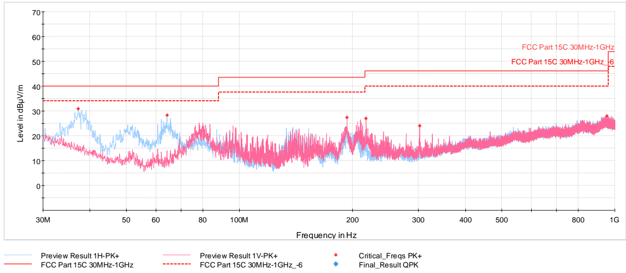
Plot 7-11. Radiated Spurious Emissions 30MHz – 1GHz (Reader 10% ASK 1 out of 256, with AC/DC Adapter and Magnetic Charger)
