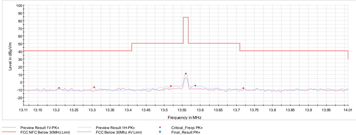
Plot 7-7. In Band Radiated Spurious Emissions (Reader 10% ASK 1 out of 256, AC/DC Adapter and Magnetic Charger)
