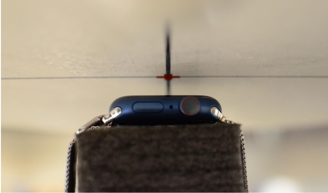
SAR Test Setup Photo 3: Aluminum with Metal Loop Wristband, Head, Front side at 1.0 cm
