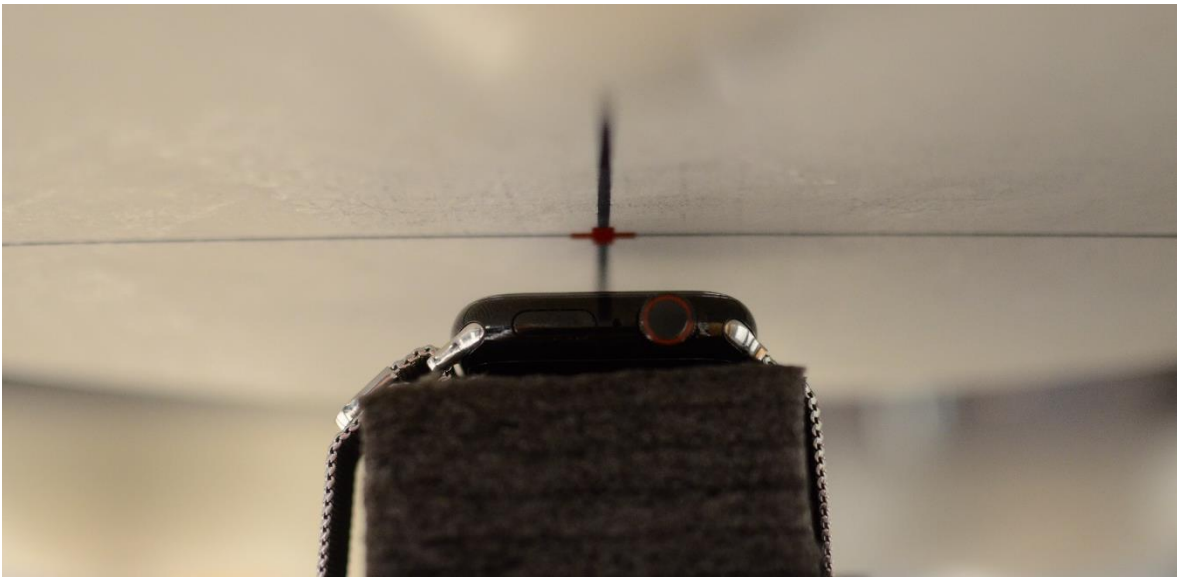
SAR Test Setup Photo 6: Stainless Steel with Metal Loop Wristband, Head, Front side at 1.0 cm
