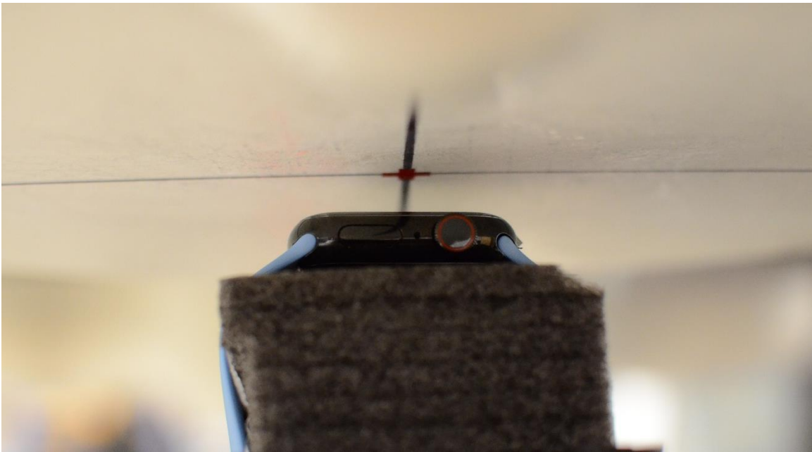
SAR Test Setup Photo 4: Stainless Steel with Sport Wristband, Head, Front side at 1.0 cm
