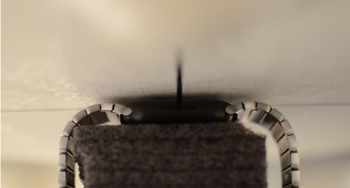
SAR Test Setup Photo 17: Titanium with Metal Links Wristband, Extremity, Back side at 0.0 cm
