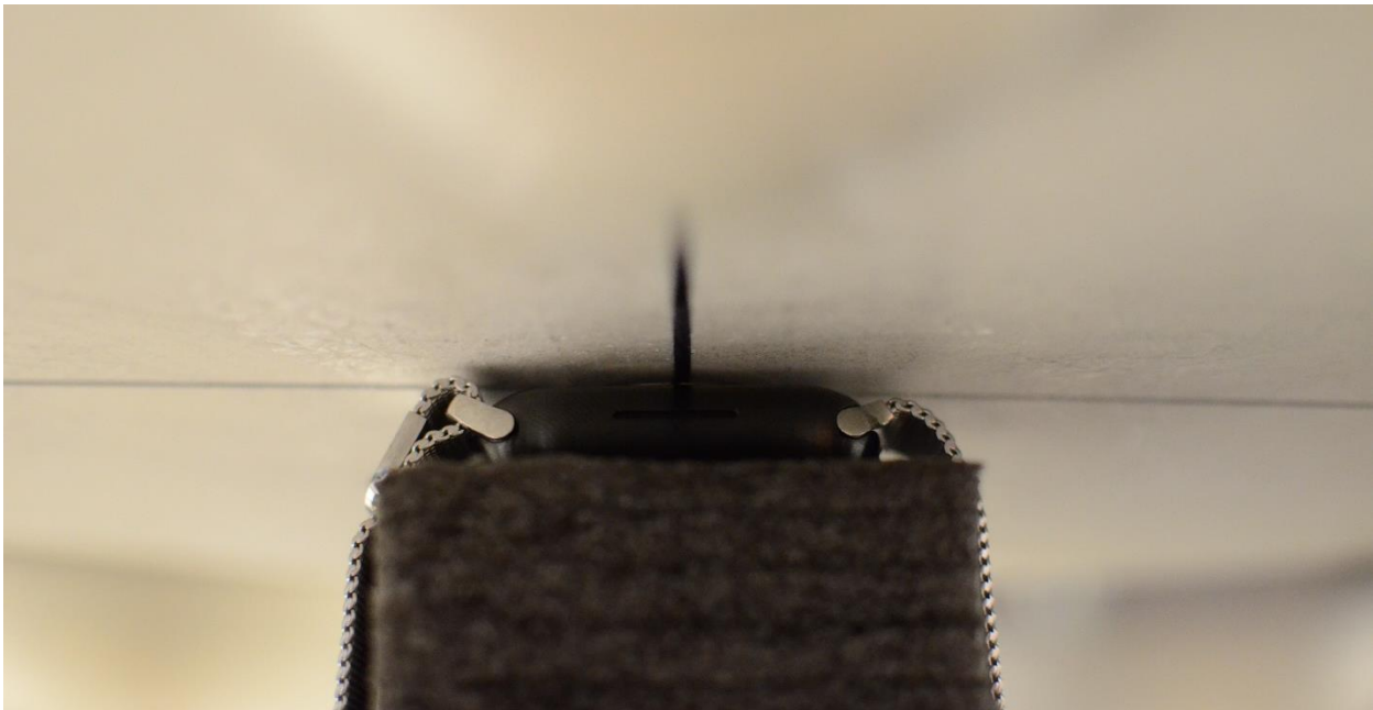
SAR Test Setup Photo 18: Titanium with Metal Loop Wristband, Extremity, Back side at 0.0 cm
