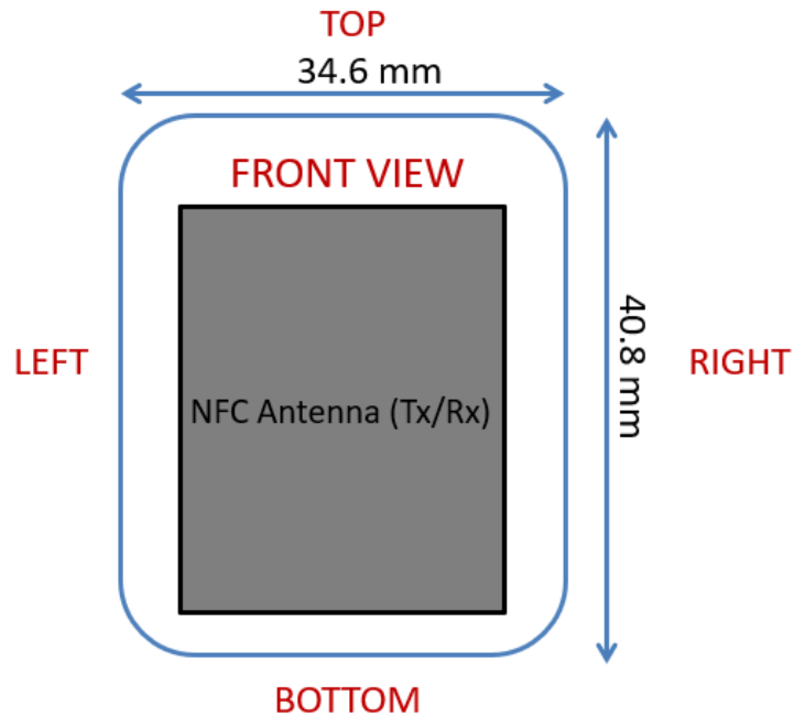
Figure E-2 NFC Antenna Location
