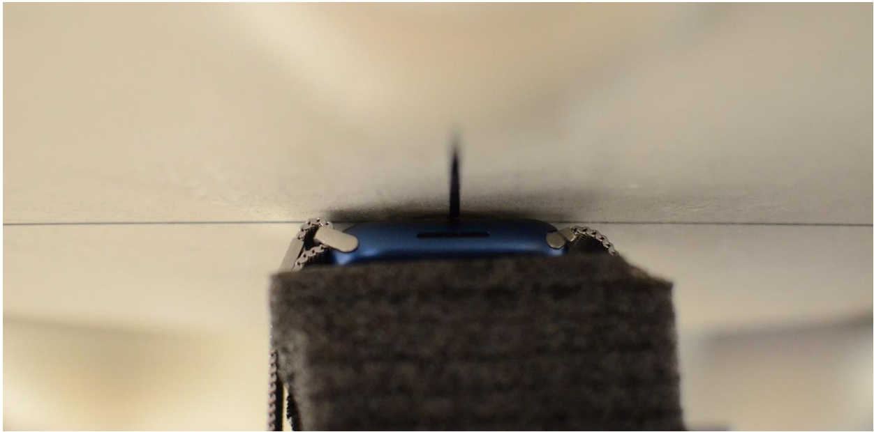
SAR Test Setup Photo 12: Aluminum with Metal Loop Wristband, Extremity, Back side at 0.0 cm
