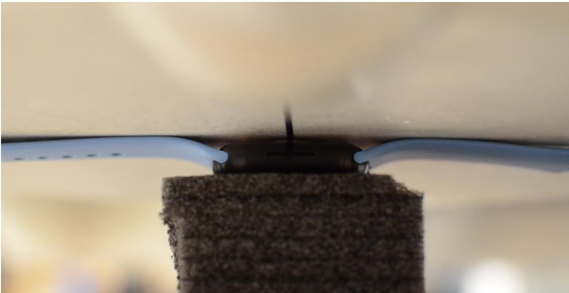
SAR Test Setup Photo 16: Titanium with Sport Wristband, Extremity, Back side at 0.0 cm
