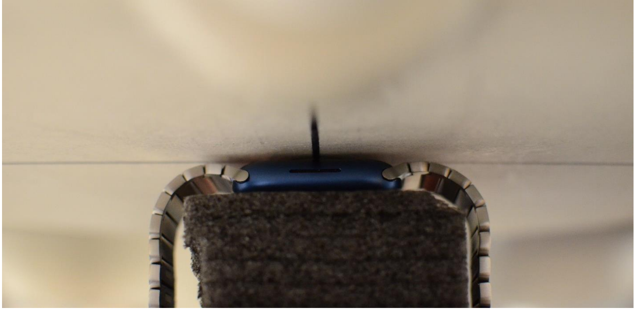
SAR Test Setup Photo 11: Aluminum with Metal Links Wristband, Extremity, Back side at 0.0 cm
