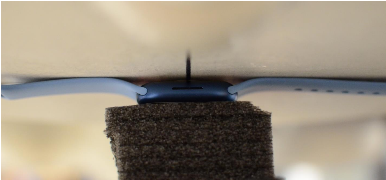
SAR Test Setup Photo 10: Aluminum with Sport Wristband, Extremity, Back side at 0.0 cm
