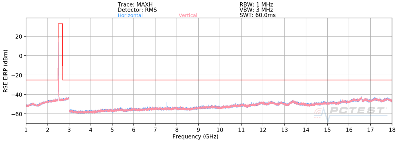
Plot 7-54. Antenna FCM Radiated Spurious Plot 1GHz – 18GHz (LTE Band 41)
