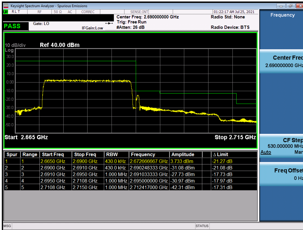
Plot 7-50. Upper ACP Plot (LTE Band 41 - 20MHz QPSK – Full RB)
