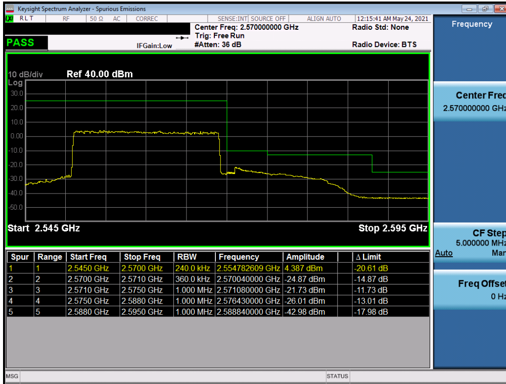
Plot 7-42. Upper ACP Plot (LTE Band 7 - 20MHz QPSK – Full RB)
