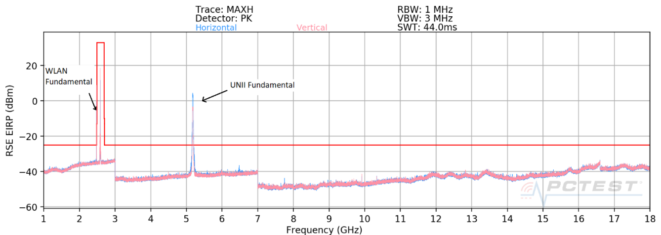
Plot 7-58. Radiated Spurious Emissions - Simultaneous Transmission 1-18GHz
