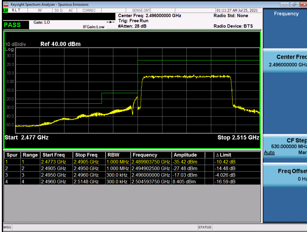
Plot 7-47. Lower ACP Plot (LTE Band 41 - 15MHz QPSK – Full RB)
