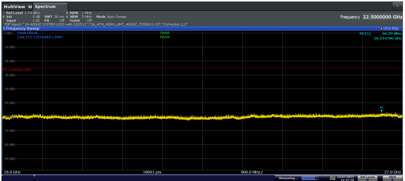
Plot 7-55. Antenna FCM Radiated Spurious Emission above 18GHz (LTE Band 41, Pol. H)
