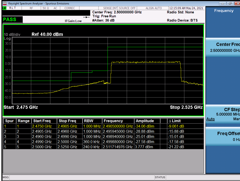
Plot 7-41. Lower ACP Plot (LTE Band 7 - 20MHz QPSK – Full RB)
