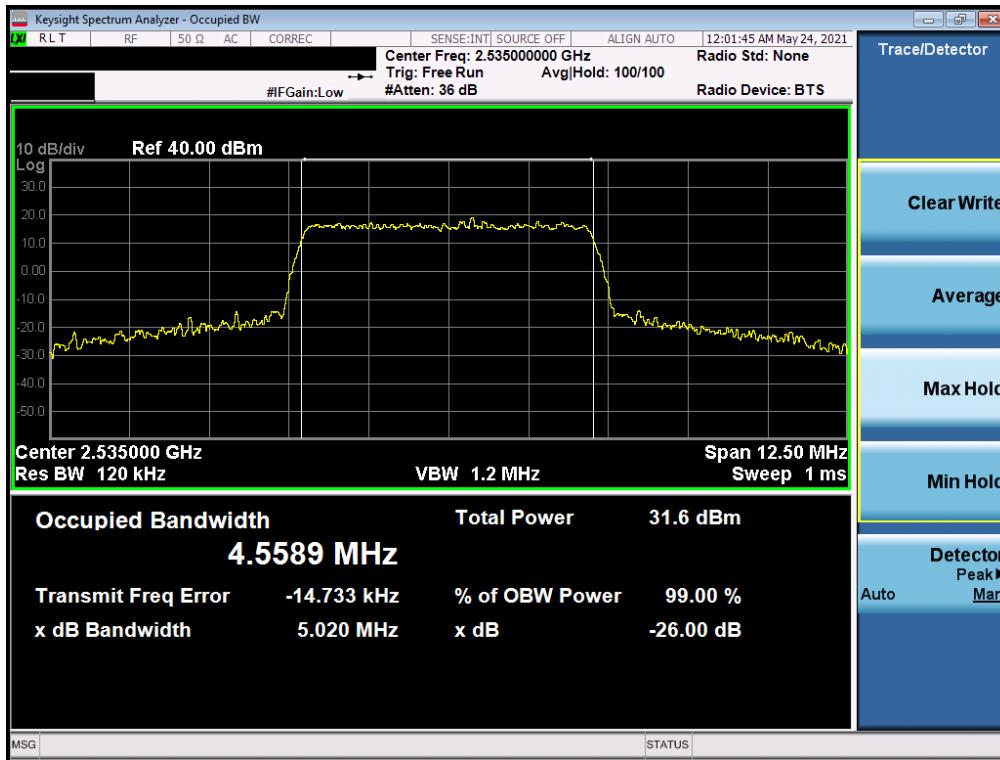
Plot 7-2. Occupied Bandwidth Plot (LTE Band 7 - 5MHz 16-QAM - Full RB)
