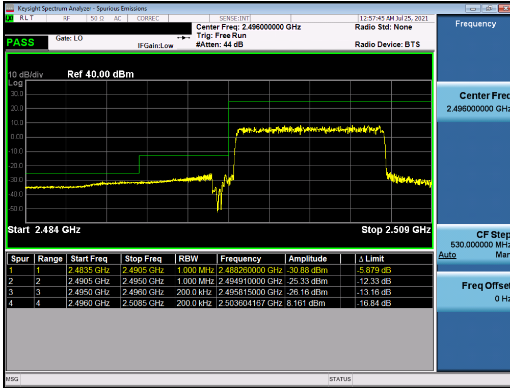
Plot 7-45. Lower ACP Plot (LTE Band 41 - 10MHz QPSK - Full RB)
