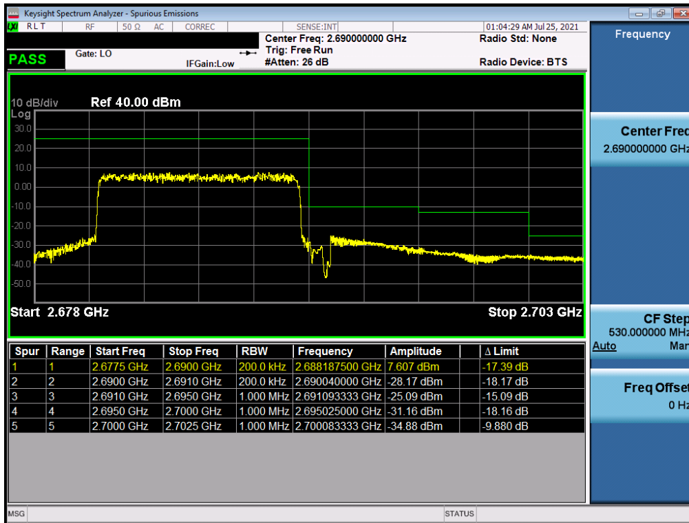
Plot 7-46. Upper ACP Plot (LTE Band 41 - 10MHz QPSK - Full RB)
