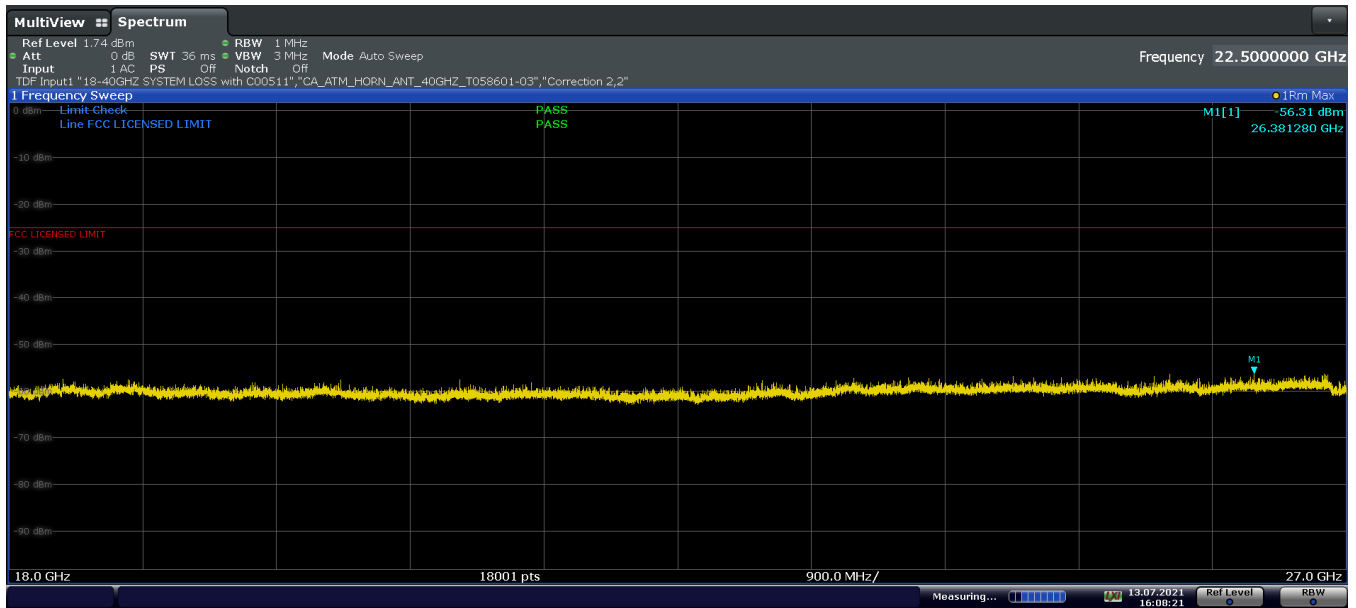
Plot 7-52. Antenna FCM Radiated Spurious Emission above 18GHz (LTE Band 7, Pol. H)
