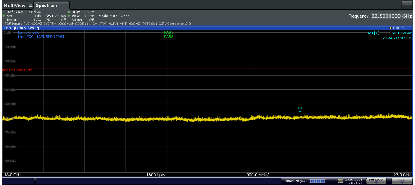
Plot 7-56. Antenna FCM Radiated Spurious Emission above 18GHz (LTE Band 41, Pol. V)
