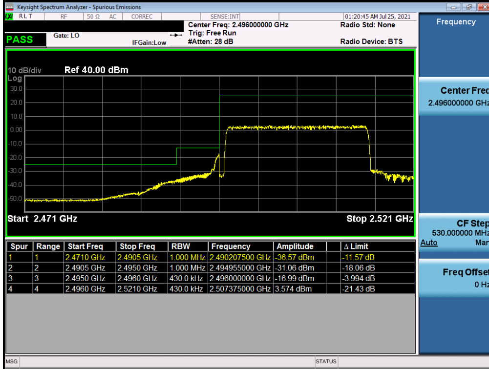
Plot 7-49. Lower ACP Plot (LTE Band 41 - 20MHz QPSK – Full RB)
