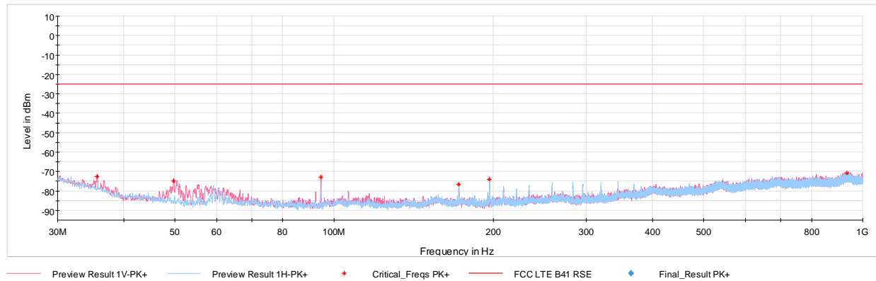
Plot 7-57. Radiated Spurious Emissions – Simultaneous Transmission 30MHz – 1GHz
