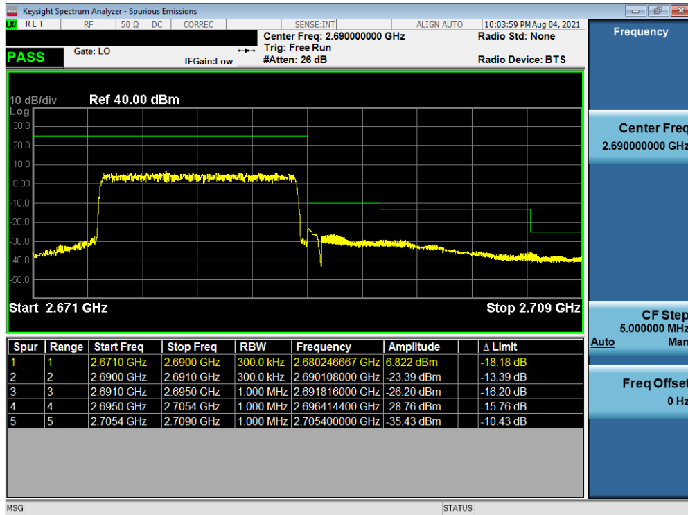
Plot 7-48. Upper ACP Plot (LTE Band 41 - 15MHz QPSK – Full RB)
