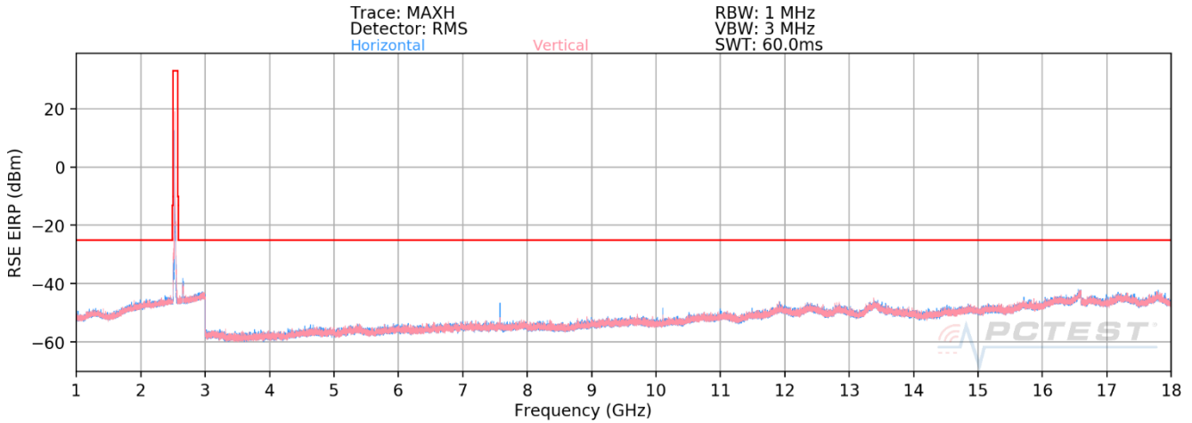
Plot 7-51. Antenna FCM Radiated Spurious Plot 1GHz – 18GHz (LTE Band 7)
