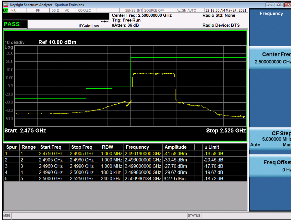
Plot 7-37. Lower ACP Plot (LTE Band 7 - 10MHz QPSK – Full RB)
