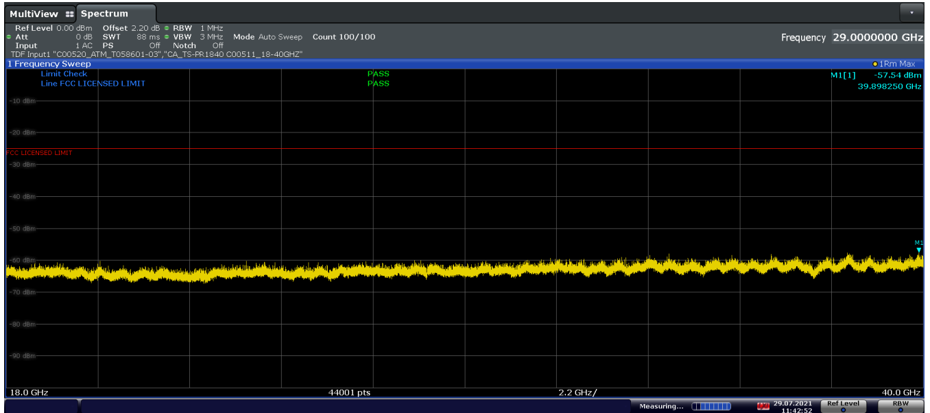
Plot 7-60. Radiated Spurious Emissions - Simultaneous Transmission 18GHz-40GHz Pol. V
