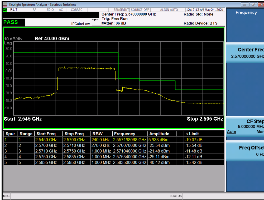
Plot 7-40. Upper ACP Plot (LTE Band 7 - 15MHz QPSK – Full RB)
