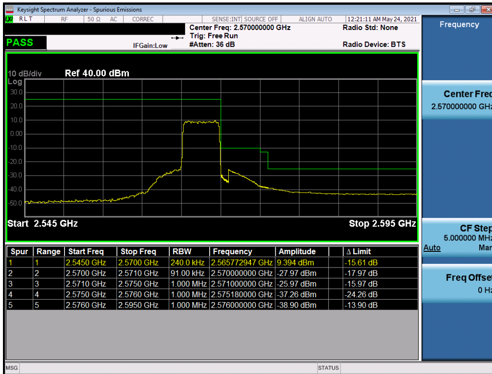
Plot 7-36. Upper ACP Plot (LTE Band 7 - 5MHz QPSK – Full RB)
