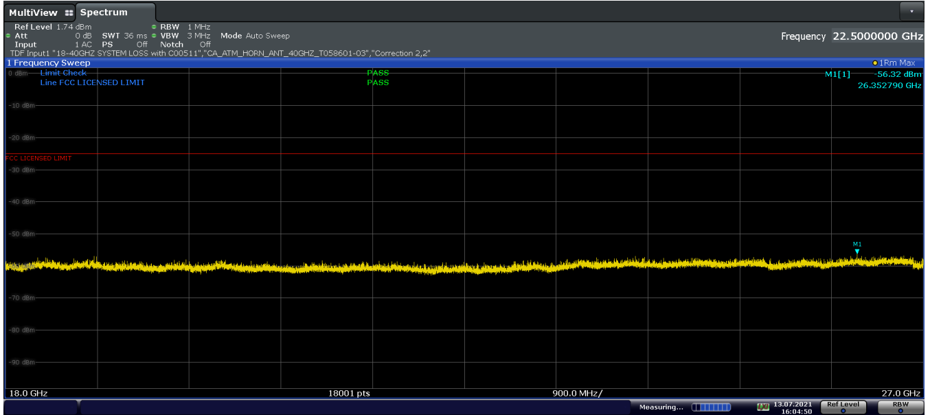
Plot 7-53. Antenna FCM Radiated Spurious Emission above 18GHz (LTE Band 7, Pol. V)
