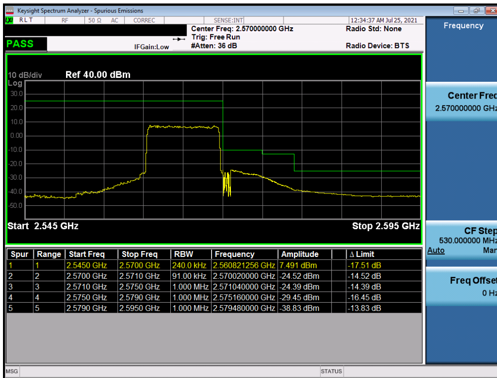
Plot 7-38. Upper ACP Plot (LTE Band 7 - 10MHz QPSK – Full RB)
