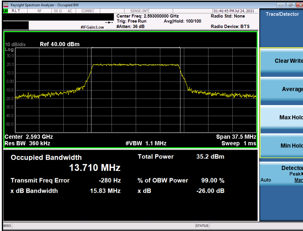
Plot 7-13. Occupied Bandwidth Plot (LTE Band 41 - 15MHz QPSK - Full RB)
