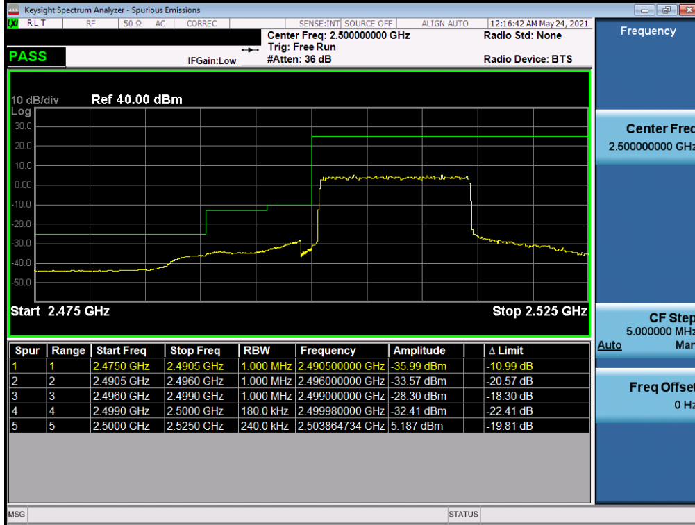
Plot 7-39. Lower ACP Plot (LTE Band 7 - 15MHz QPSK – Full RB)
