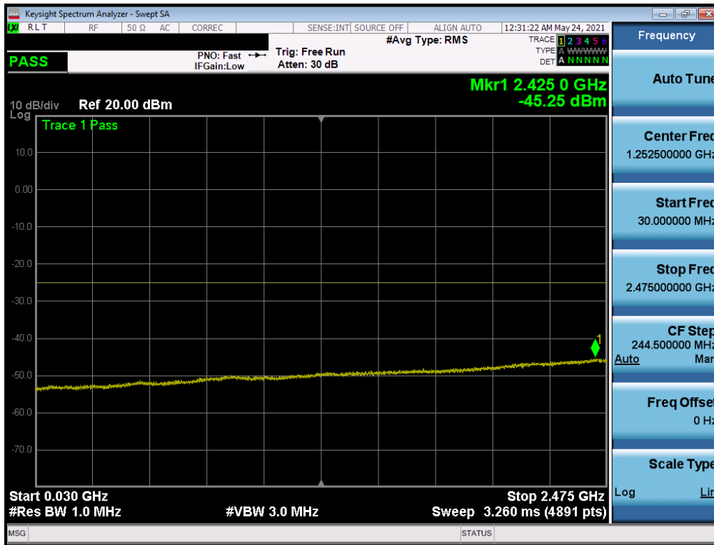
Plot 7-17. Conducted Spurious Plot (LTE Band 7 - 20MHz QPSK - RB Size 1, RB Offset 0 - Low Channel)
