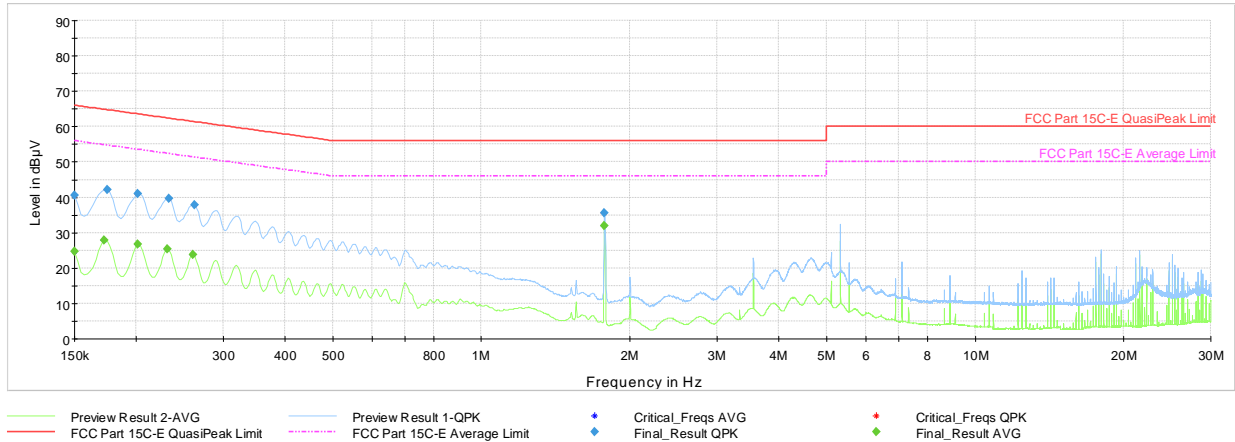
Plot 7-40. AC Line Conducted Plot with Bluetooth LE (1Mbps, ePA – Ch.19, N, with AC/DC Adapter + Magnetic Charger)
