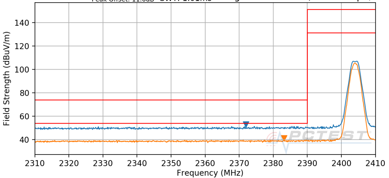
Plot 7-36. Radiated Restricted Lower Band Edge Measurement (Average & Peak)
