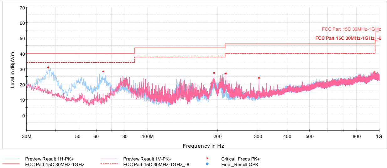
Plot 7-38. Radiated Spurious Plot Below 1GHz 1Mbps, ePA – Ch.19, Pol. H & V, with AC/DC Adapter + Magnetic Charger)
