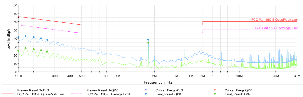
Plot 7-39. AC Line Conducted Plot with Bluetooth LE (1Mbps, ePA – Ch.19, L1, with AC/DC Adapter + Magnetic Charger)
