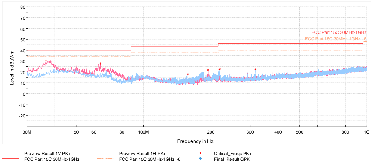
Plot 7-44. Radiated Spurious Emission – Simultaneous Transmission below 960 MHz with AC/DC Adapter + Magnetic Charger
