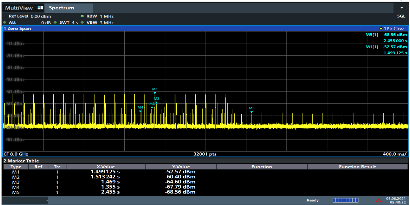
Plot 7-13. Zoom in Cessation Time – Mode1 (Ch. 9, 8 GHz)
