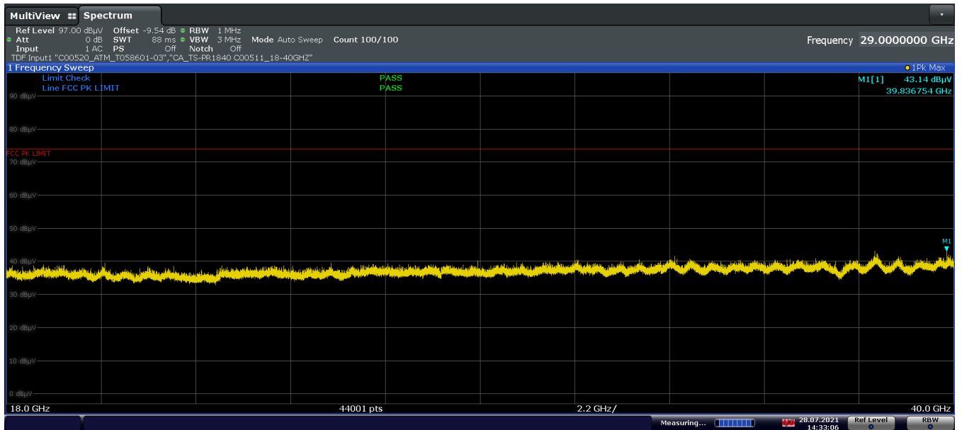
Plot 7-41. Radiated Spurious Emission- Simultaneous Transmission 18GHz-40GHz Pol. V
