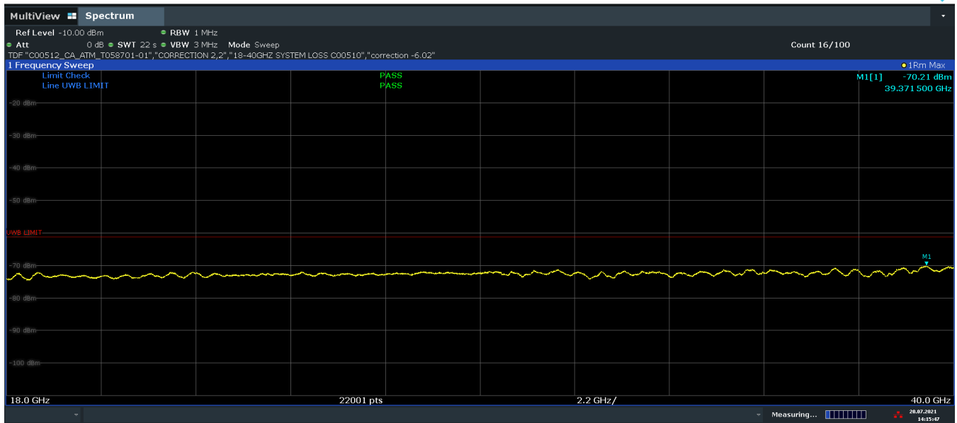
Plot 7-38. Radiated Spurious Emission 18-40GHz (Ch. 9, Config 3, Payload 125 Ant. Pol. V)
