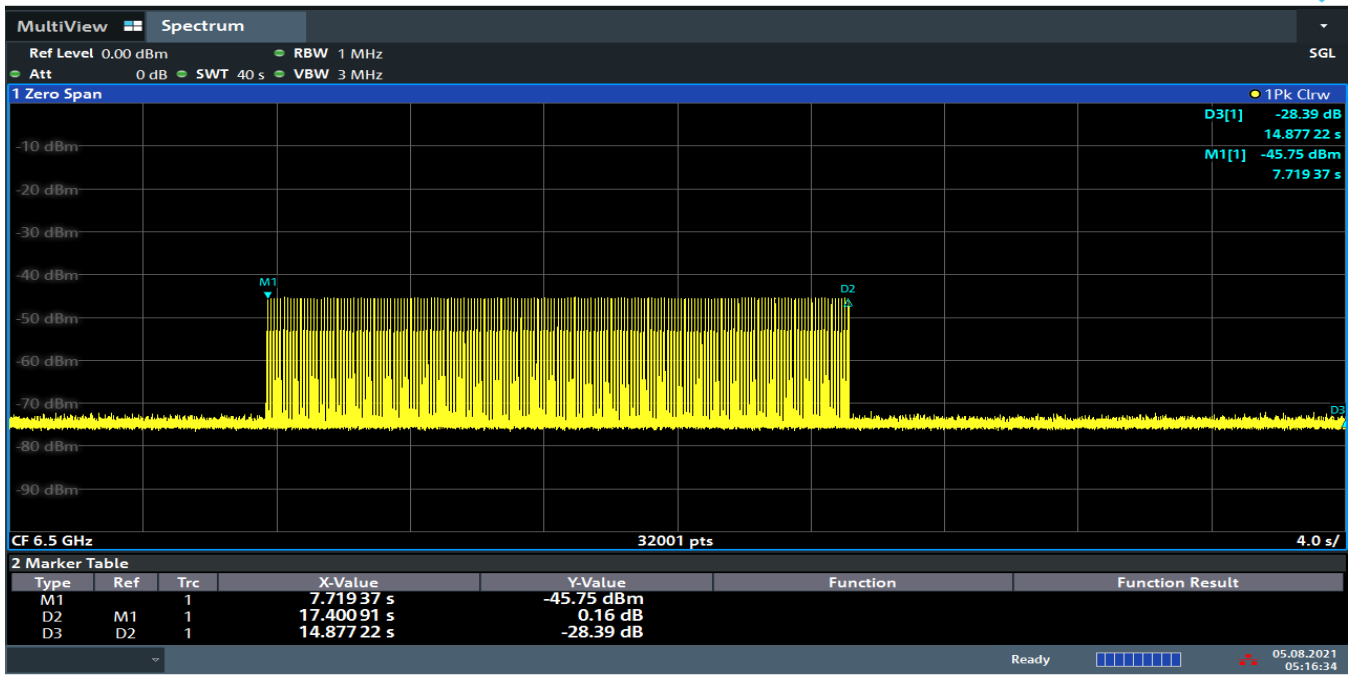
Plot 7-11. Cessation Time – Mode2 (Ch. 5, 6.5 GHz)
