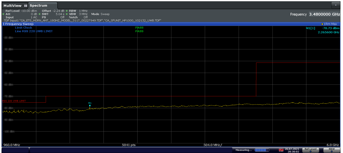
Plot 7-18. ISED Radiated Spurious Emission 960-6000MHz (Ch. 5, Config 3, Payload 125 Ant. Pol. V)
