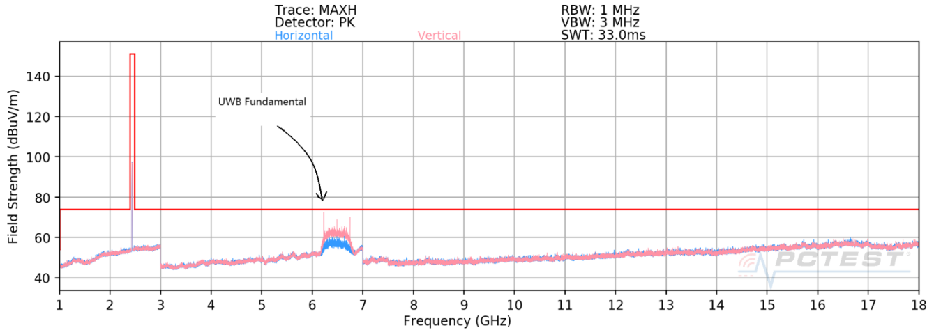
Plot 7-39. Radiated Spurious Simultaneous Transmission 1-18GHz (Ch. 5, Config 3, Payload 125)
