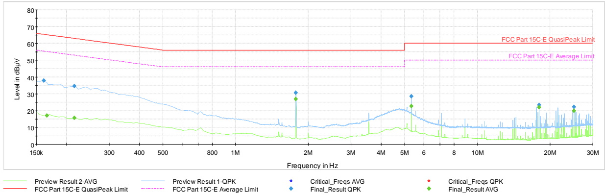
Plot 7-47. AC Line Conducted (Ch. 9, Config 3, Payload 125 L1, with AC/DC Adapter + Magnetic Charger)
