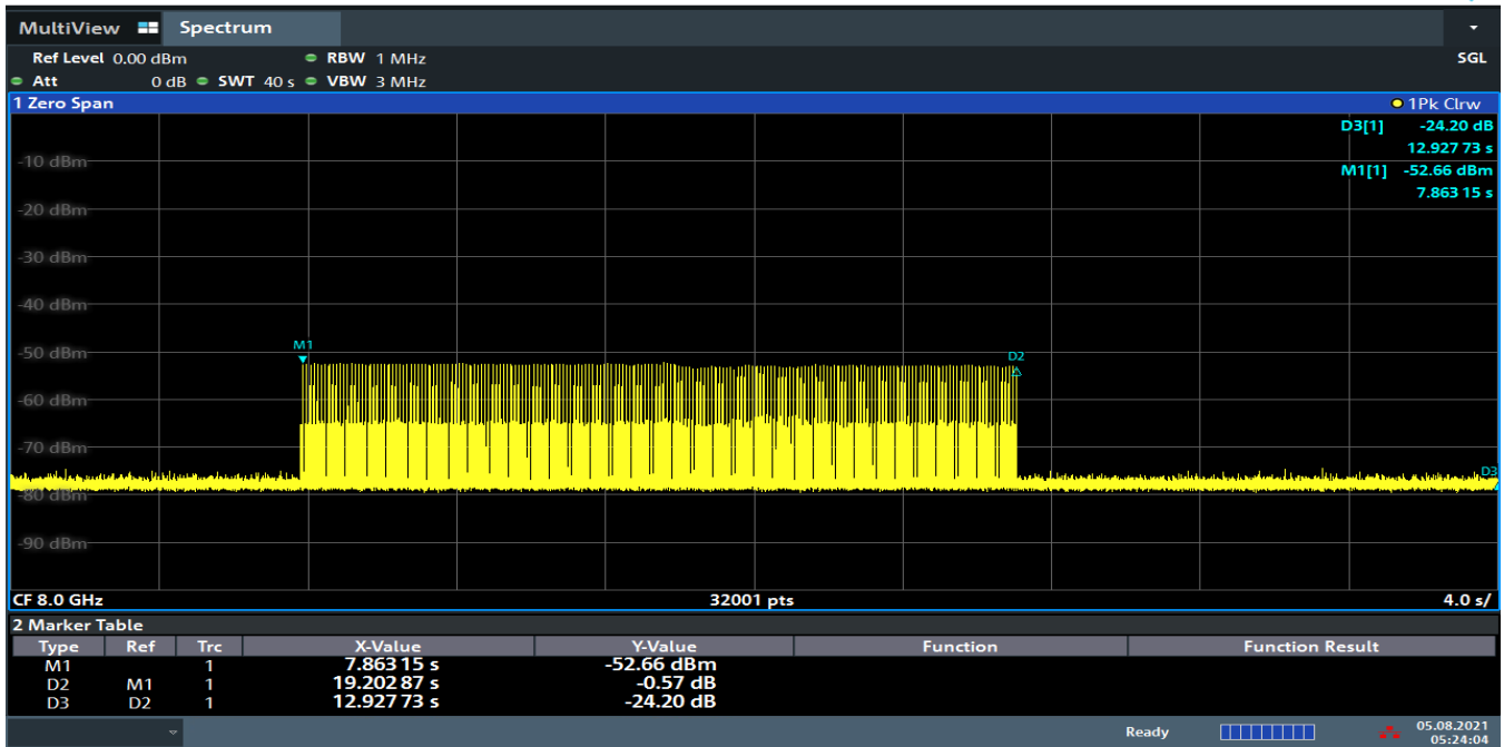
Plot 7-14. Cessation Time – Mode2 (Ch. 9, 8 GHz)
