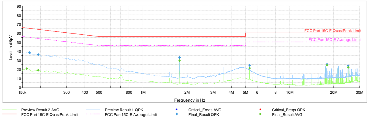
Plot 7-46. AC Line Conducted (Ch. 5, Config 3, Payload 125 N, with AC/DC Adapter + Magnetic Charger)
