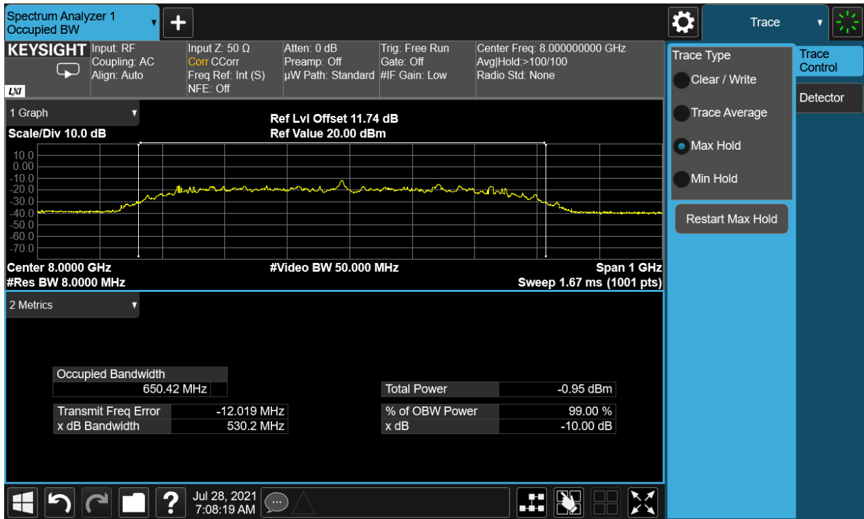
Plot 7-4. ISED 10dBc Bandwidth & 99% OBW (Ch. 9, Config 3/Payload 125)
