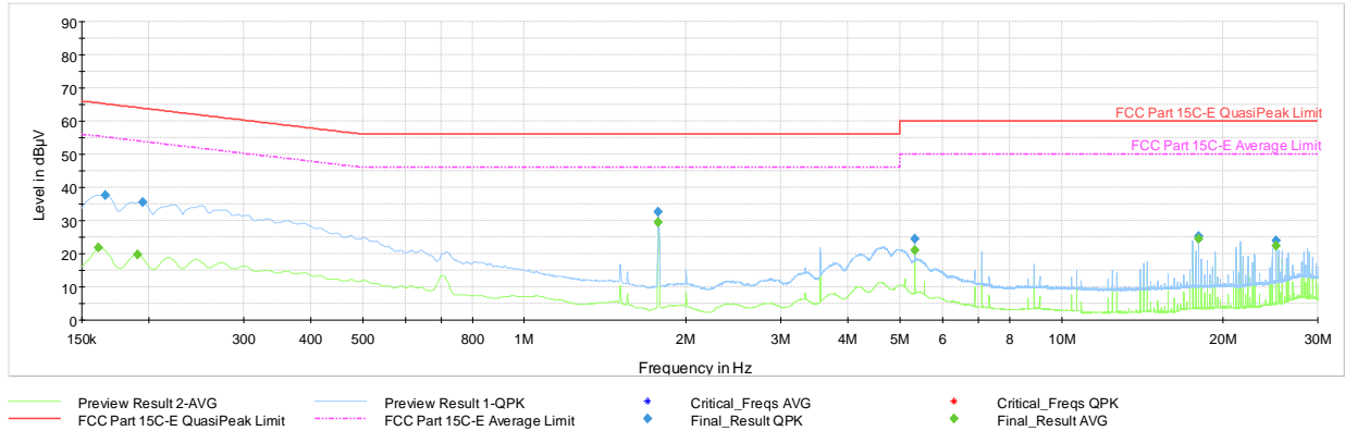
Plot 7-48. AC Line Conducted Plot (Ch. 9, Config 3, Payload 125 N, with AC/DC Adapter + Magnetic Charger)
