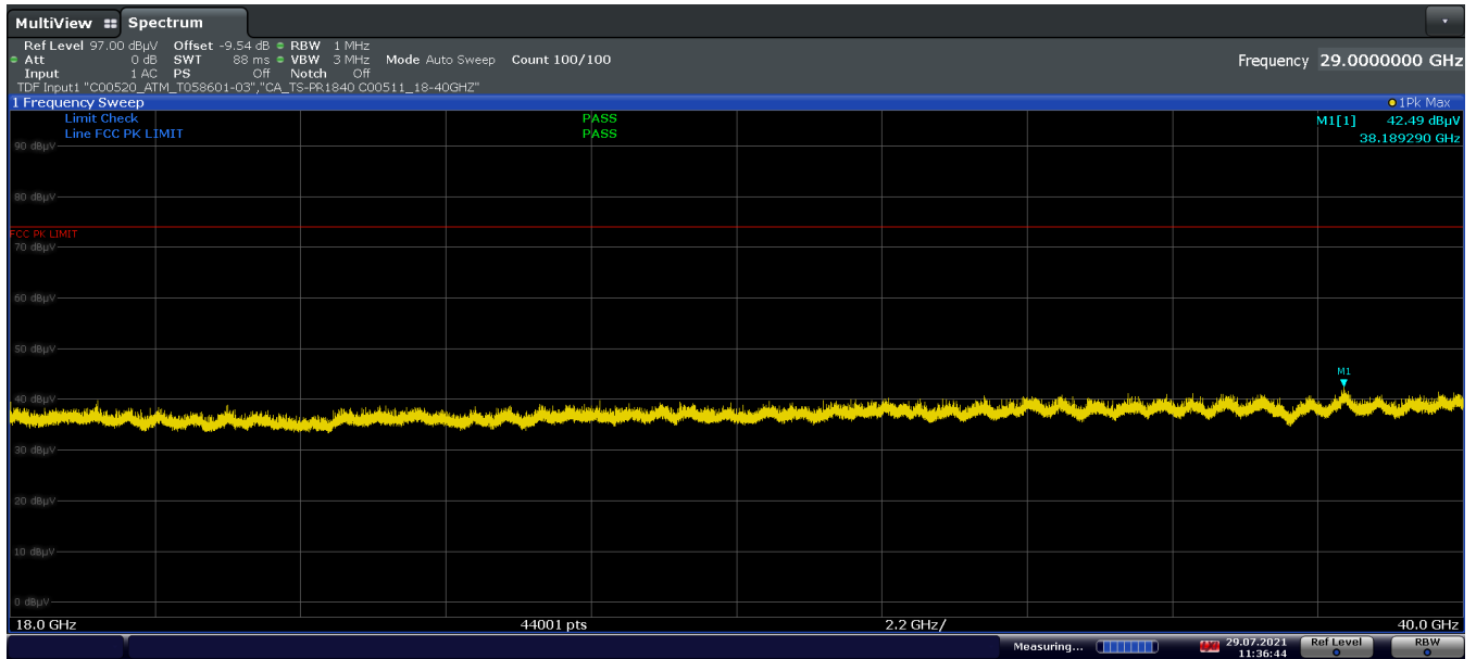
Plot 7-40. Radiated Spurious Emission- Simultaneous Transmission 18GHz-40GHz Pol. H
