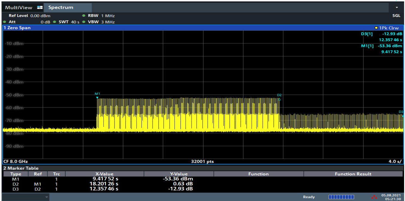
Plot 7-12. Cessation Time – Mode1 (Ch. 9, 8 GHz)
