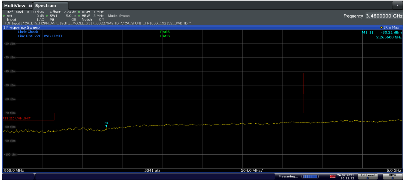
Plot 7-17. ISED Radiated Spurious Emission 960-6000MHz (Ch. 5, Config 3, Payload 125 Ant. Pol. H)
