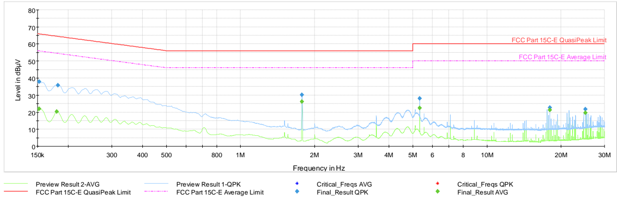
Plot 7-45. AC Line Conducted (Ch. 5, Config 3, Payload 125 L1, with AC/DC Adapter + Magnetic Charger)
