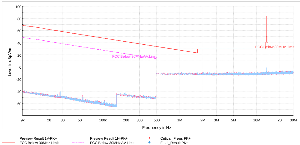
Plot 7-9. Radiated Spurious Emissions 9kHz – 30MHz (Reader 10% Ask 1 out of 256, with WCP + AC/DC Adapter)
