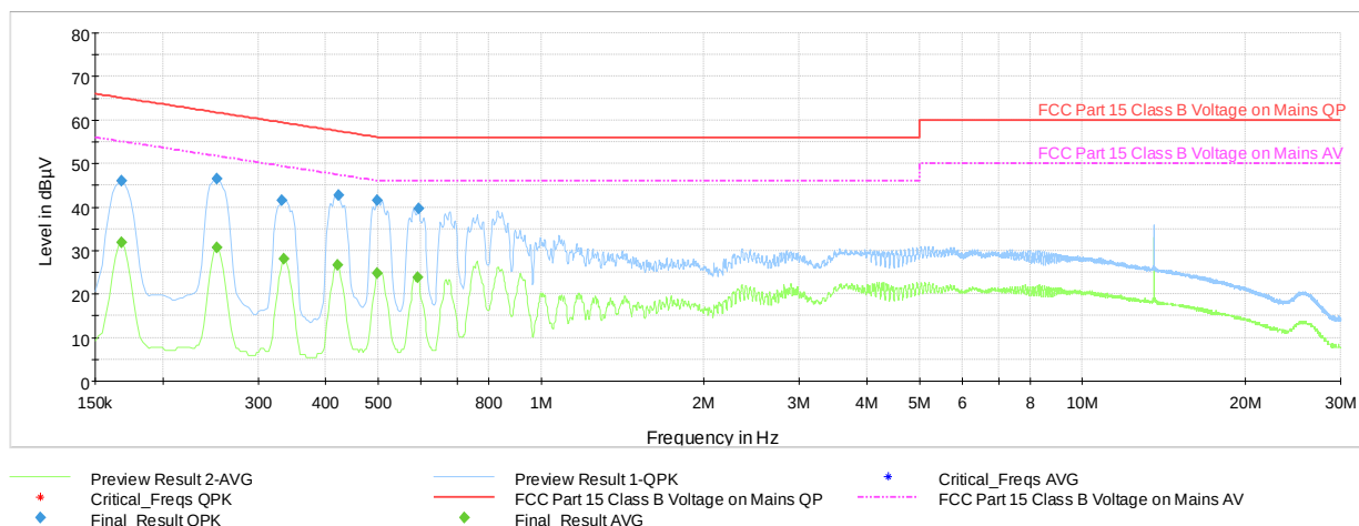
Plot 7-13. AC Line-Conducted Test Plot (N, with WCP + AC/DC Adapter)
