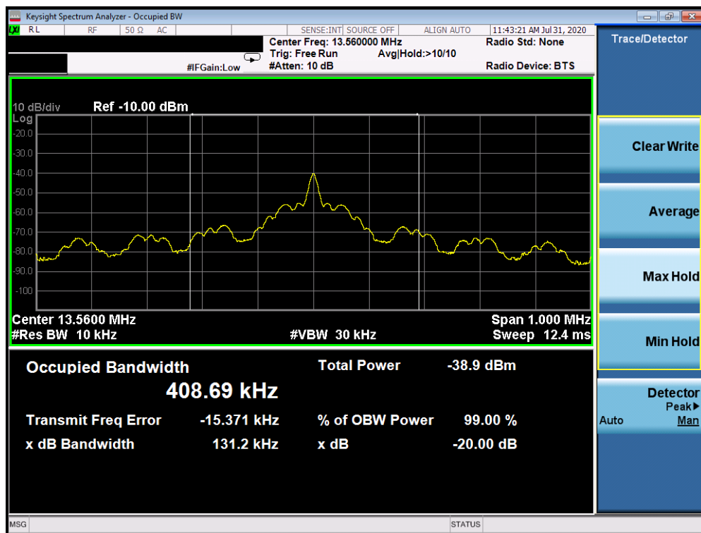
Plot 7-5. 20dB Bandwidth Plot (Reader 10% Ask 1 out of 256)
