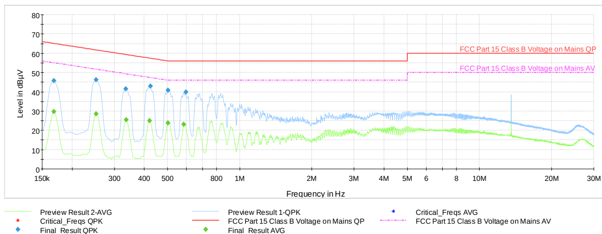
Plot 7-12. AC Line-Conducted Test Plot (L1, with WCP + AC/DC Adapter)
