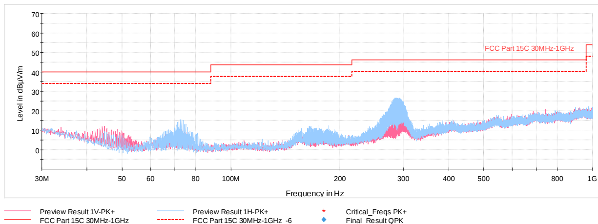
Plot 7-41. Radiated Spurious Emissions 30MHz-1GHz (GFSK ePA – Ch.39, with WCP + laptop)
