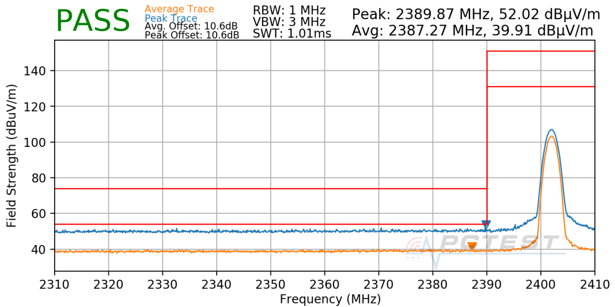
Plot 7-38. Radiated Restricted Lower Band Edge Measurement
