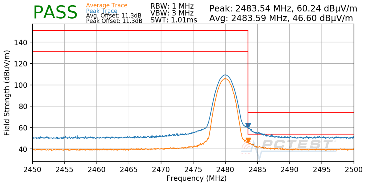
Plot 7-40. Radiated Restricted Upper Band Edge Measurement
