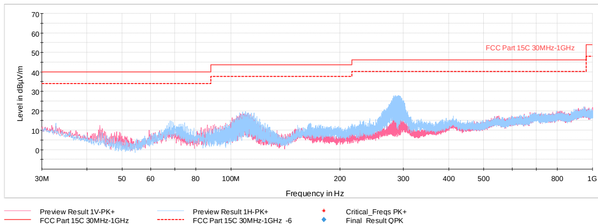
Plot 7-38. Radiated Spurious Emissions 30MHz-1GHz (1Mbps, ePA – Ch.19, with WCP + Laptop)
