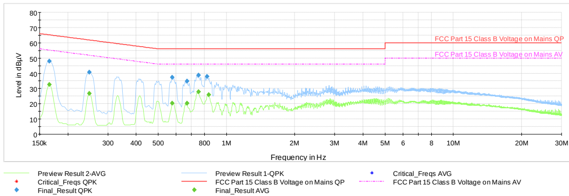
Plot 7-40. AC Line Conducted Emission with Bluetooth LE (N - 1Mbps, ePA, Ch.19, with WCP + AC/DC Adapter)
