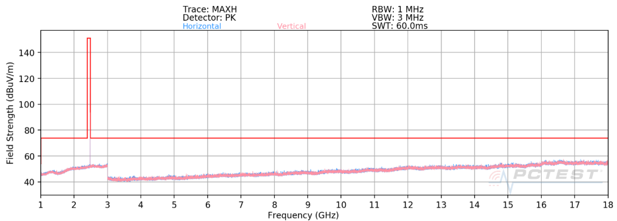
Plot 7-31. Radiated Spurious Emissions 1-18GHz (1Mbps ePA – Ch. 39)
