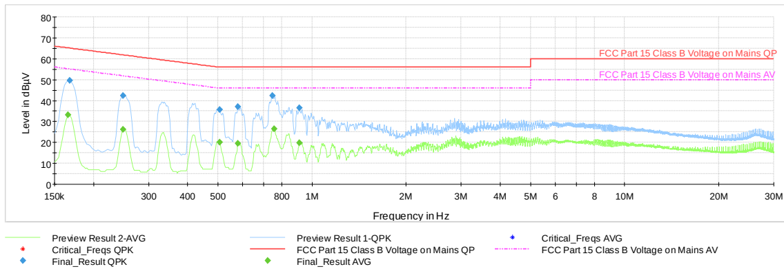
Plot 7-39. AC Line Conducted Emission with Bluetooth LE (L1 - 1Mbps, ePA, Ch.19, with WCP + AC/DC Adapter)
