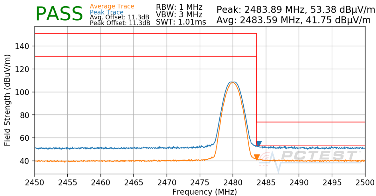
Plot 7-36. Radiated Restricted Upper Band Edge Measurement
