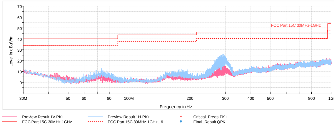
Plot 7-38. Radiated Spurious Emissions 30MHz-1GHz (4Mbps, ePA – Ch.38, with WCP + laptop)
