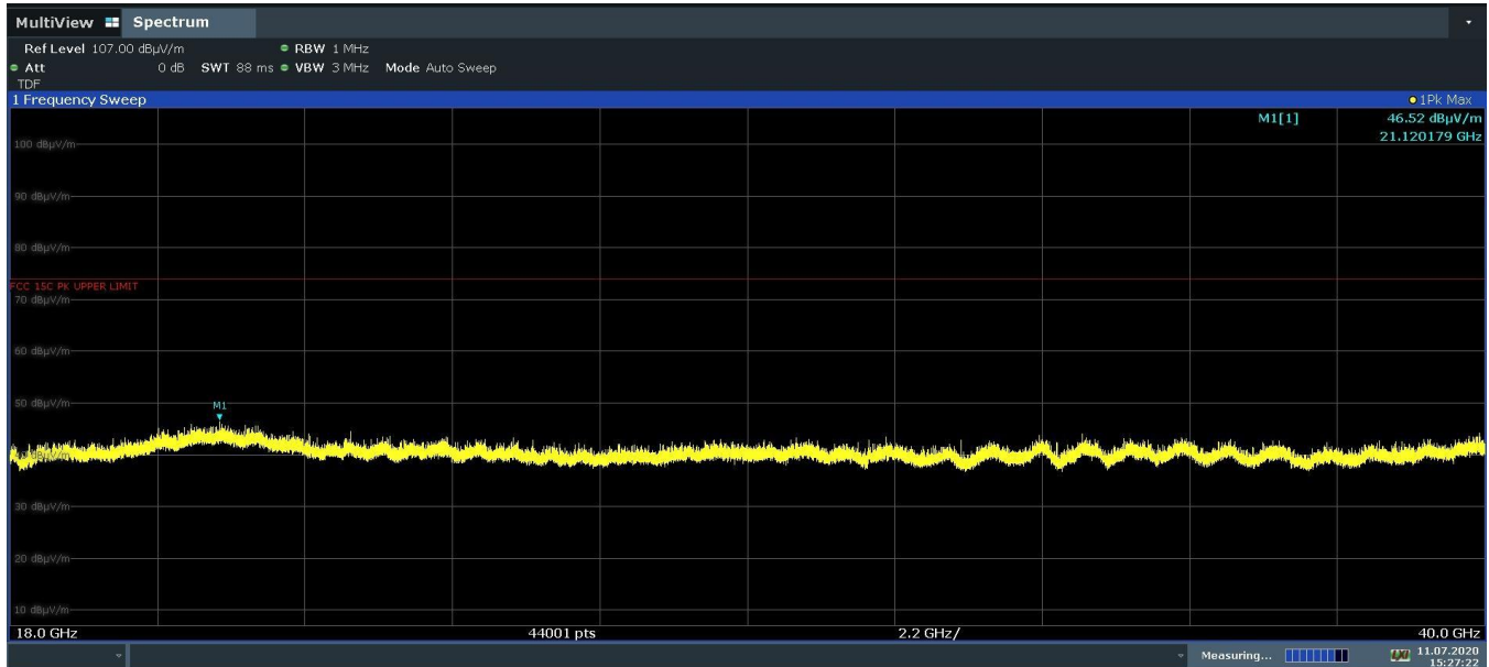
Plot 7-37. Radiated Spurious Emissions 18GHz - 40GHz – H Polarity (802.11n Ch 52)
