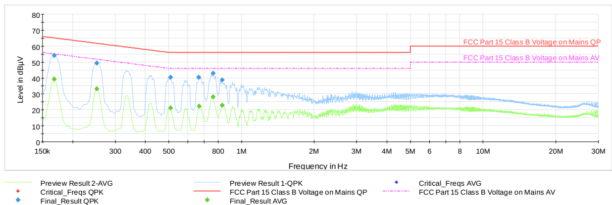
Plot 7-51. AC Line Conducted Plot with 802.11n UNII Band 2A – Ch.52 (L1) with WCP + AC/DC Charger
