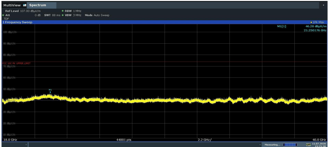
Plot 7-38. Radiated Spurious Emissions 18GHz - 40GHz – V Polarity (802.11n Ch 52)
