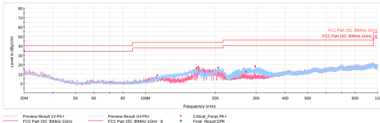
Plot 7-50. Radiated Spurious Emissions – Simultaneous Transmission below 1GHz with WCP + AC/DC Adapter
