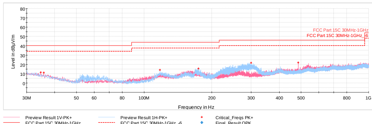
Plot 7-49. Radiated Spurious Emissions below 1GHz (802.11n – UNII 2A Ch. 52) with WCP + laptop
