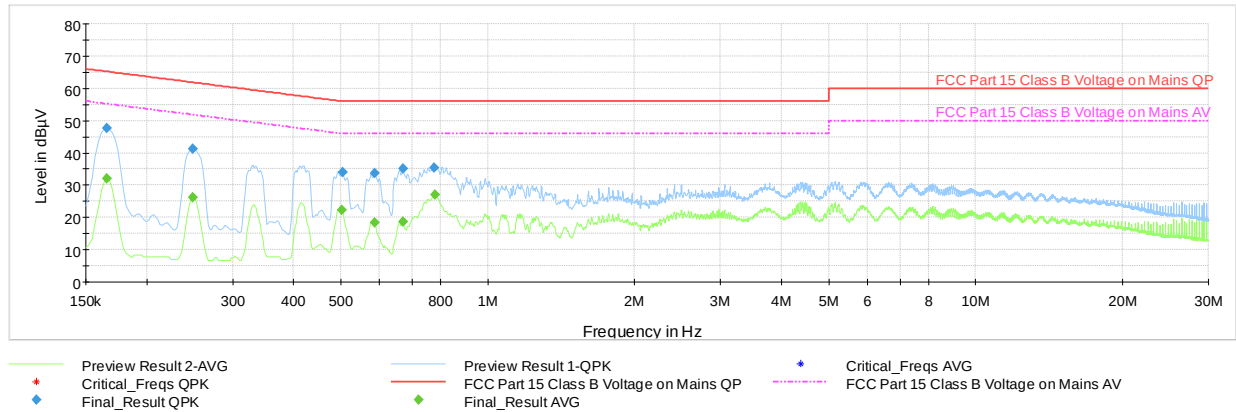
Plot 7-52. AC Line Conducted Plot with 802.11n UNII Band 2A – Ch.52 (N) with WCP + AC/DC Charger
