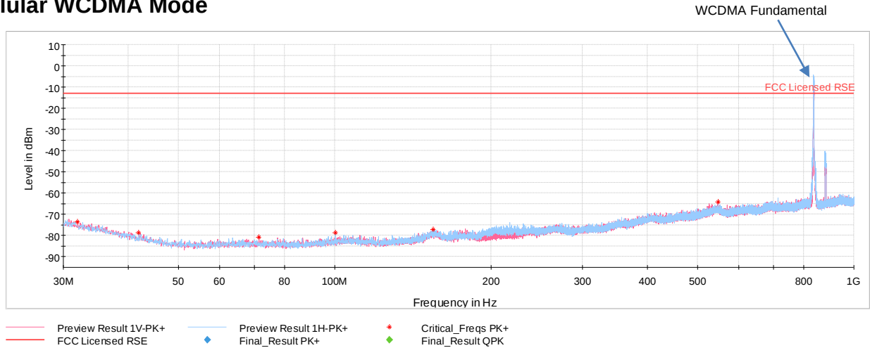
Plot 7-44. Radiated Spurious Emissions below 1GHz (Cellular WCDMA Mode – Ch. 4132)
