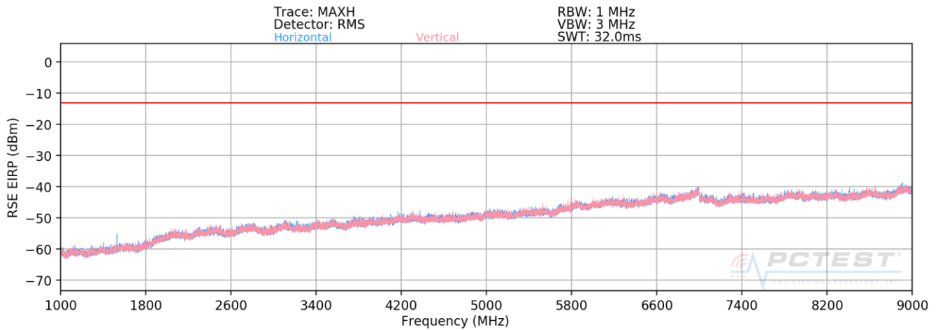
Plot 7-45. Radiated Spurious Emissions above 1GHz (Cellular WCDMA Mode – Ch. 4132)
