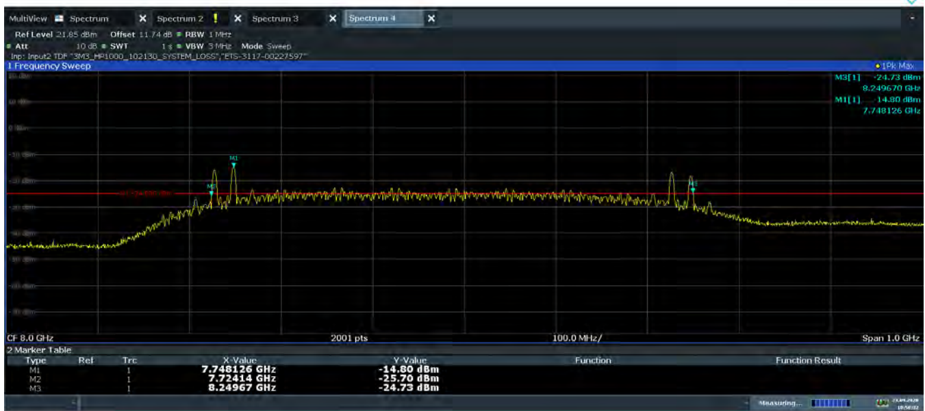
Plot 7-20. 10dBc Bandwidth (Ch. 9, Config 5/Payload 0)
