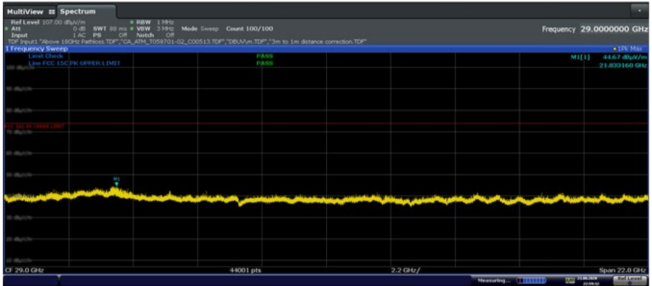
Plot 7-35. Radiated Spurious Emissions 18-40GHz (Simultaneous Transmission, Ant. Pol. H)
