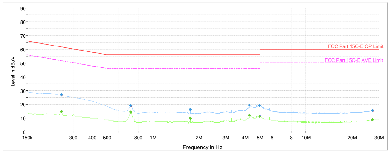
Plot 7-44. AC Line Conducted Emission with GFSK ePA Ch.0 (N, with AC/DC Adapter)
