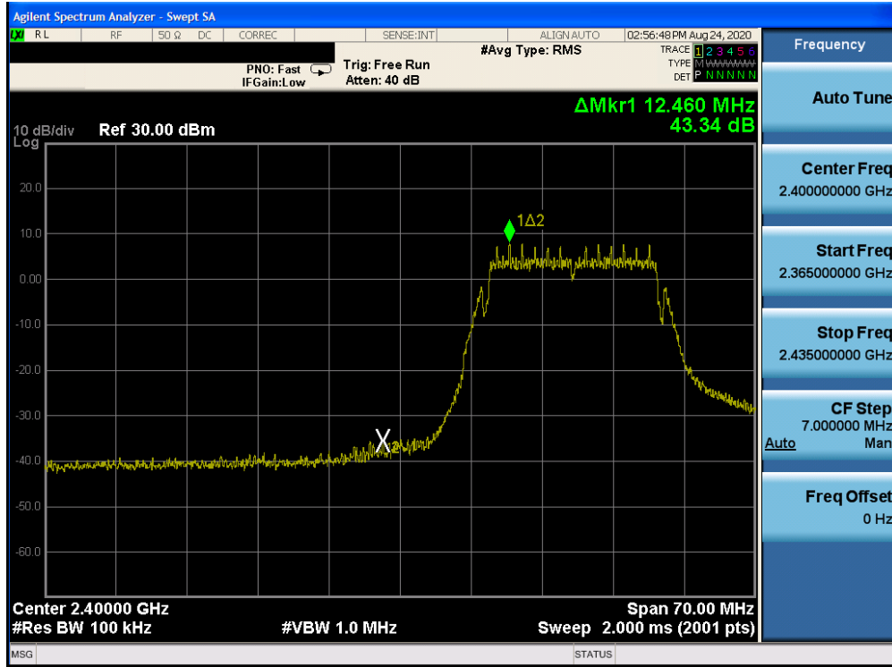
Plot 7-27: Band Edge Plot (802.11g– Ch. 2)
