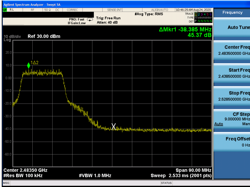
Plot 7-43: Band Edge Plot (802.11n (2.4GHz) – Ch. 9)
