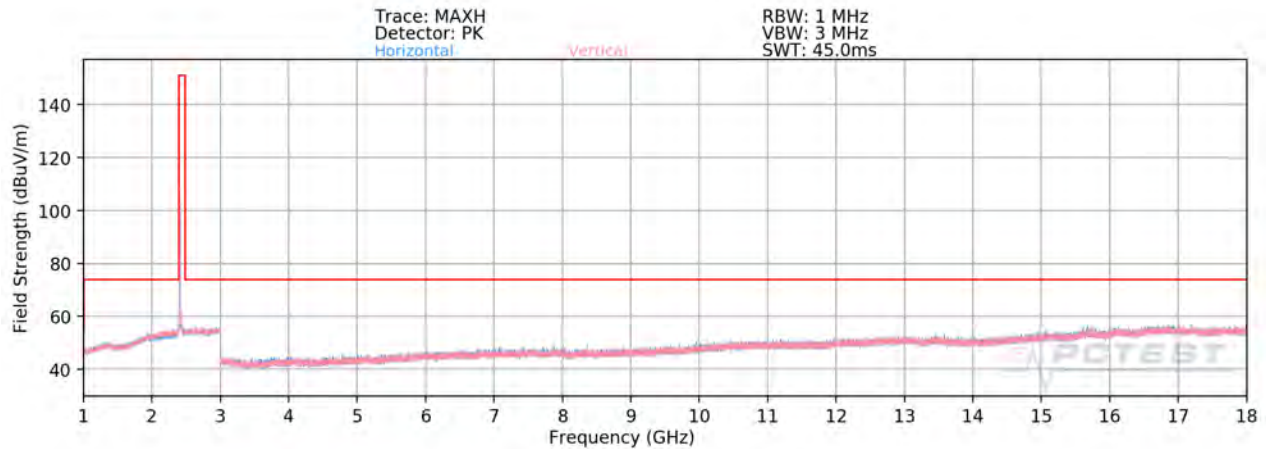
Plot 7-54. Radiated Spurious Emissions 1-18GHz (802.11b – Ch. 1)
