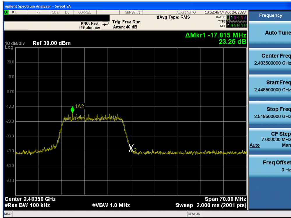
Plot 7-47: Band Edge Plot (802.11n (2.4GHz) - Ch. 13)
