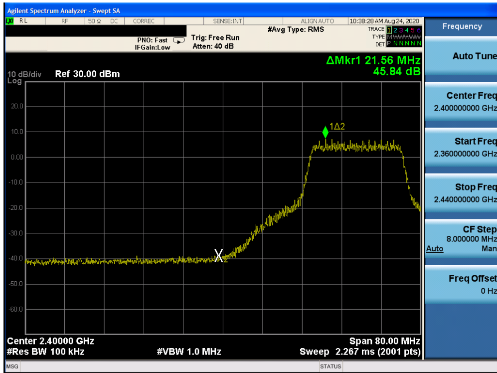
Plot 7-40: Band Edge Plot (802.11n (2.4GHz) – Ch. 4)
