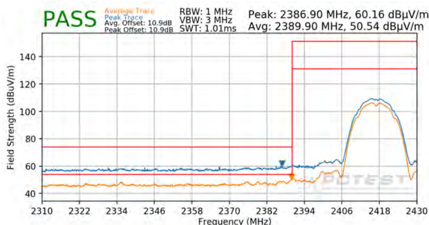
Plot 7-60: Radiated Restricted Lower Band Edge Measurement
