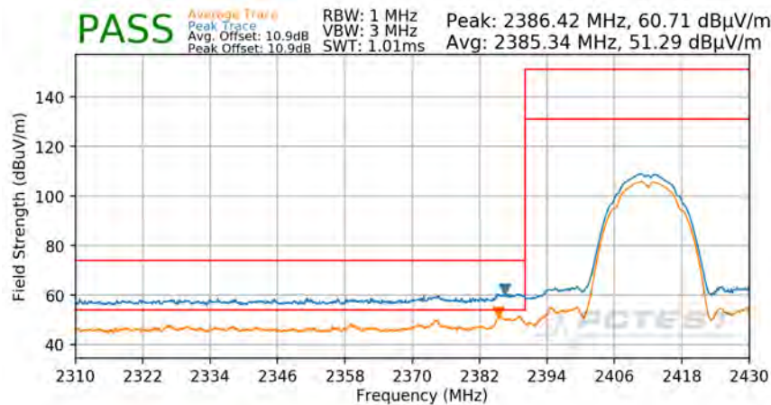
Plot 7-59: Radiated Restricted Lower Band Edge Measurement
