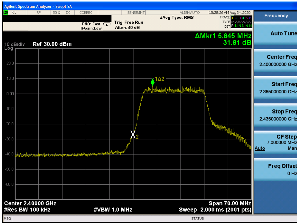
Plot 7-37. Band Edge Plot (802.11n (2.4GHz) – Ch. 1)
