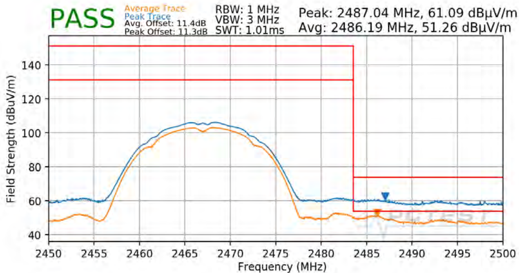
Plot 7-63: Radiated Restricted Upper Band Edge Measurement
