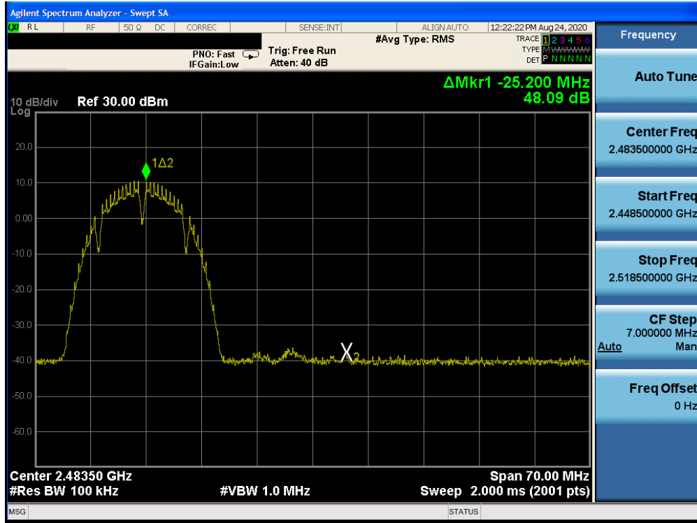
Plot 7-23: Band Edge Plot (802.11b - Ch.11)
