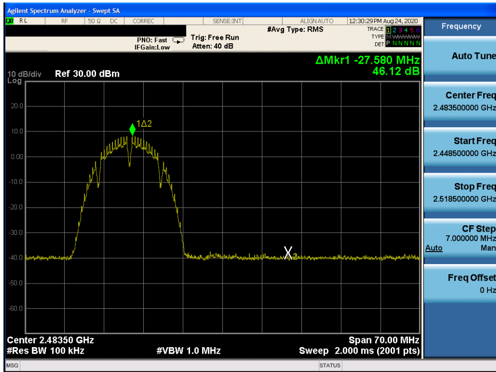
Plot 7-24: Band Edge Plot (802.11b - Ch.12)
