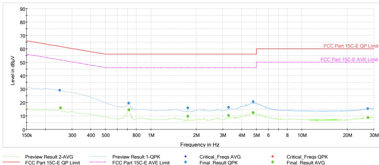
Plot 7-78. AC Line Conducted Emission with 802.11b (N with AC/DC Adapter)
