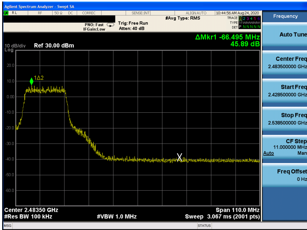
Plot 7-41: Band Edge Plot (802.11n (2.4GHz) – Ch. 7)
