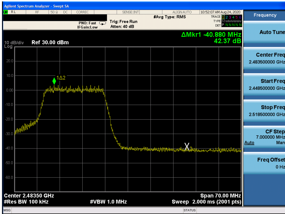
Plot 7-46: Band Edge Plot (802.11n (2.4GHz) – Ch. 12)
