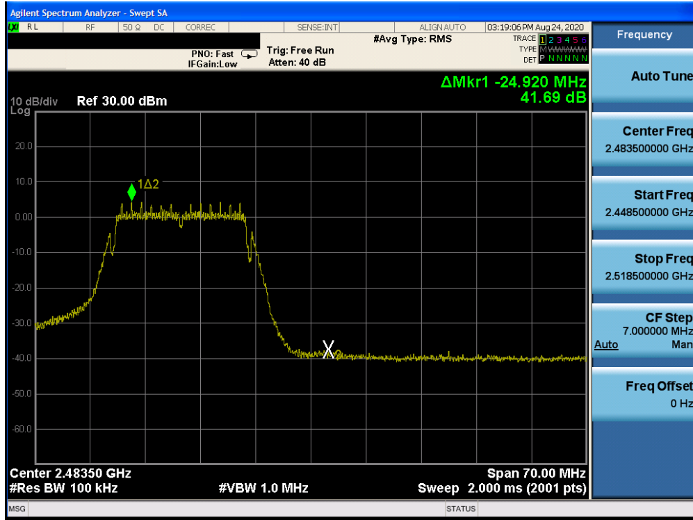
Plot 7-35: Band Edge Plot (802.11g– Ch. 12)
