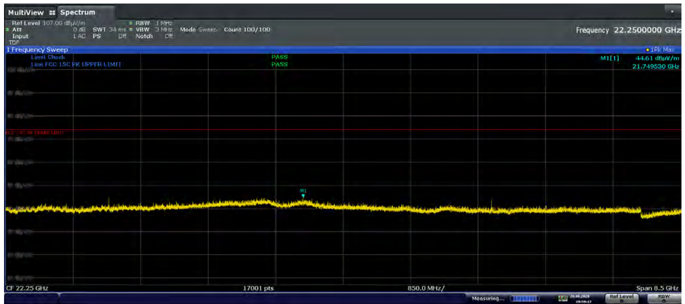
Plot 7-58: Radiated Spurious Plot 18-26.5GHz (802.11b – Ch. 1, Ant. Pol. V)
