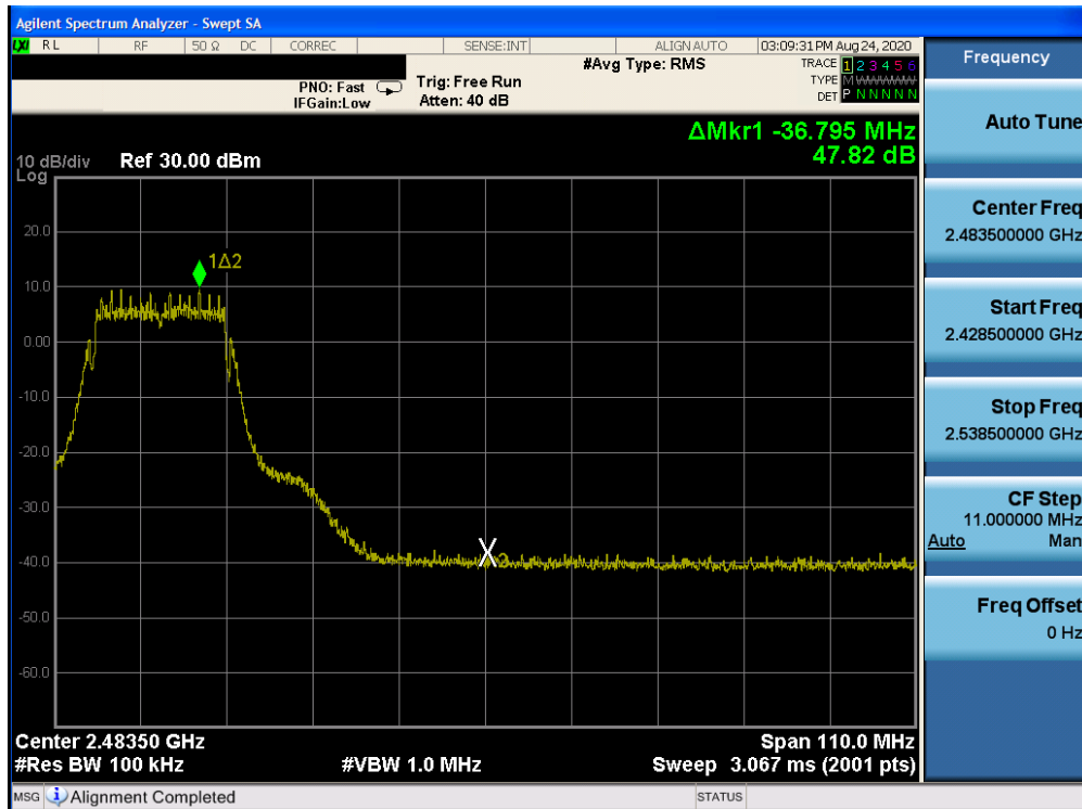
Plot 7-30: Band Edge Plot (802.11g– Ch. 7)
