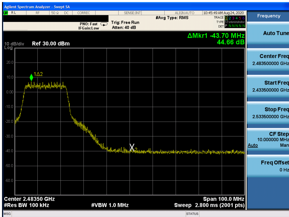
Plot 7-42: Band Edge Plot (802.11n (2.4GHz) – Ch. 8)
