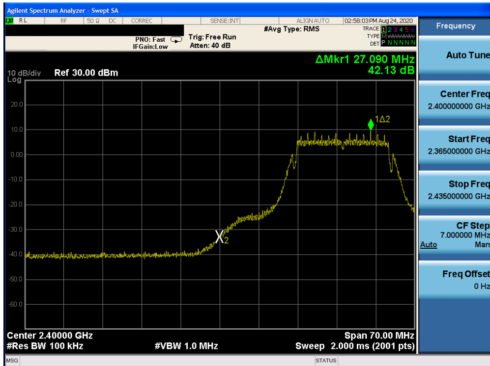
Plot 7-28: Band Edge Plot (802.11g– Ch. 3)
