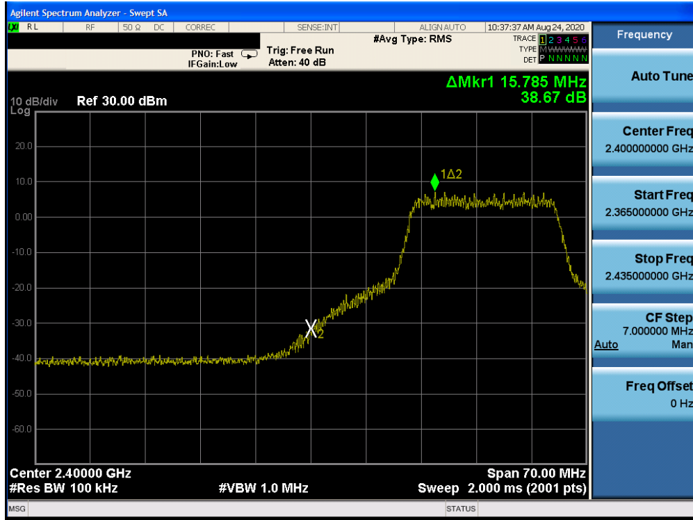
Plot 7-39: Band Edge Plot (802.11n (2.4GHz) – Ch. 3)
