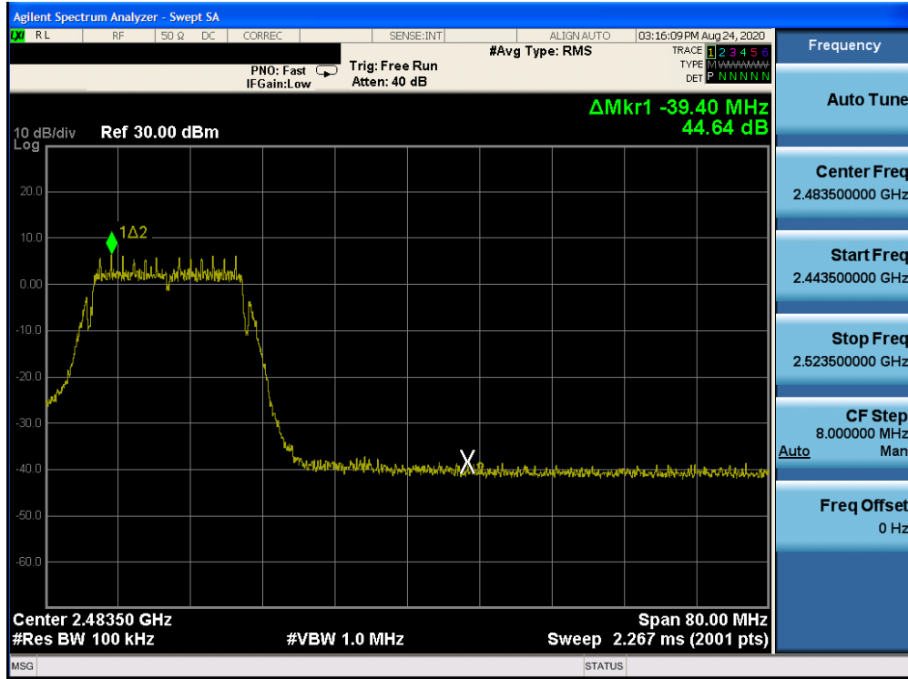
Plot 7-33: Band Edge Plot (802.11g– Ch. 10)
