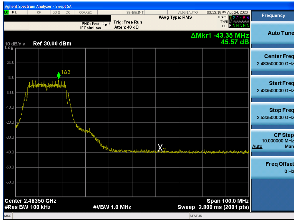
Plot 7-31: Band Edge Plot (802.11g– Ch. 8)
