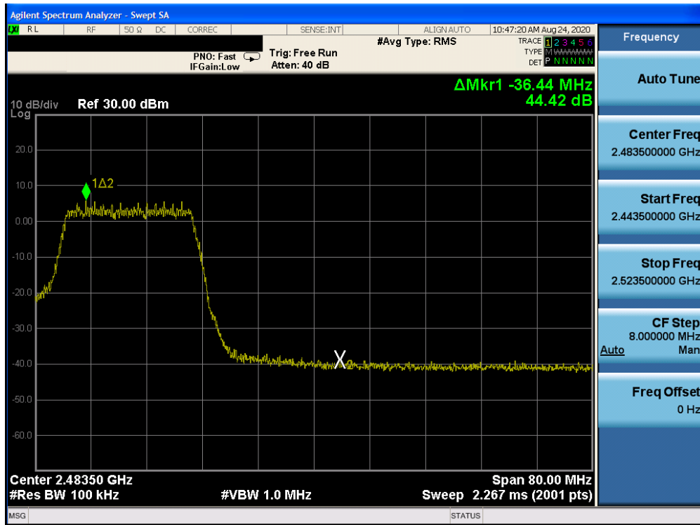
Plot 7-44: Band Edge Plot (802.11n (2.4GHz) – Ch. 10)
