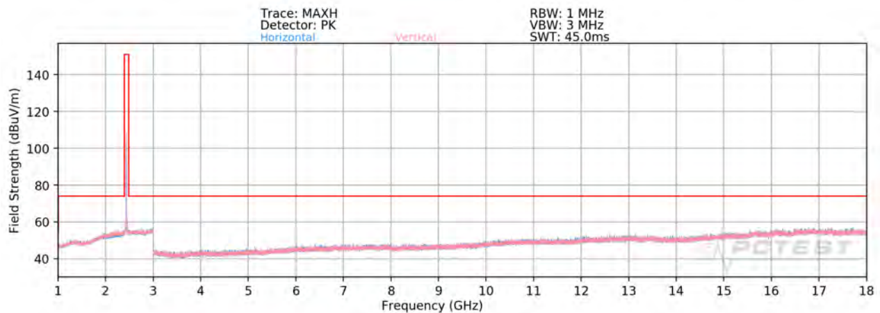
Plot 7-55. Radiated Spurious Emissions 1-18GHz (802.11b – Ch. 6)
