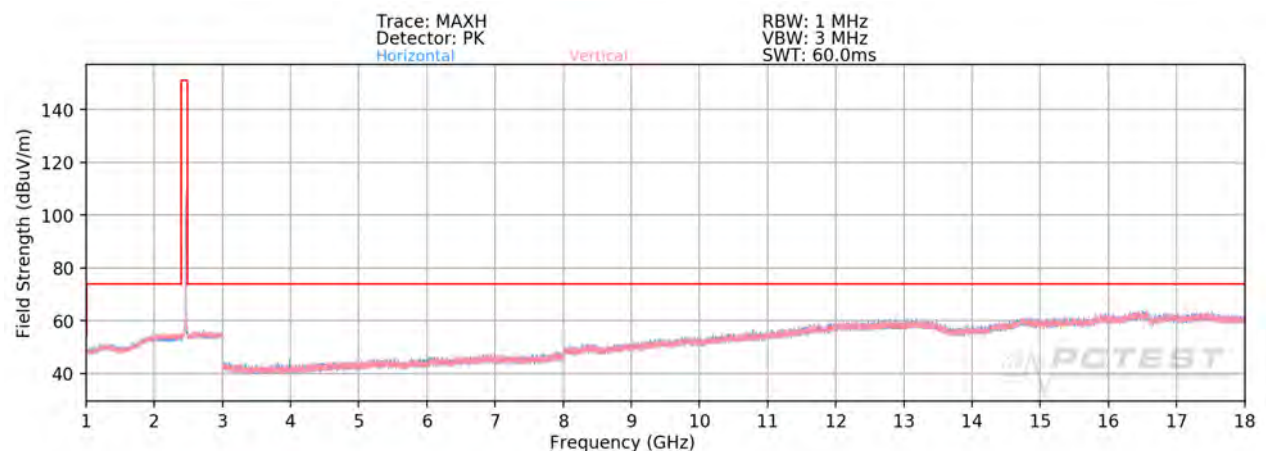
Plot 7-56. Radiated Spurious Emissions 1-18GHz (802.11b – Ch. 11)
