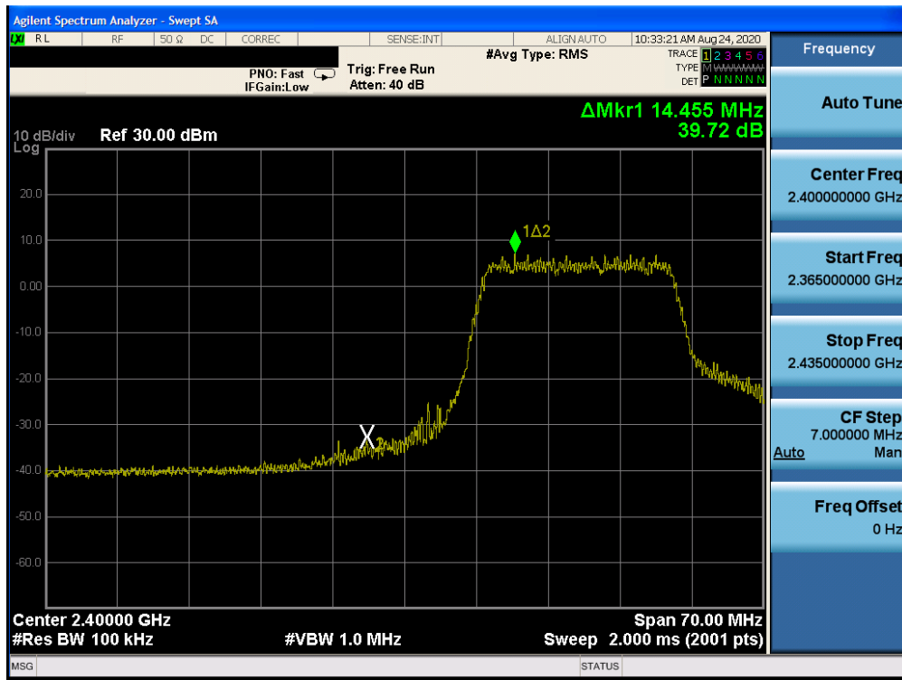
Plot 7-38: Band Edge Plot (802.11n (2.4GHz) – Ch. 2)
