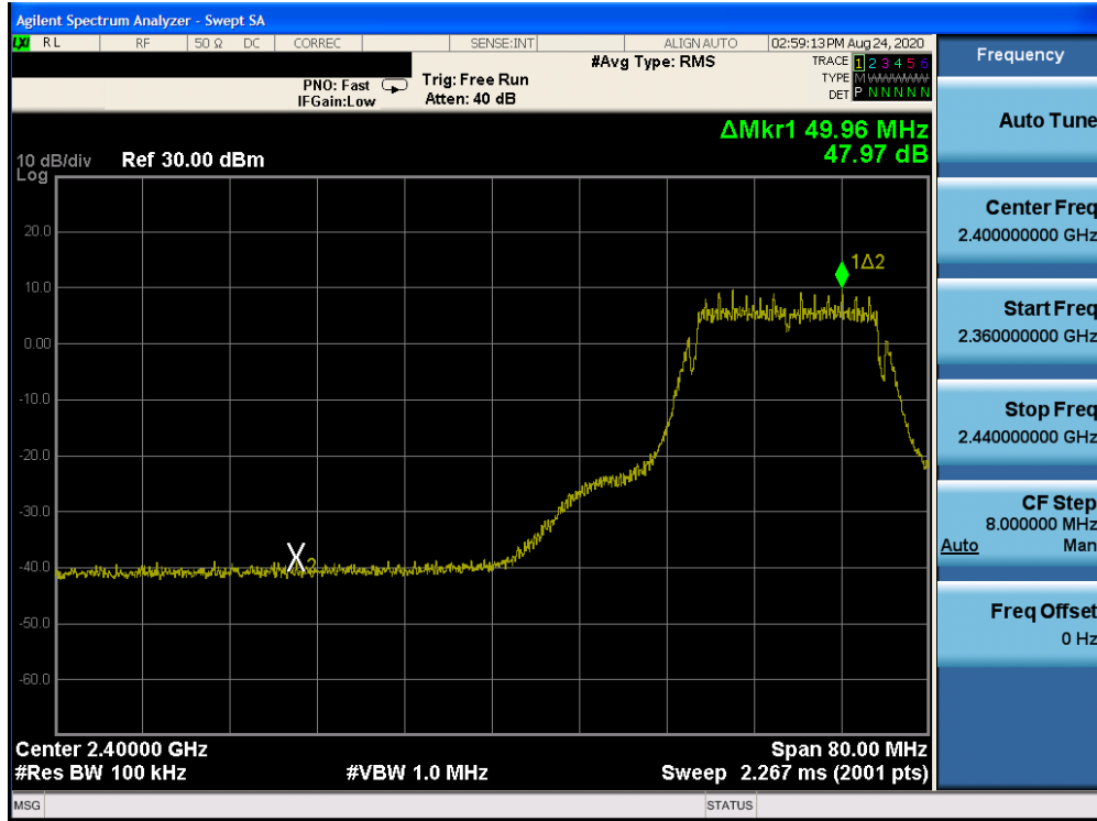
Plot 7-29: Band Edge Plot (802.11g– Ch. 4)
