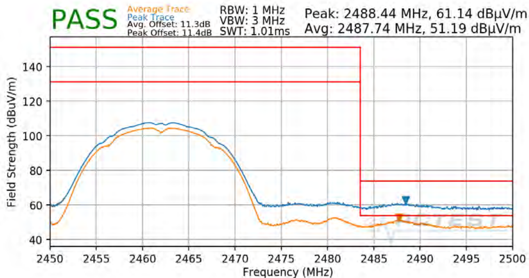
Plot 7-62: Radiated Restricted Upper Band Edge Measurement
