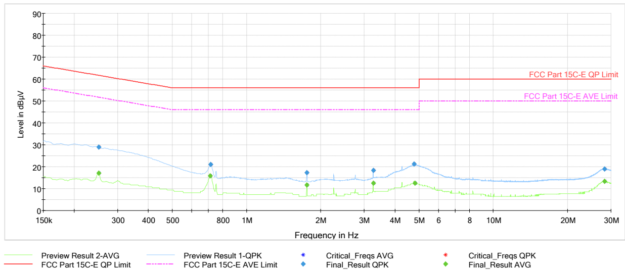
Plot 7-77. AC Line Conducted Emission with 802.11b (L1 with AC/DC Adapter)
