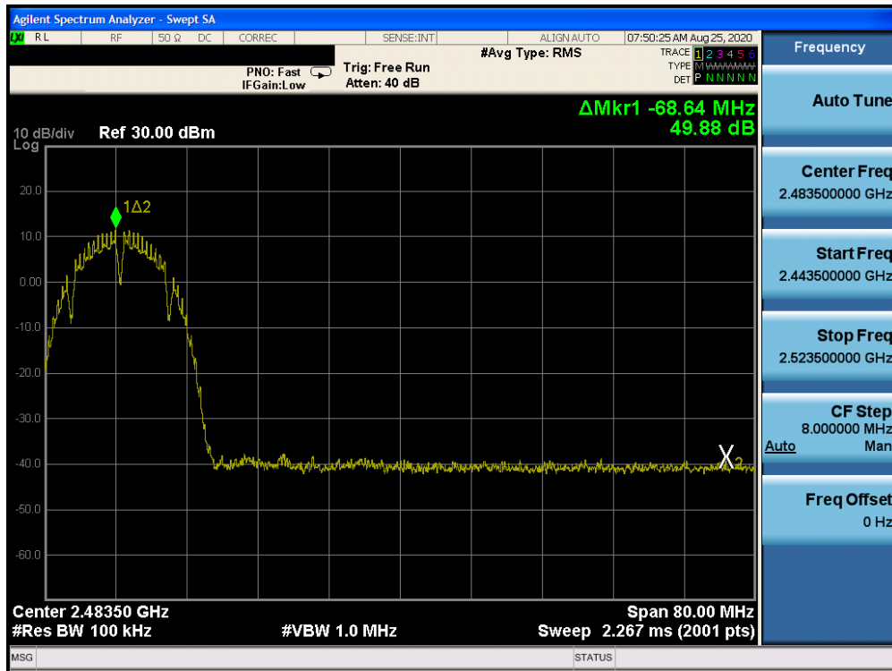
Plot 7-21: Band Edge Plot (802.11b – Ch.9)
