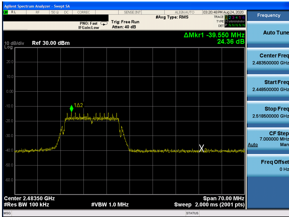
Plot 7-36: Band Edge Plot (802.11g– Ch. 13)
