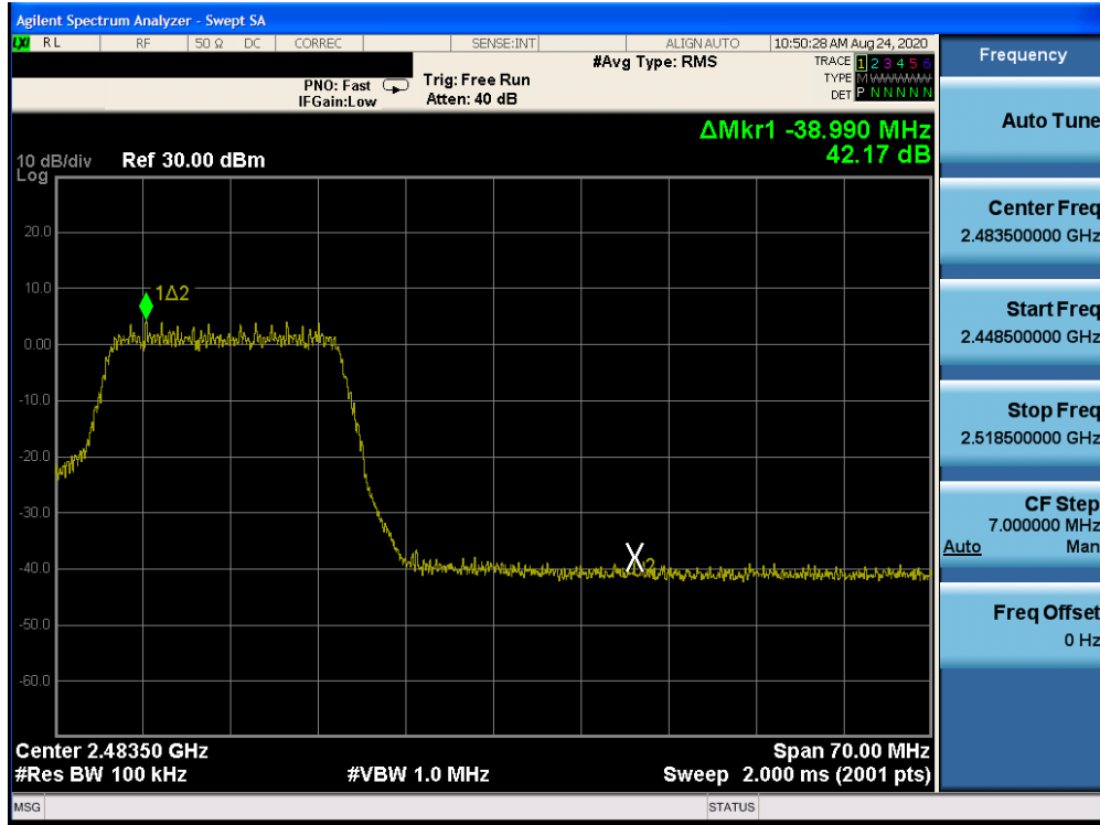
Plot 7-45: Band Edge Plot (802.11n (2.4GHz) – Ch. 11)
