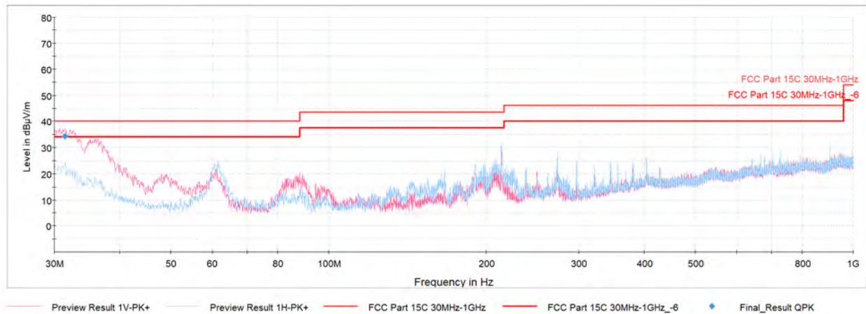
Plot 7-76. Radiated Spurious Emissions 30MHz-1GHz (802.11b – Ch 1)
