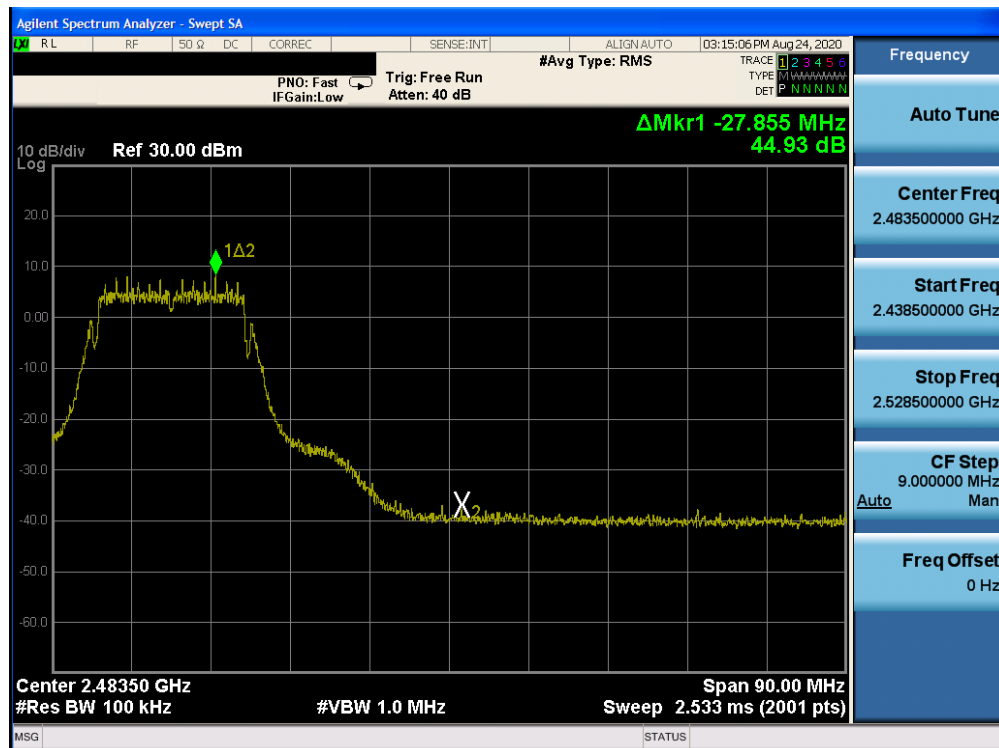
Plot 7-32: Band Edge Plot (802.11g– Ch. 9)
