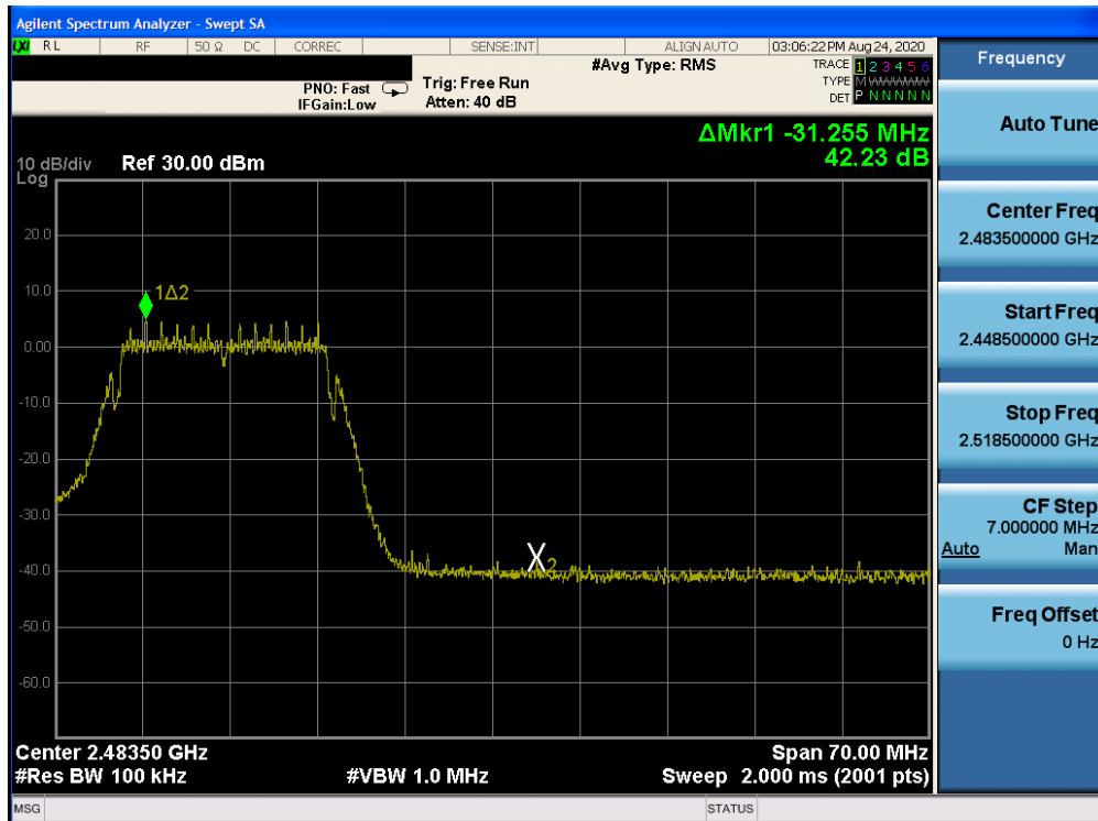
Plot 7-34: Band Edge Plot (802.11g– Ch. 11)
