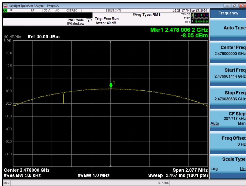
Plot 7-18. Power Spectral Density Plot (Bluetooth (LE), 2Mbps, iPA – Ch. 38)
