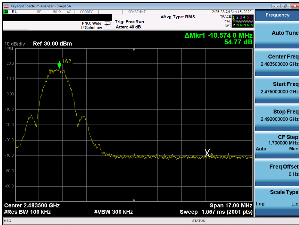
Plot 7-22. Band Edge Plot (Bluetooth (LE), 2Mbps, ePA – Ch. 38)
