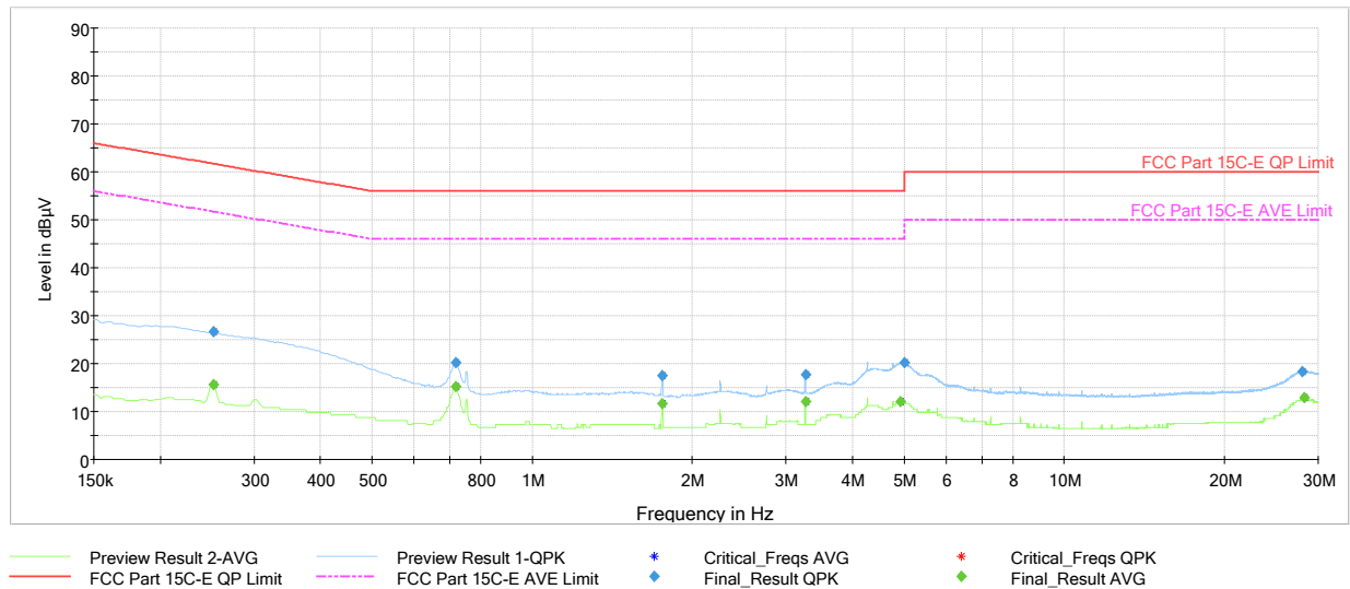
Plot 7-39. AC Line Conducted Emission with Bluetooth LE (L1 - 1Mbps, ePA, Ch.0, with AC/DC Adapter)
