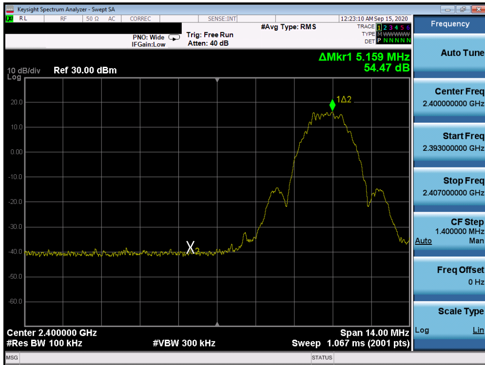
Plot 7-21. Band Edge Plot (Bluetooth (LE), 2Mbps, ePA – Ch. 1)
