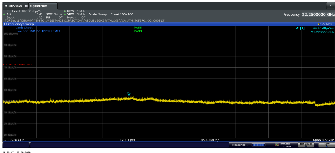
Plot 7-32. Radiated Spurious Emissions 18-26.5GHz (1Mbps, ePA – Ch.0, Pol. H)
