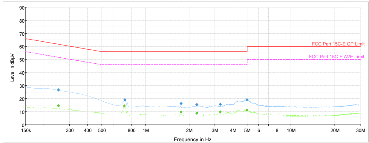
Plot 7-40. AC Line Conducted Emission with Bluetooth LE (N - 1Mbps, ePA, Ch.0, with AC/DC Adapter)
