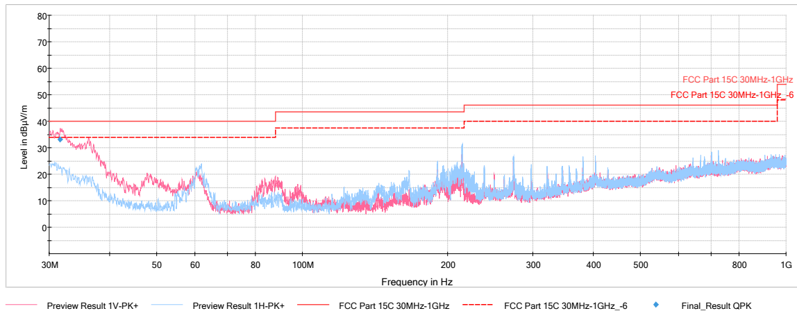
Plot 7-38. Radiated Spurious Emissions 30MHz-1GHz (1Mbps, ePA – Ch.0, with AC/DC Adapter)
