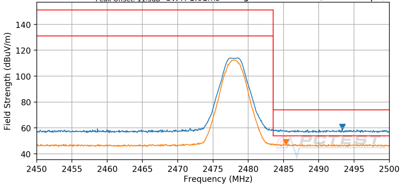
Plot 7-37. Radiated Restricted Upper Band Edge Measurement
