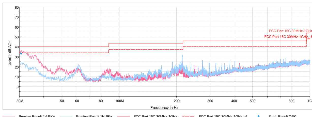
Plot 7-38. Radiated Spurious Emissions 30MHz-1GHz (4Mbps, ePA – Ch.1, with AC/DC Adapter)
