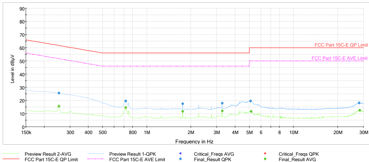
Plot 7-39. AC Line Conducted Emission with Bluetooth HDR (L1 – 4Mbps, ePA, Ch.1, with AC/DC Adapter)
