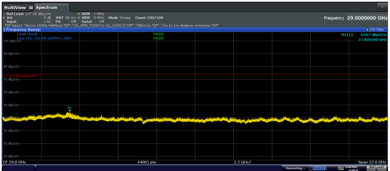
Plot 7-44: Radiated Spurious Emissions – Simultaneous Transmission 18GHz – 40GHz Pol H
