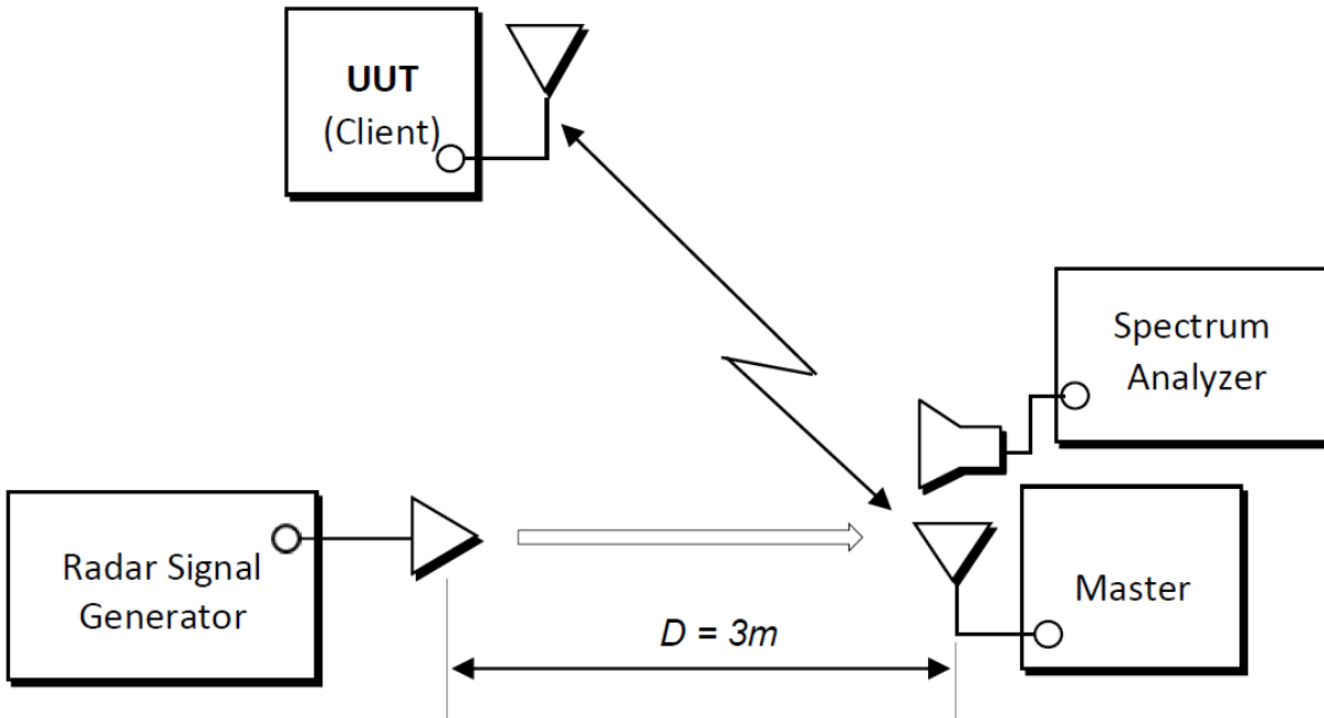
Figure 7-1. Radiated Test Setup for DFS
