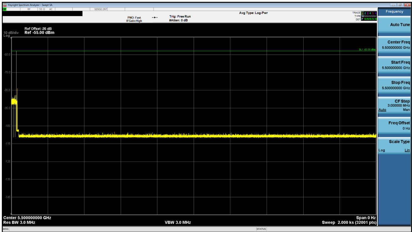
Figure 9-12: 5500MHz - Non-Occupancy Period (30 Minutes) – Mode 3 (20MHz)
