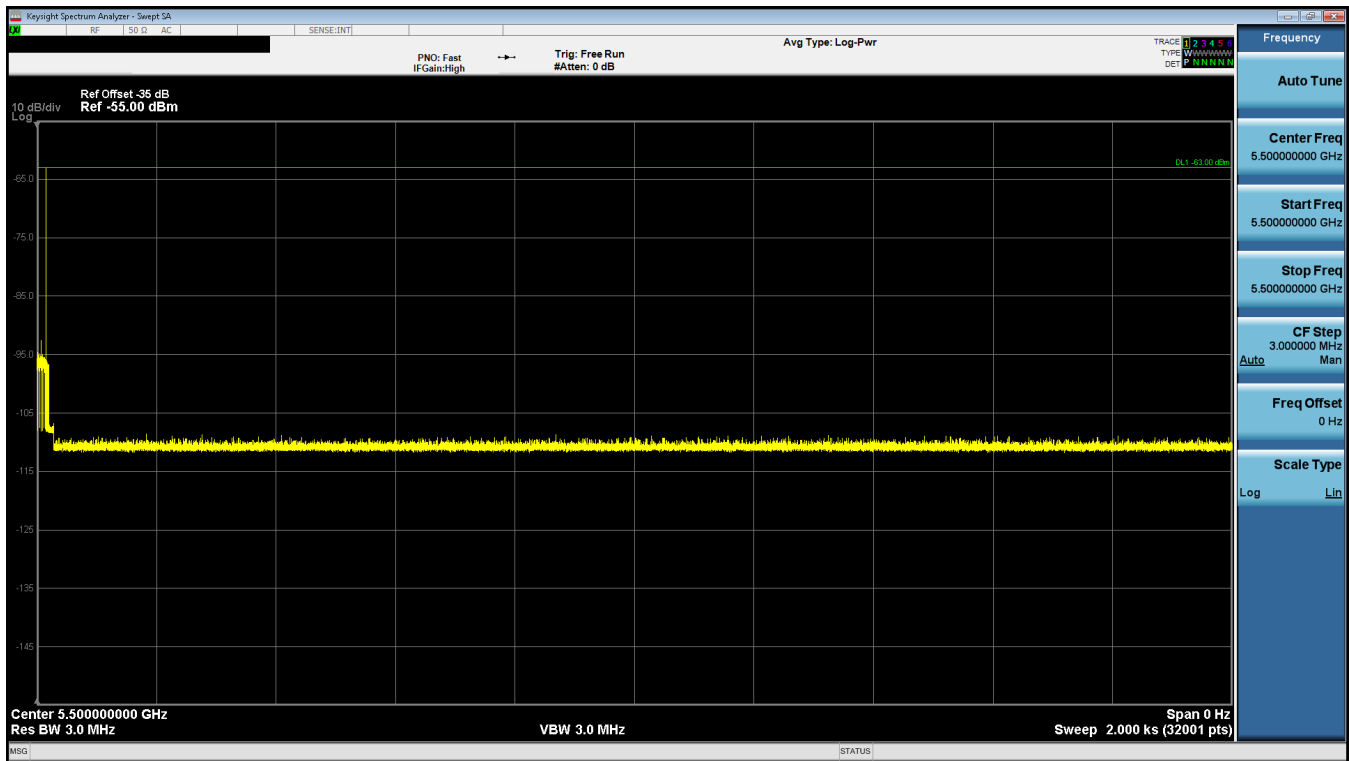
Figure 9-11: 5500MHz - Non-Occupancy Period (30 Minutes) – Mode 2 (20MHz)
