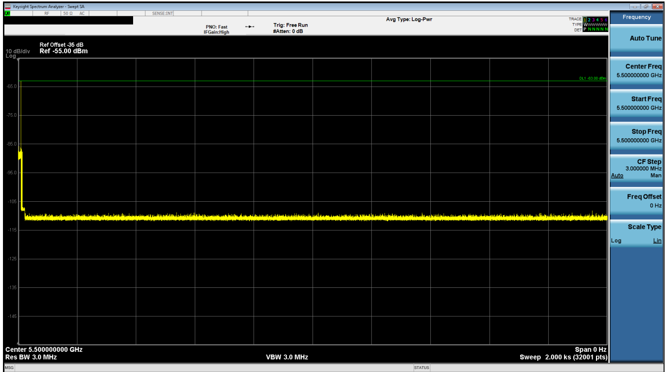
Figure 9-10. 5500MHz - Non-Occupancy Period (30 Minutes) – Mode 1 (20MHz)
