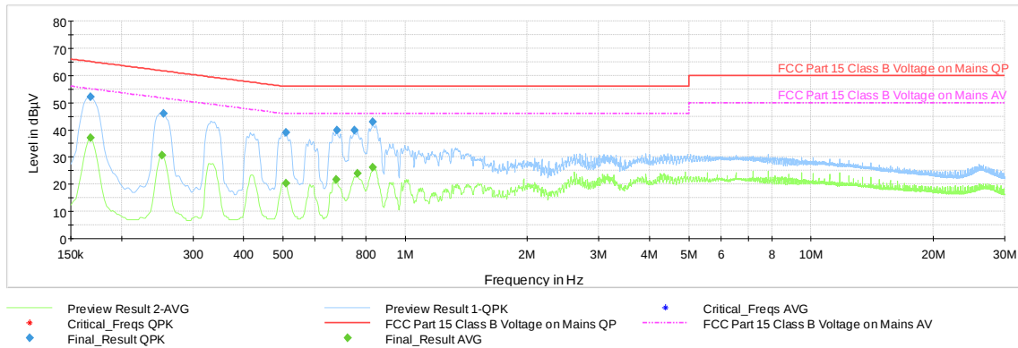
Plot 7-39. AC Line Conducted Emission with GFSK ePA Ch.39 (L1, with WCP + AC/DC Adapter)
