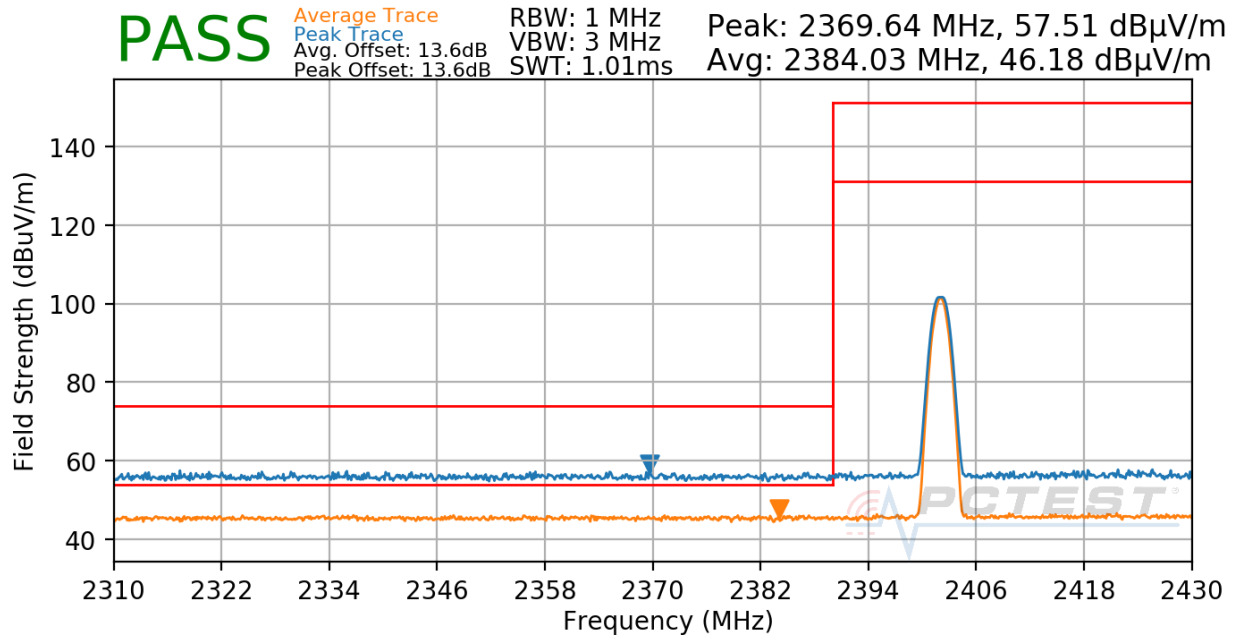
Plot 7-34. Radiated Restricted Lower Band Edge Measurement
