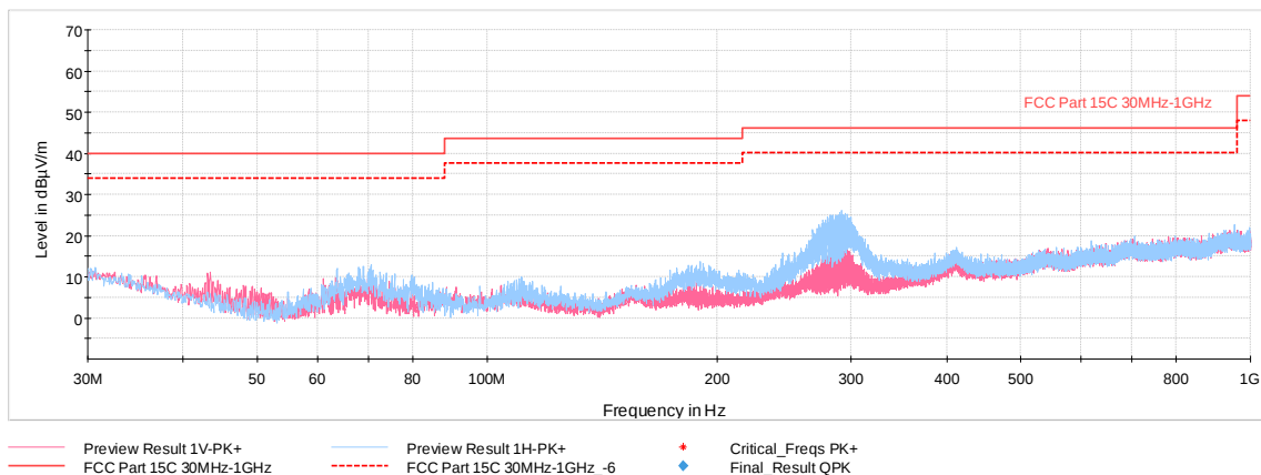
Plot 7-38. Radiated Spurious Emissions 30MHz-1GHz (GFSK ePA – Ch.39, with WCP + AC/DC adapter)
