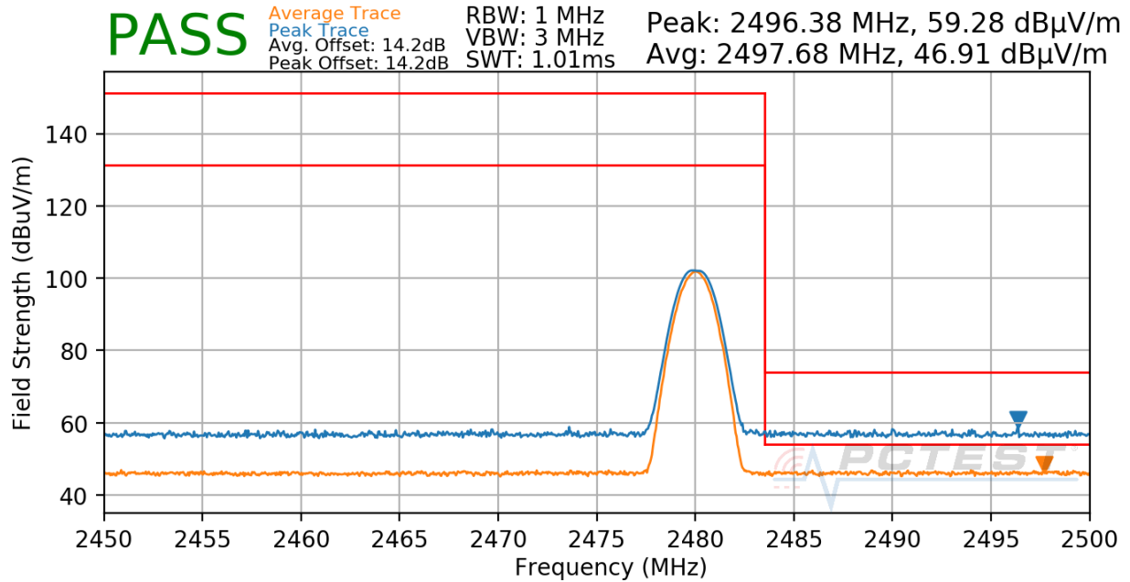
Plot 7-36. Radiated Restricted Upper Band Edge Measurement
