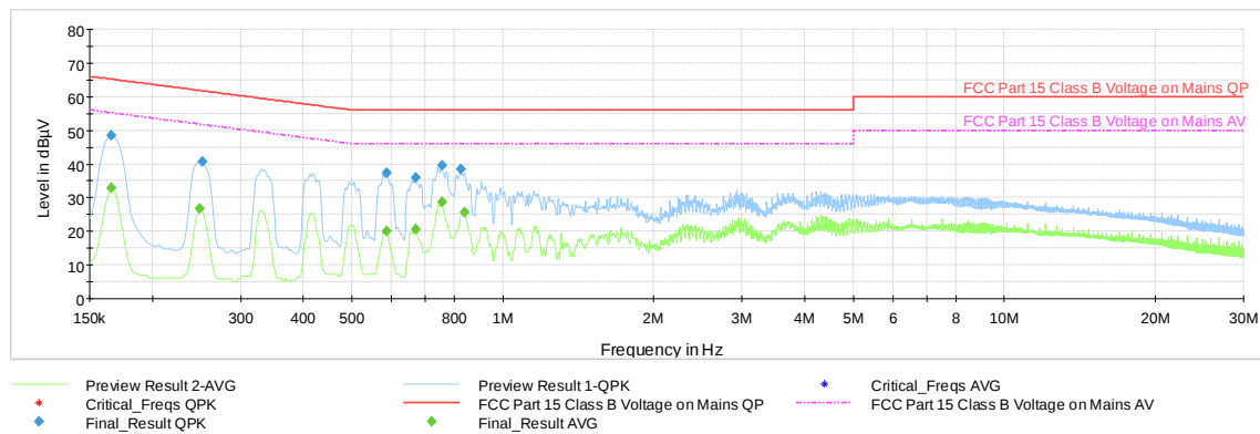
Plot 7-40. AC Line Conducted Emission with GFSK ePA Ch.39 (N, with WCP + AC/DC Adapter)
