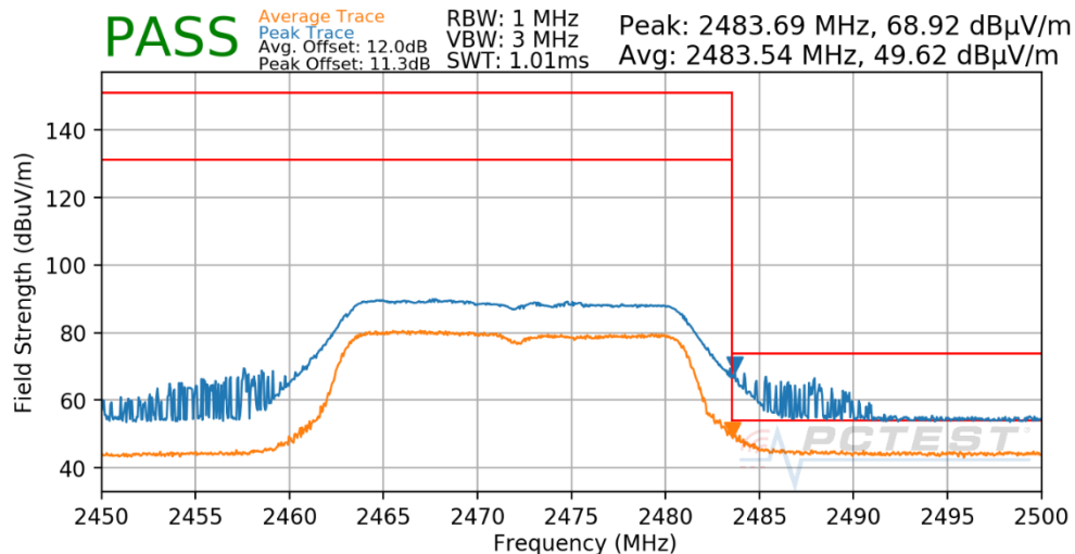
Plot 7-56. Radiated Restricted Upper Band Edge Measurement
