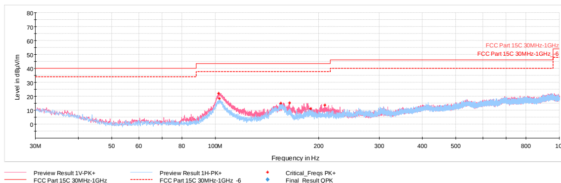
Plot 7-58. Radiated Spurious Emissions 30MHz-1GHz (Simultaneous Transmission, with WCP + laptop)
