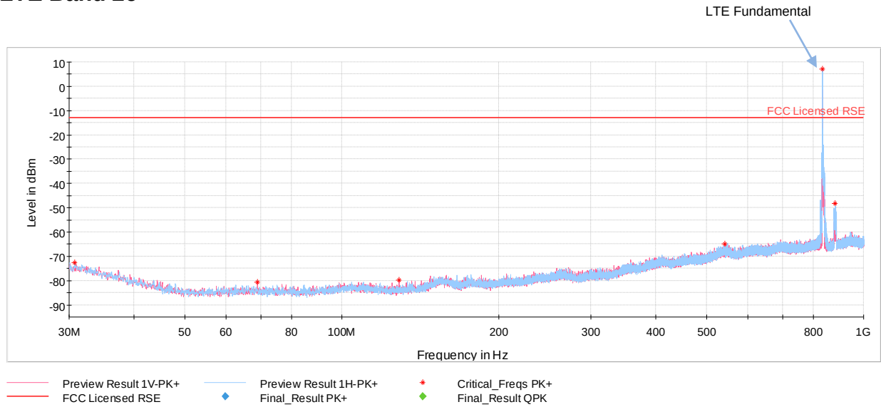
Plot 7-22. Radiated Spurious Emissions Below 1GHz (Band 26)
