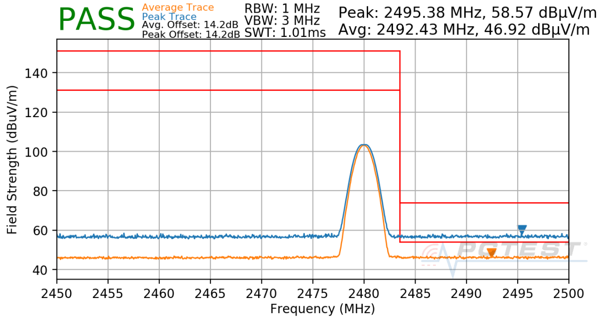
Plot 7-39. Radiated Restricted Upper Band Edge Measurement
