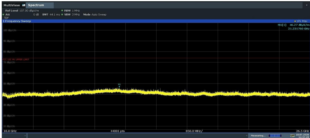
Plot 7-33. Radiated Spurious Emissions 18-26.5GHz (BT GFSK ePA – Ch.78, Pol. V)
