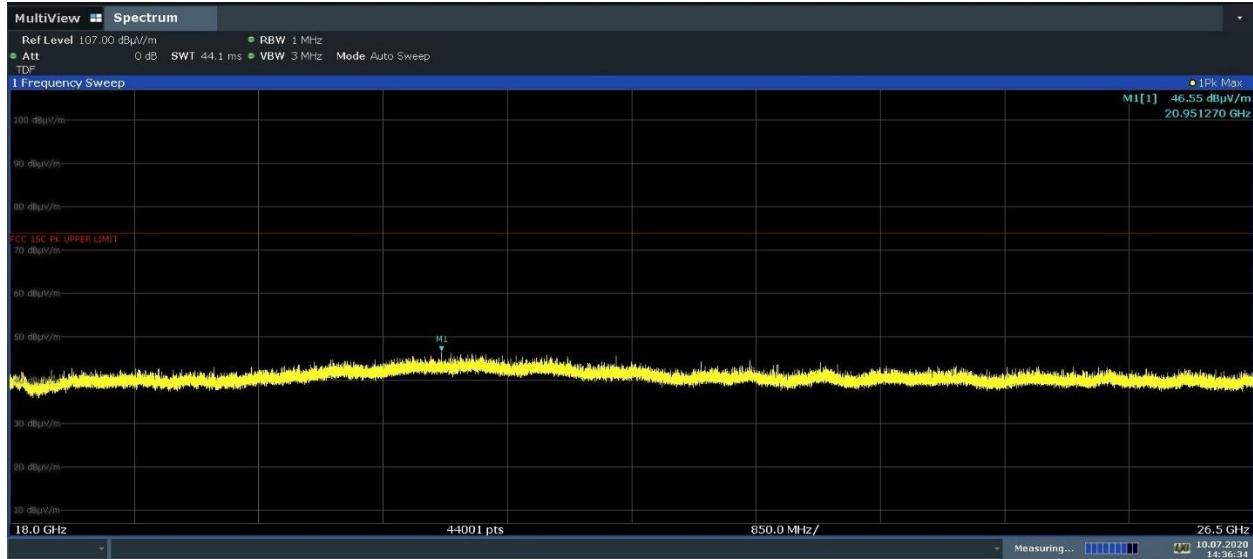
Plot 7-32. Radiated Spurious Emissions 18-26.5GHz (BT GFSK ePA – Ch.78, Pol. H)
