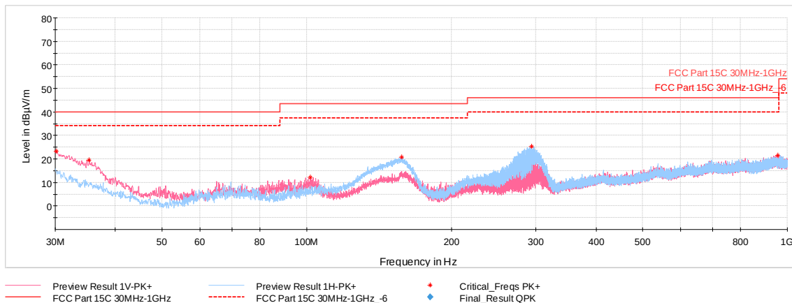
Plot 7-41. Radiated Spurious Emissions 30MHz-1GHz (GFSK ePA – Ch.78, with WCP + AC/DC adapter)
