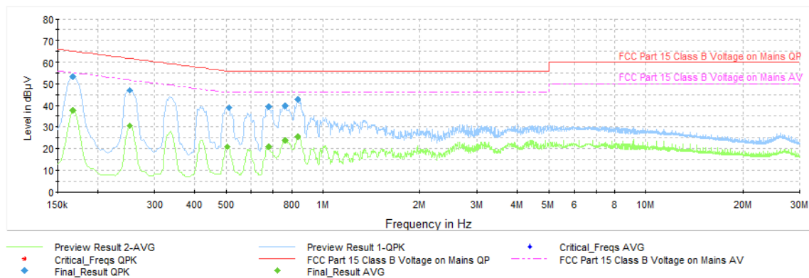
Plot 7-43. AC Line Conducted Emission with GFSK ePA Ch.78 (L1, with WCP + AC/DC Adapter)
