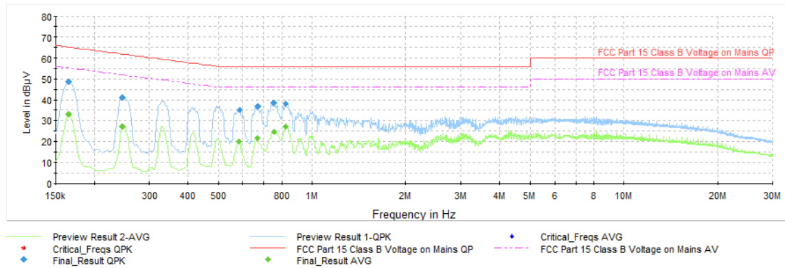
Plot 7-44. AC Line Conducted Emission with GFSK ePA Ch.78 (N, with WCP + AC/DC Adapter)
