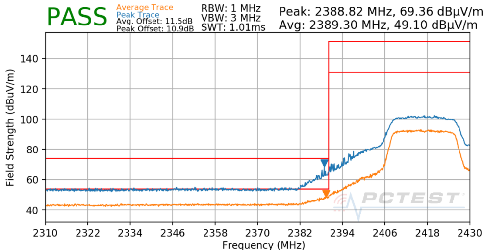
Plot 7-49. Radiated Restricted Lower Band Edge Measurement
