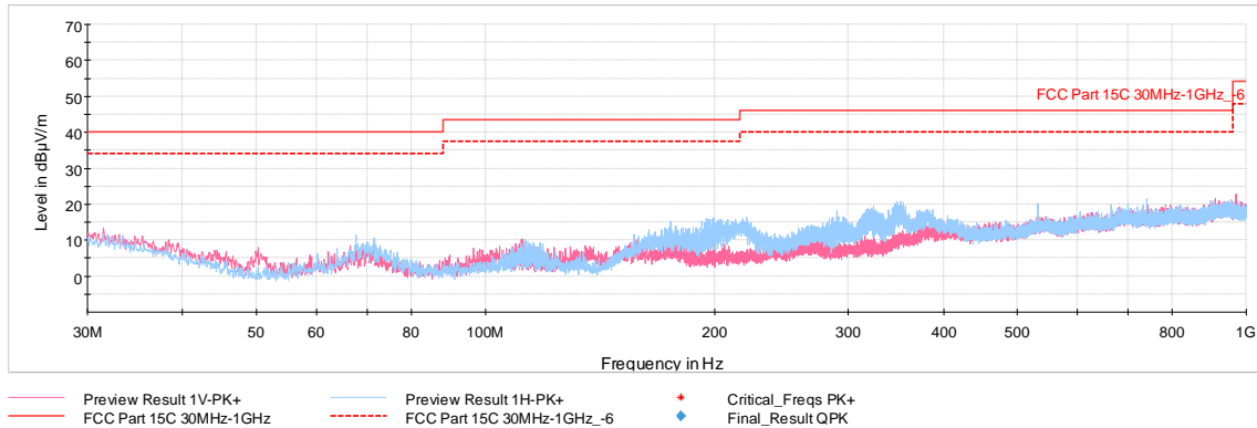
Plot 7-54. Radiated Spurious Emissions 30MHz-1GHz (802.11b – Ch.6, with WCP + laptop)
