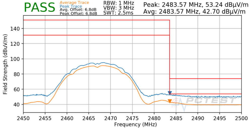
Plot 7-46. Radiated Restricted Upper Band Edge Measurement
