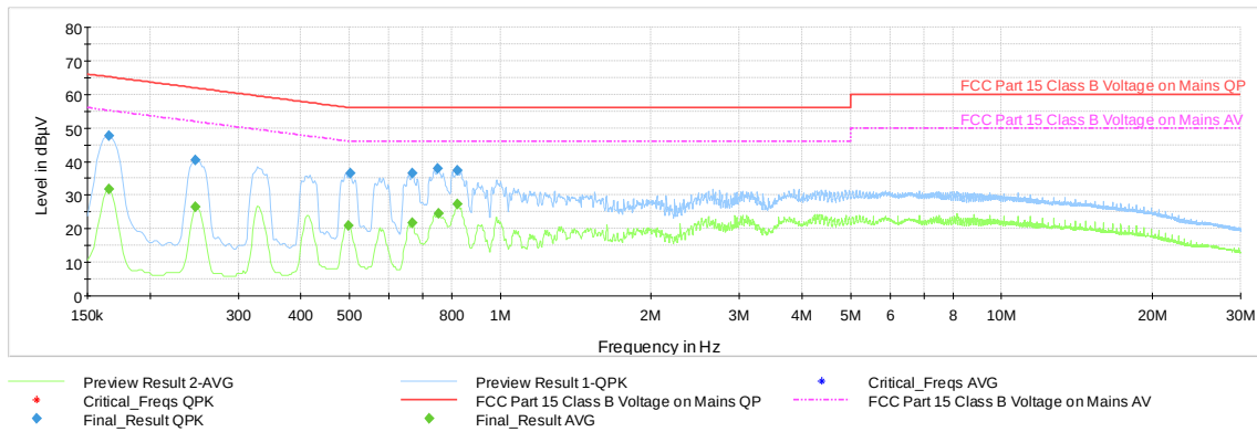
Plot 7-40. AC Line Conducted Emission with Bluetooth LE (N - 1Mbps, ePA, Ch.39, with WCP + AC/DC Adapter)
