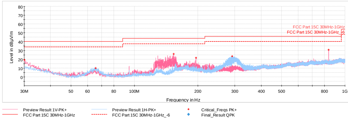
Plot 7-38. Radiated Spurious Emissions 30MHz-1GHz (1Mbps, ePA – Ch.39, with WCP + laptop)
