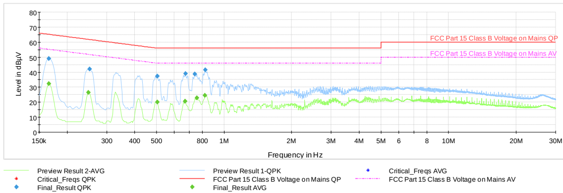
Plot 7-39. AC Line Conducted Emission with Bluetooth LE (L1 - 1Mbps, ePA, Ch.39, with WCP + AC/DC Adapter)
