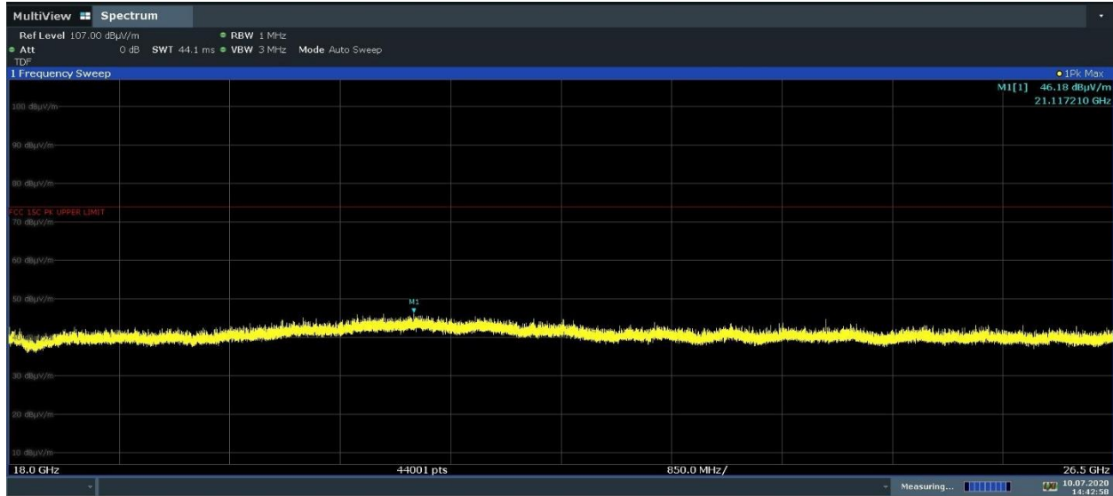
Plot 7-32. Radiated Spurious Emissions 18-26.5GHz (1Mbps, ePA – Ch.39, Pol. H)
