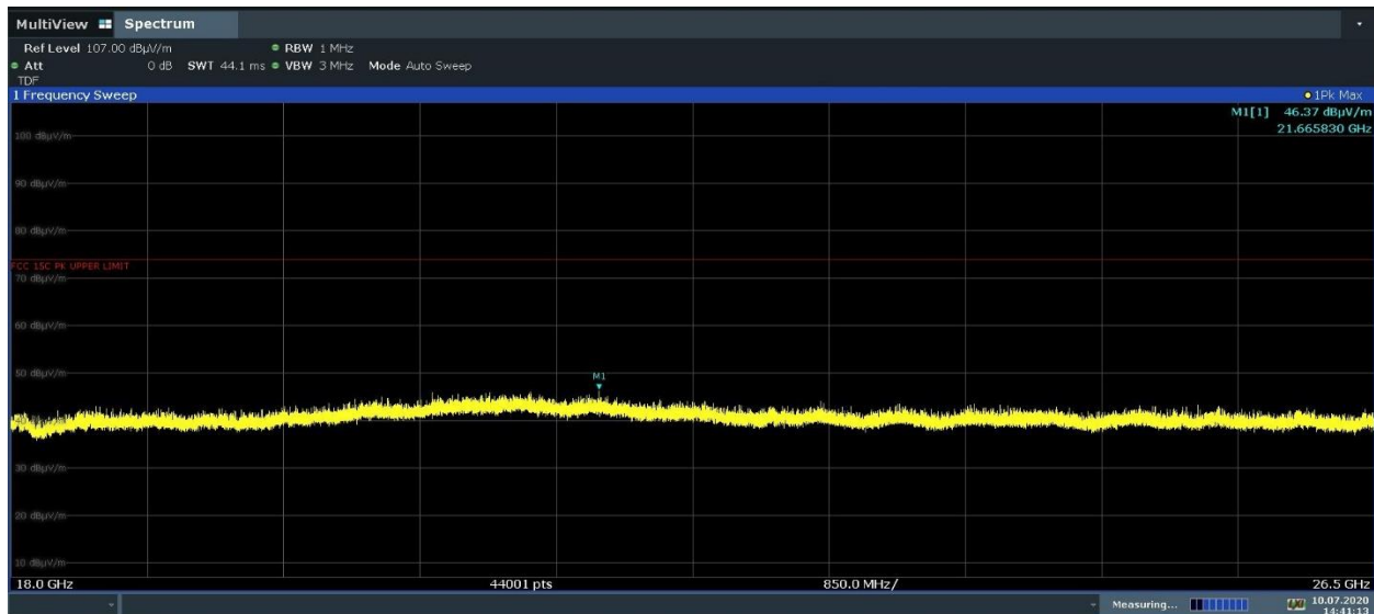
Plot 7-33. Radiated Spurious Emissions 18-26.5GHz (1Mbps, ePA – Ch.39, Pol. V)
