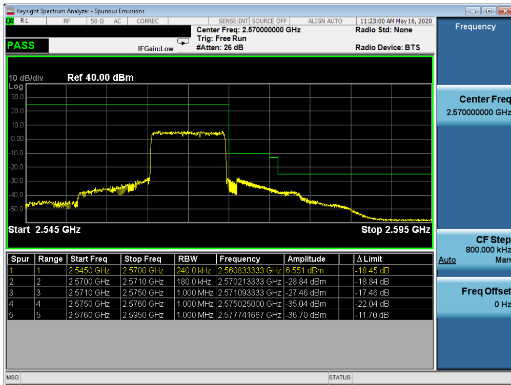
Plot 7-259. Upper ACP Plot (Band 7 - 10.0MHz QPSK - Full RB Configuration)
