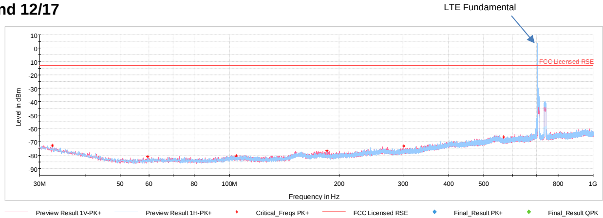
Plot 7-320. Radiated Spurious Emissions below 1GHz (Band 12/17)
