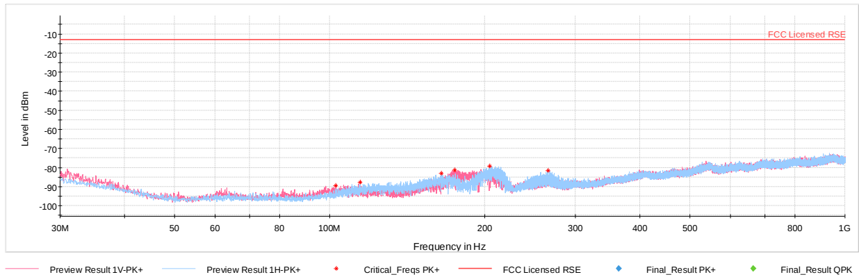
Plot 7-334. Radiated Spurious Emissions – Simultaneous Transmission 30MHz – 1GHz
