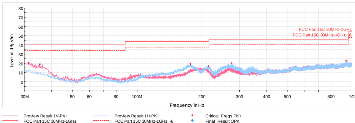
Plot 7-38. Radiated Spurious Emissions 30MHz-1GHz (4Mbps, ePA – Ch.38, with WCP + AC/DC adapter)
