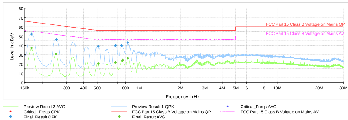
Plot 7-39. AC Line Conducted Emission with GFSK ePA Ch.78 (L1, with WCP + AC/DC Adapter)
