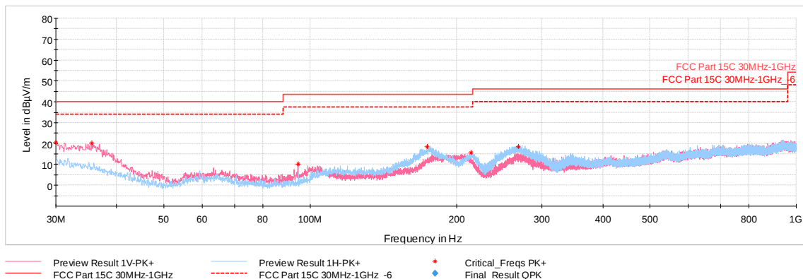
Plot 7-38. Radiated Spurious Emissions 30MHz-1GHz (GFSK ePA – Ch.78, with WCP + AC/DC adapter)
