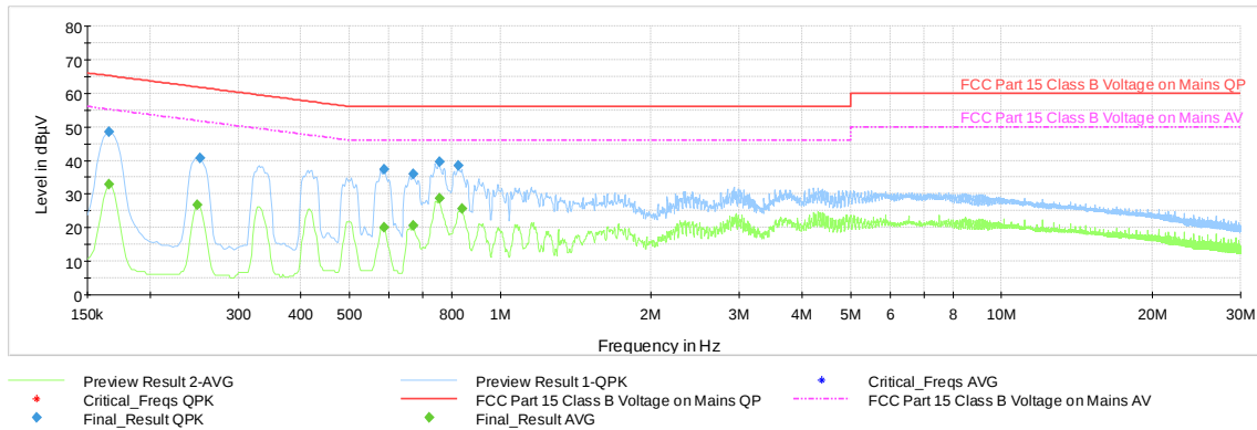
Plot 7-40. AC Line Conducted Emission with GFSK ePA Ch.78 (N, with WCP + AC/DC Adapter)
