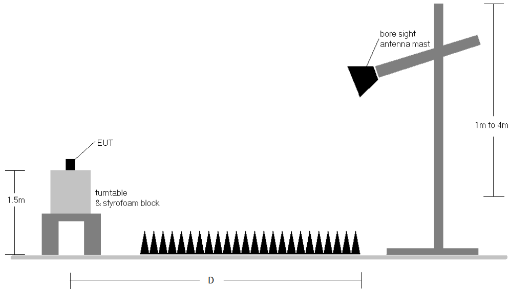
Figure 7-8. Radiated Measurement Setup >1GHz
