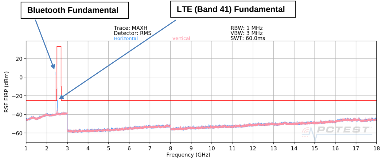
Plot 7-34. Radiated Spurious Emissions 1-18GHz (Simultaneous Transmission)
