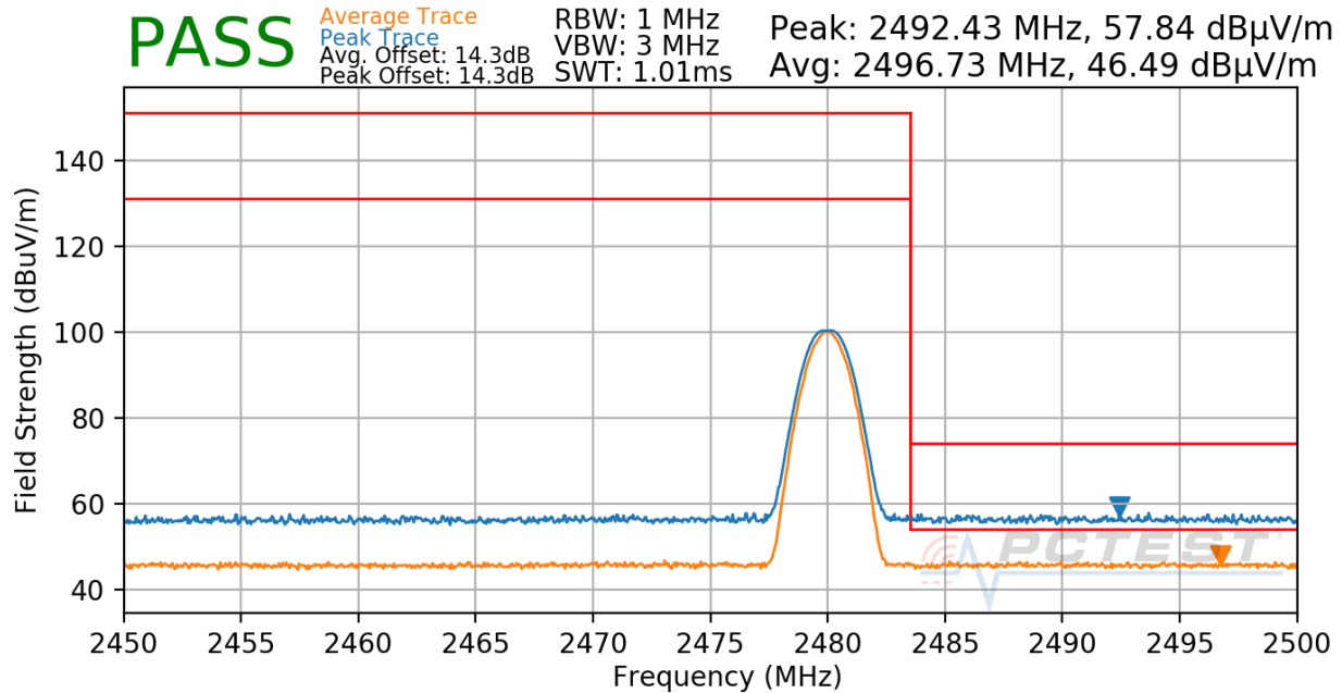
Plot 7-39. Radiated Restricted Upper Band Edge Measurement
