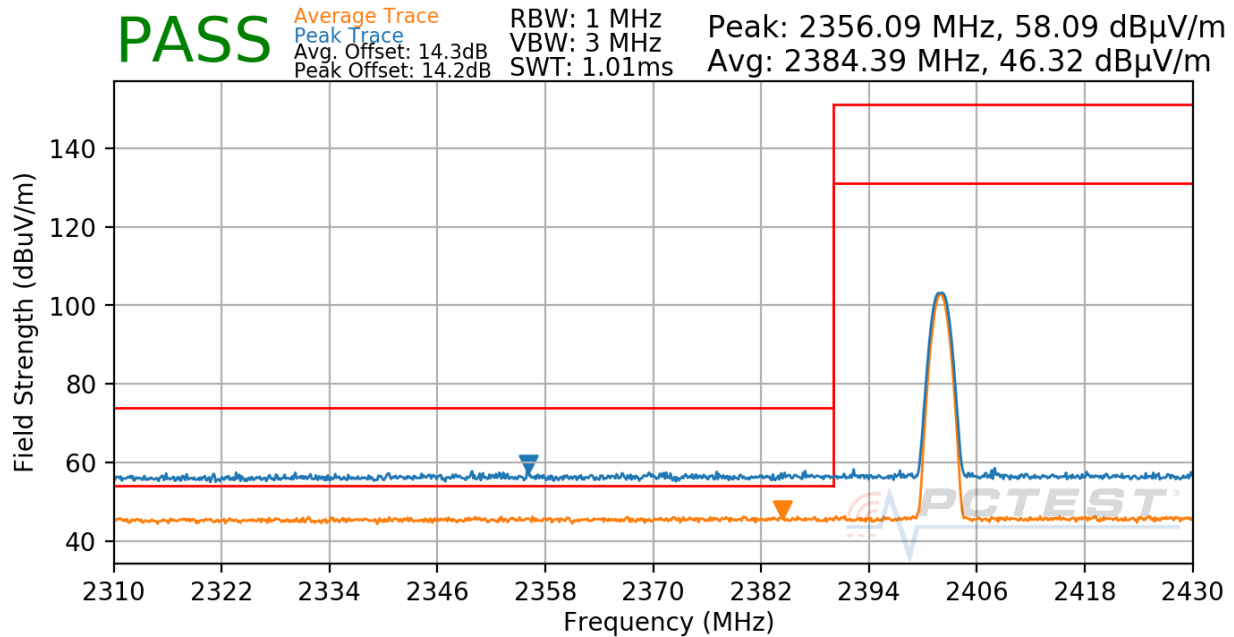
Plot 7-37. Radiated Restricted Lower Band Edge Measurement
