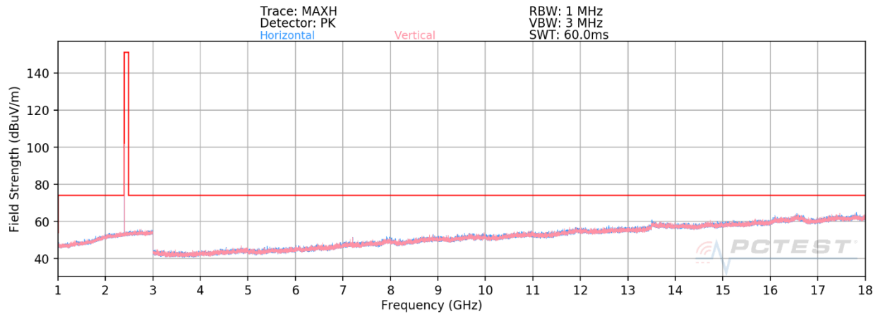
Plot 7-29. Radiated Spurious Emissions 1-18GHz (BT GFSK ePA – Ch. 0)
