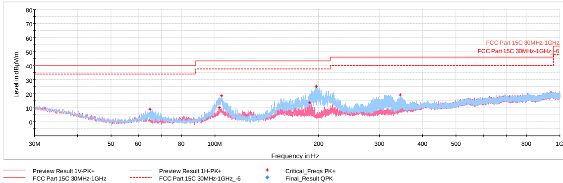
Plot 7-42. Radiated Spurious Emissions 30MHz-1GHz (Simultaneous Transmission, with WCP + Laptop)
