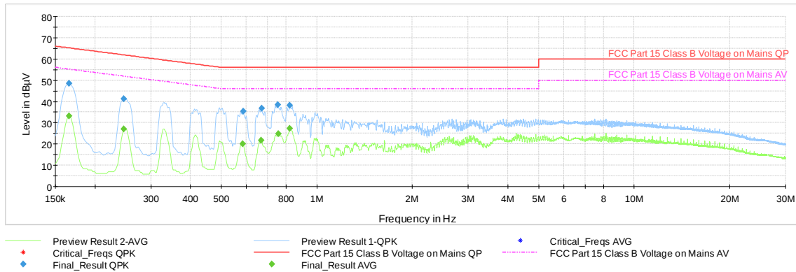
Plot 7-44. AC Line Conducted Emission with GFSK ePA Ch.39 (N, with WCP + AC/DC Adapter)
