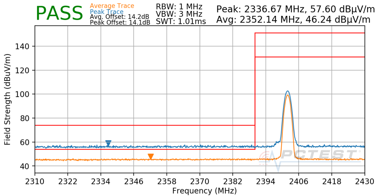
Plot 7-38. Radiated Restricted Lower Band Edge Measurement
