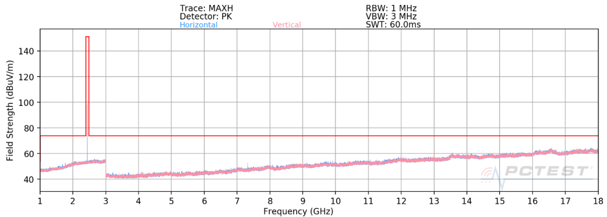
Plot 7-30. Radiated Spurious Emissions 1-18GHz (BT GFSK ePA – Ch. 39)
