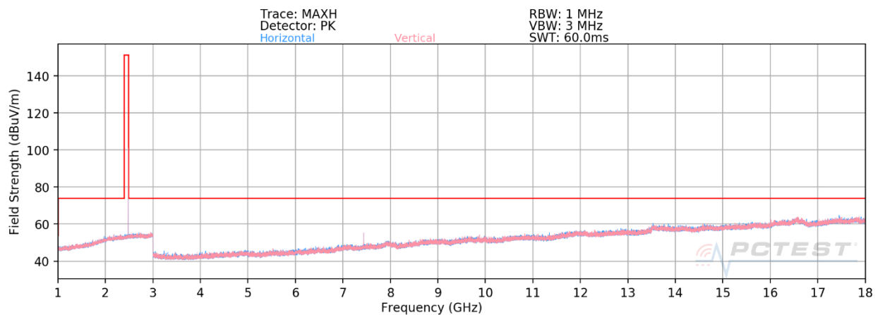
Plot 7-31. Radiated Spurious Emissions 1-18GHz (BT GFSK ePA – Ch. 78)
