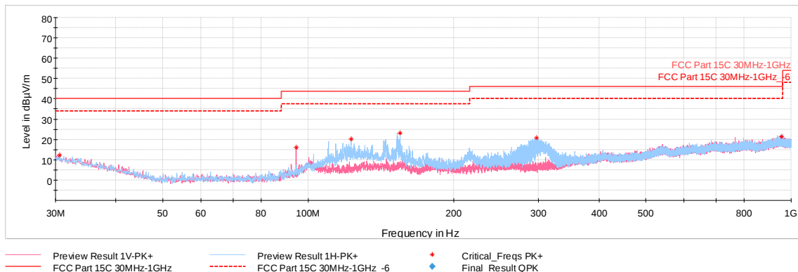
Plot 7-41. Radiated Spurious Emissions 30MHz-1GHz (GFSK ePA – Ch.39, with WCP + Laptop)
