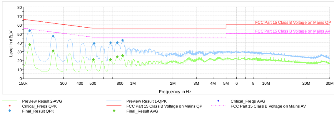
Plot 7-43. AC Line Conducted Emission with GFSK ePA Ch.39 (L1, with WCP + AC/DC Adapter)
