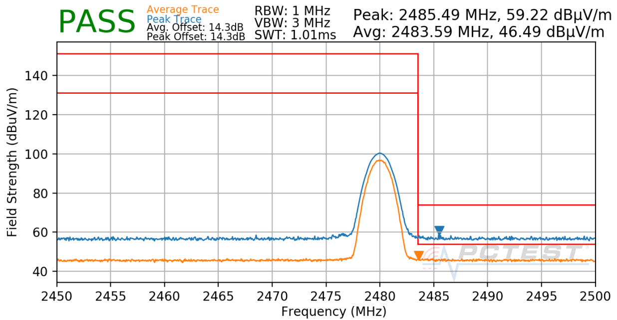
Plot 7-40. Radiated Restricted Upper Band Edge Measurement
