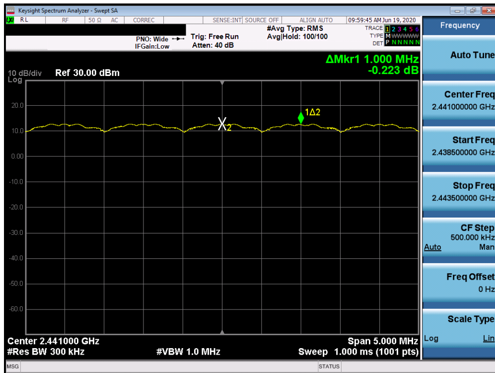
Plot 7-16. Channel Separation Plot (Bluetooth, 8DPSK, ePA)
