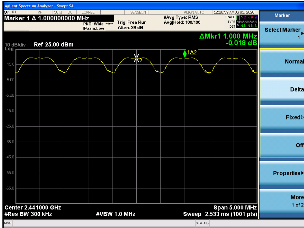
Plot 7-15. Channel Separation Plot (Bluetooth, GFSK, ePA)
