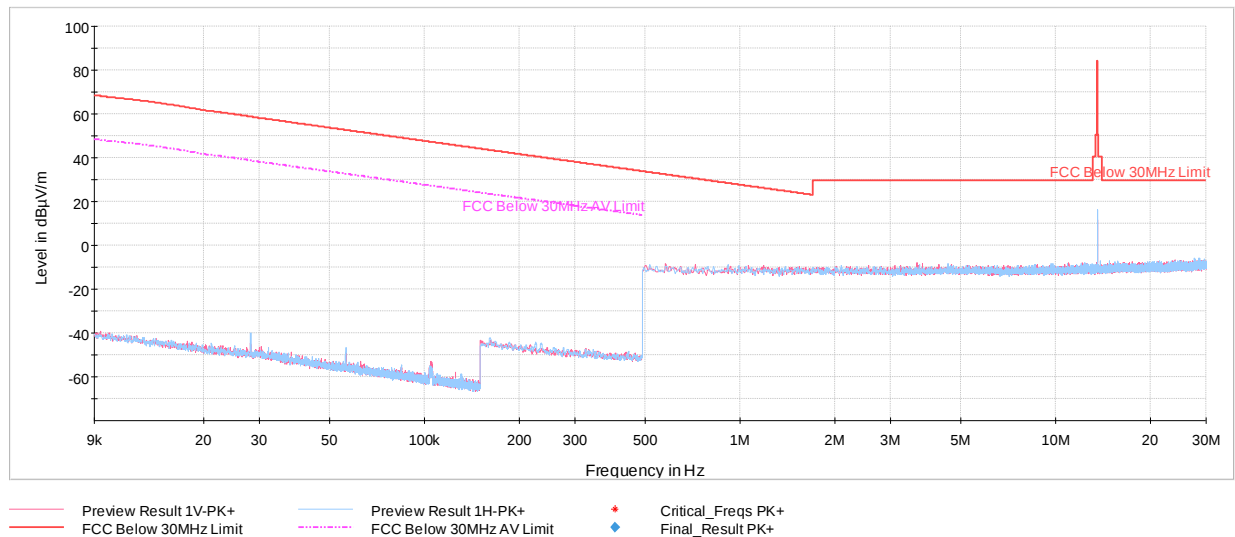
Plot 7-8. Radiated Spurious Emissions 9kHz – 30MHz (CE A 848kbps, with WCP + AC/DC Adapter)
