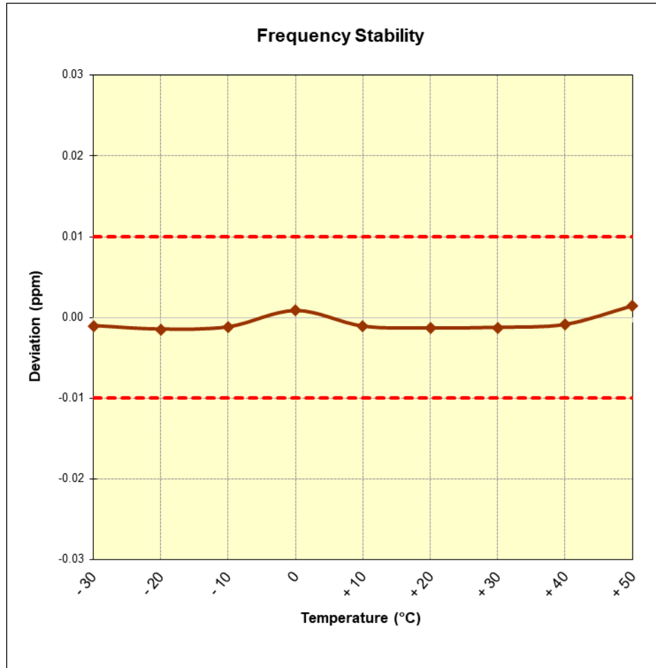
Figure 7-4. Frequency Stability Plot (Reader 10% Ask 1 out of 256)
