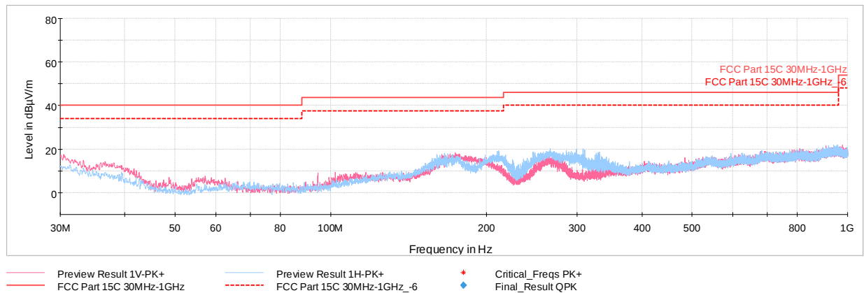
Plot 7-11. Radiated Spurious Emissions 30MHz – 1GHz (Reader 10% Ask 1 out of 256, with WCP + AC/DC Adapter)
