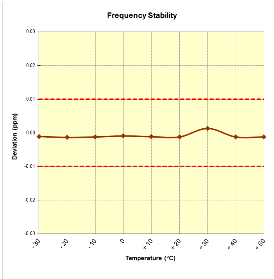
Figure 7-3. Frequency Stability Plot (CE A 848kbps)
