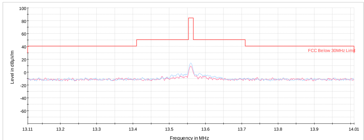
Plot 7-7. In Band Radiated Spurious Emissions (Reader 10% Ask 1 out of 256, with WCP + AC/DC Adapter)
