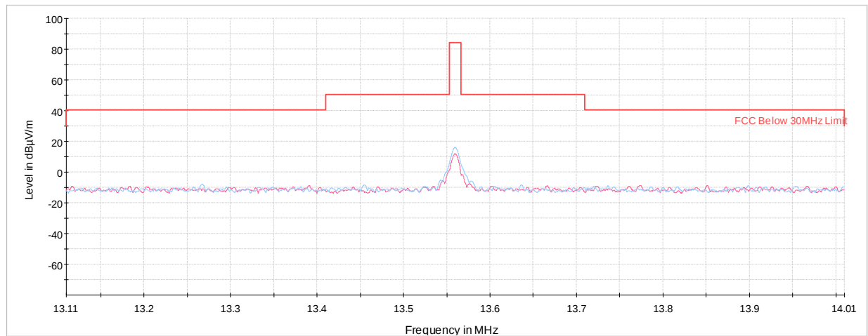
Plot 7-6. In Band Radiated Spurious Emissions (CE A 848kbps, with WCP + AC/DC Adapter)
