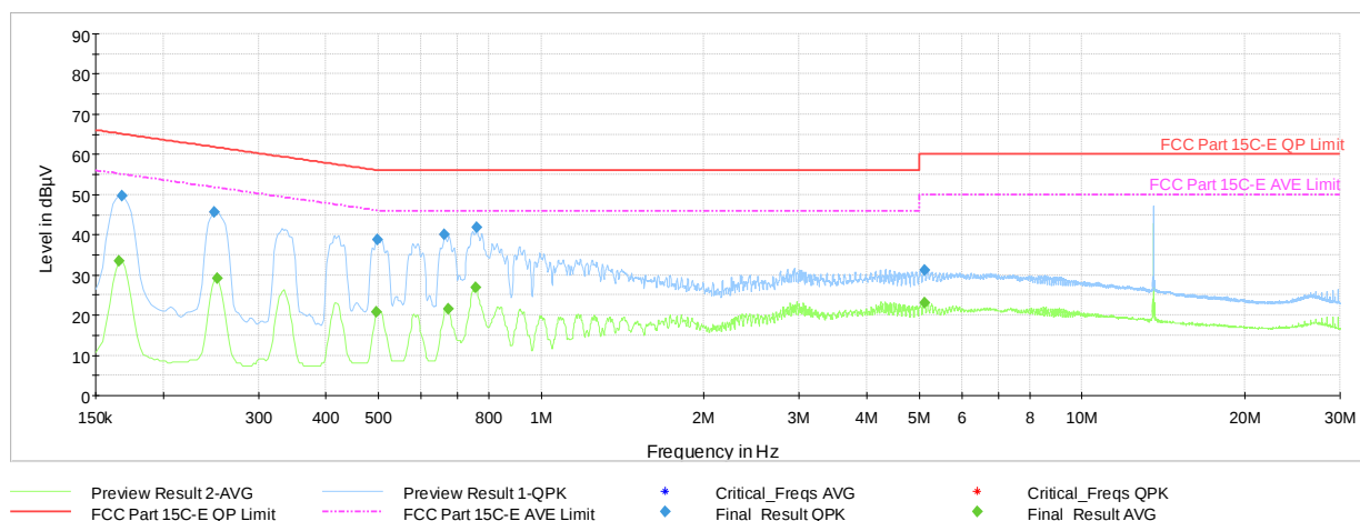
Plot 7-12. AC Line-Conducted Test Plot (L1, CE A 848kbps, with WCP + AC/DC Adapter)
