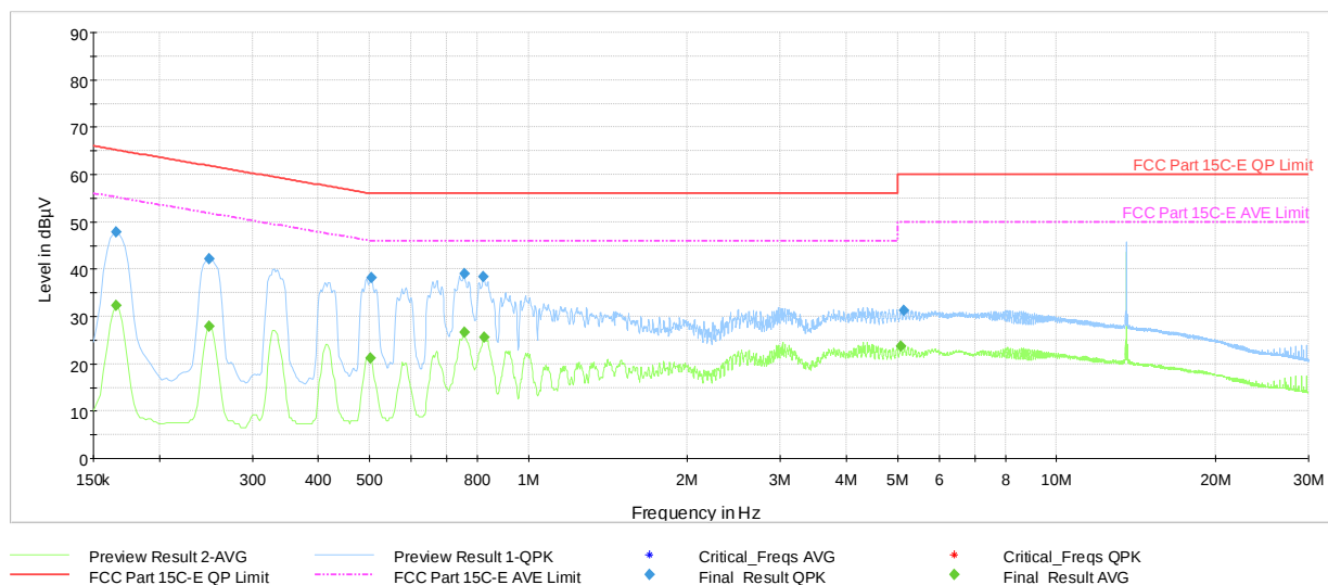
Plot 7-13. AC Line-Conducted Test Plot (N, CE A 848kbps, with WCP + AC/DC Adapter)
