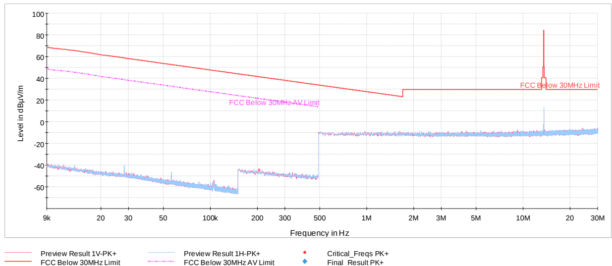
Plot 7-9. Radiated Spurious Emissions 9kHz – 30MHz (Reader 10% Ask 1 out of 256, with WCP + AC/DC Adapter)
