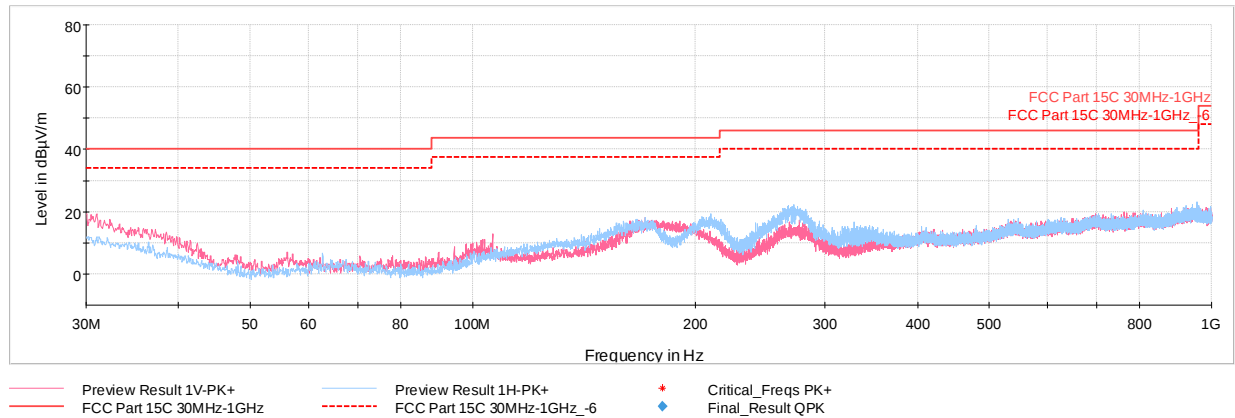
Plot 7-10. Radiated Spurious Emissions 30MHz – 1GHz (CE A 848kbps, with WCP + AC/DC Adapter)
