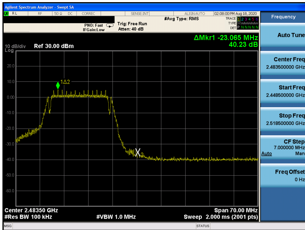
Plot 7-26. Band Edge Plot (802.11g - Ch. 12)
