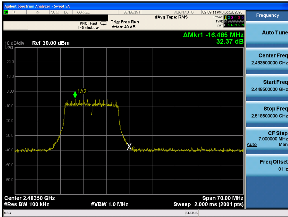
Plot 7-27. Band Edge Plot (802.11g – Ch. 13)
