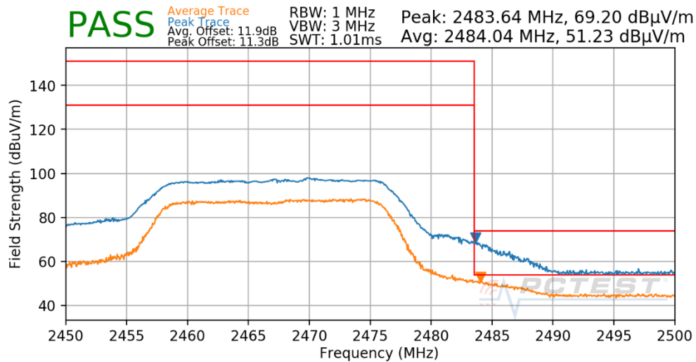
Plot 7-52. Radiated Restricted Upper Band Edge Measurement
