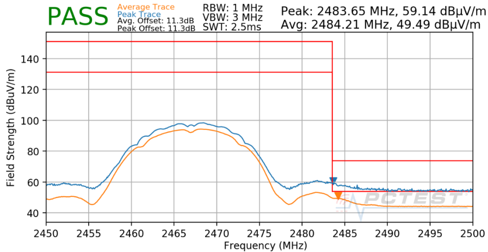
Plot 7-46. Radiated Restricted Upper Band Edge Measurement
