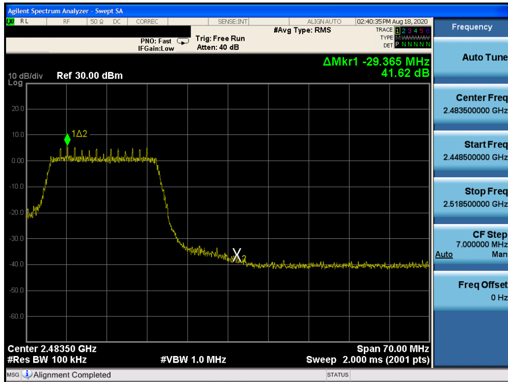
Plot 7-31. Band Edge Plot (802.11n (2.4GHz) – Ch. 11)
