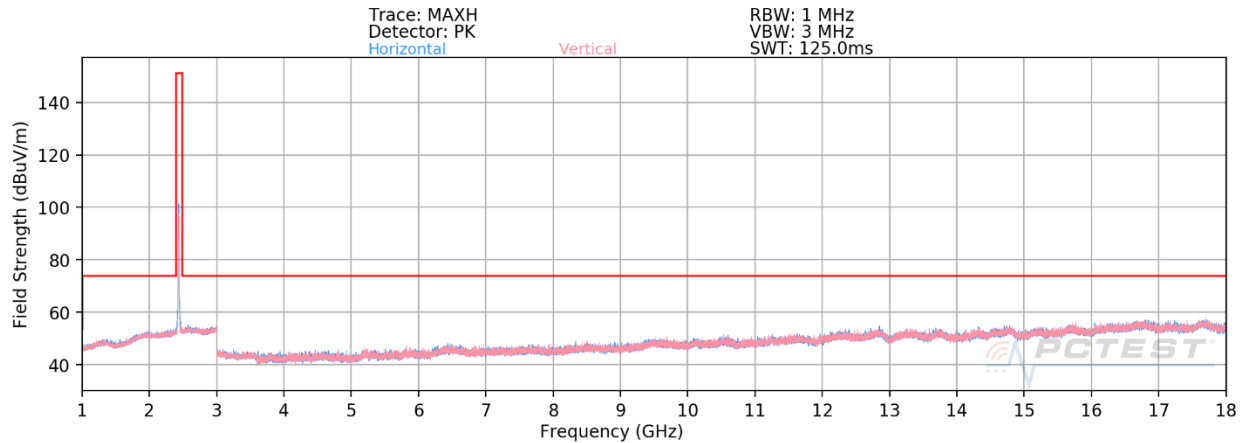
Plot 7-41. Radiated Spurious Emissions 1-18GHz (802.11b – Ch. 6)
