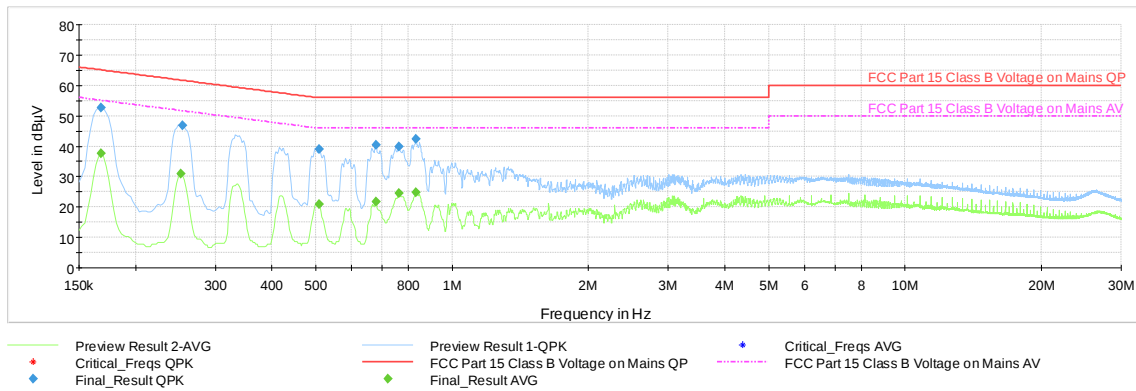
Plot 7-55. AC Line Conducted Emission with 802.11b Ch.6 (L1, with WCP + AC/DC Adapter)
