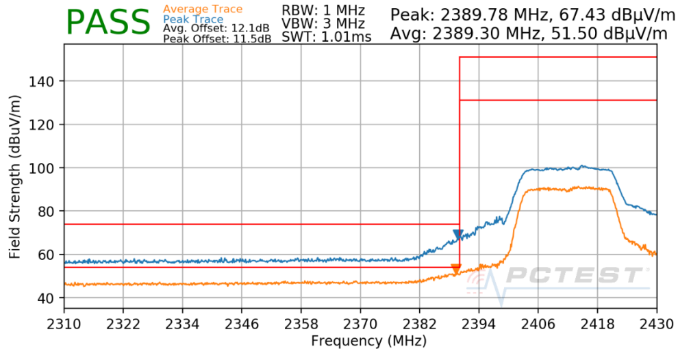
Plot 7-48. Radiated Restricted Lower Band Edge Measurement
