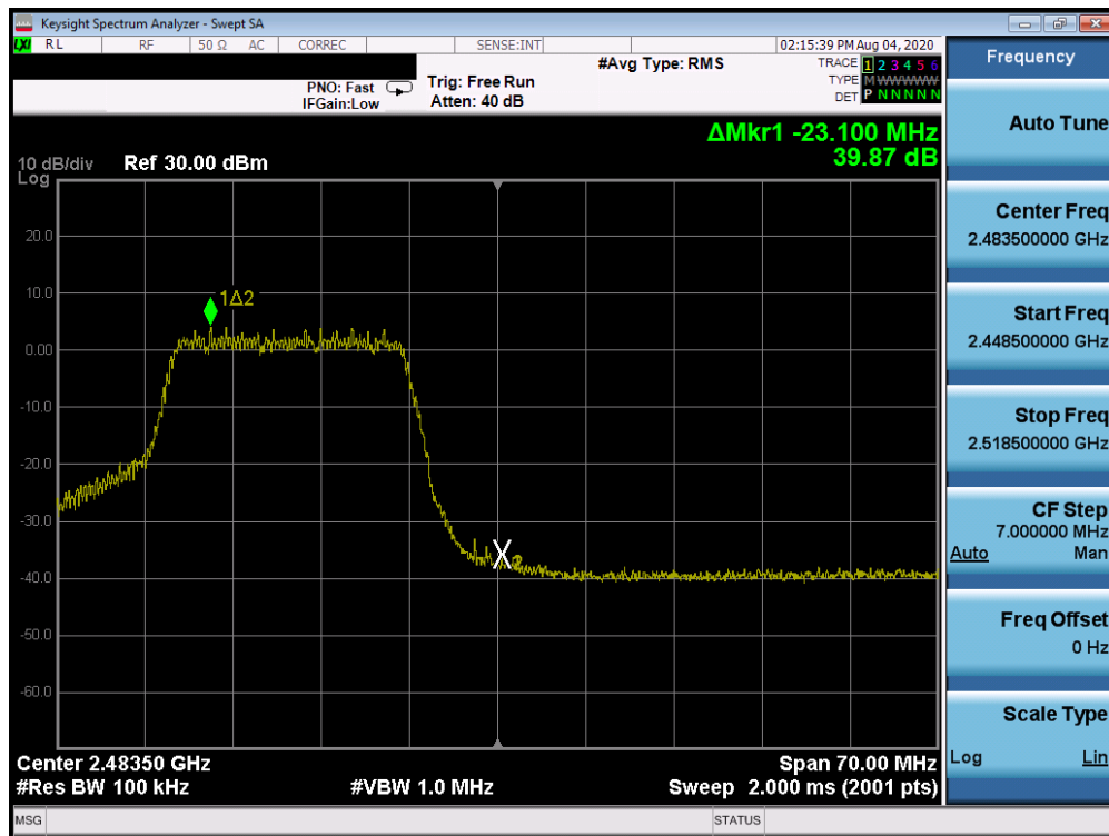
Plot 7-32. Band Edge Plot (802.11n (2.4GHz) – Ch. 12)
