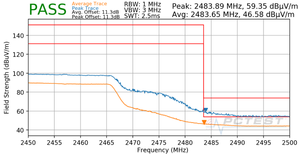
Plot 7-50. Radiated Restricted Upper Band Edge Measurement
