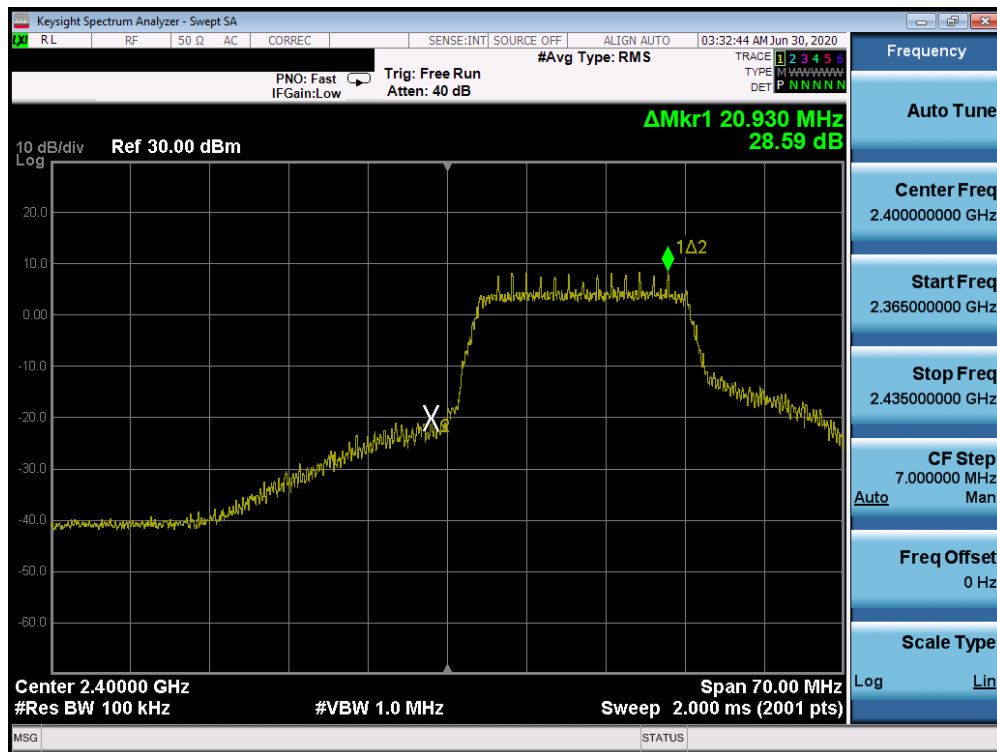
Plot 7-28. Band Edge Plot (802.11n (2.4GHz) – Ch. 1)
