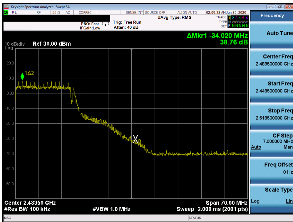
Plot 7-24. Band Edge Plot (802.11g– Ch. 10)
