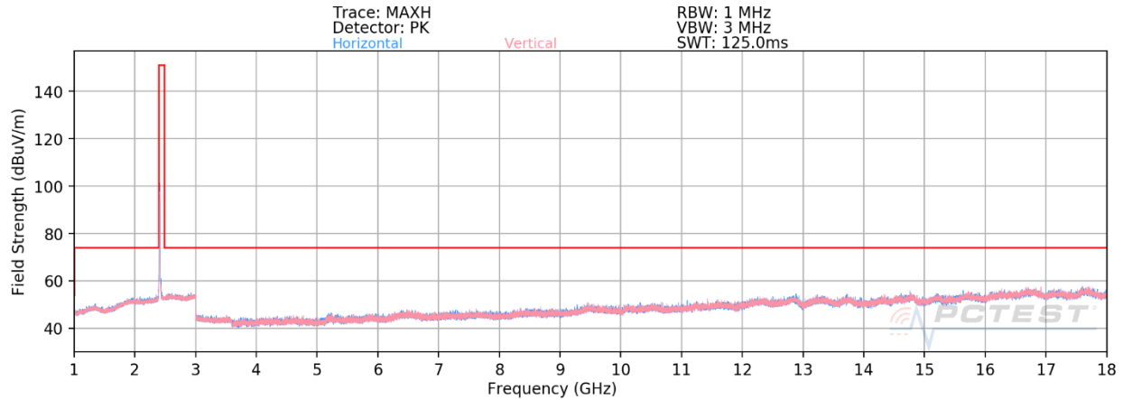
Plot 7-40. Radiated Spurious Emissions 1-18GHz (802.11b – Ch. 1)
