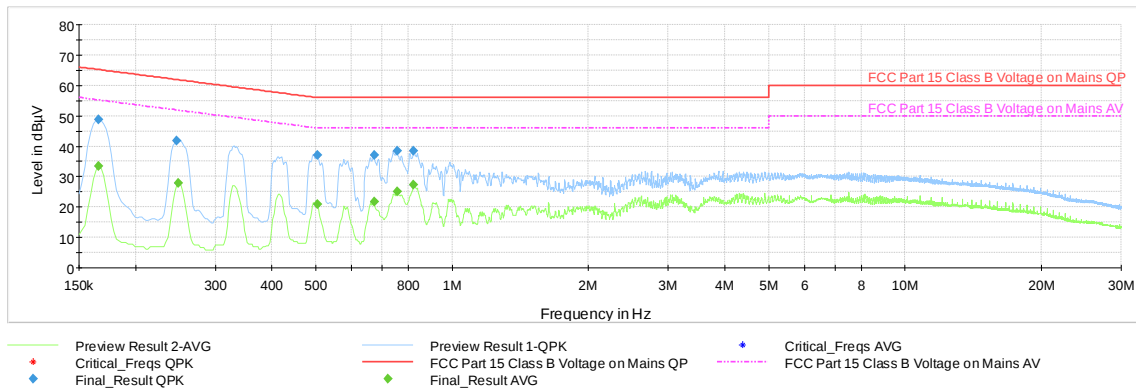
Plot 7-56. AC Line Conducted Emission with 802.11b Ch.6 (N, with WCP + AC/DC Adapter)
