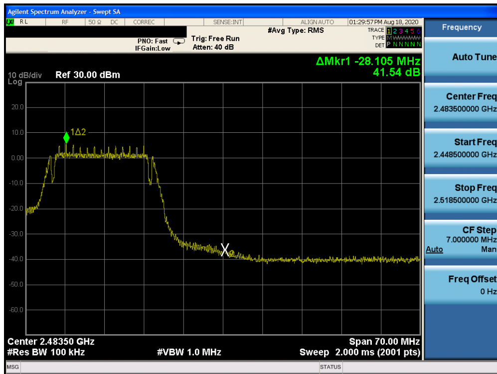
Plot 7-25. Band Edge Plot (802.11g - Ch. 11)
