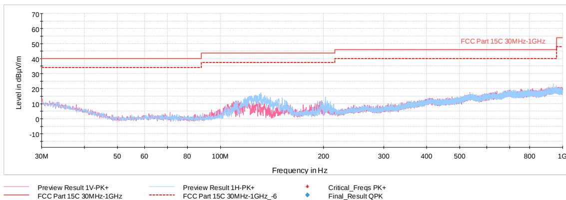
Plot 7-54. Radiated Spurious Emissions 30MHz-1GHz (802.11b – Ch.6, with WCP + laptop)
