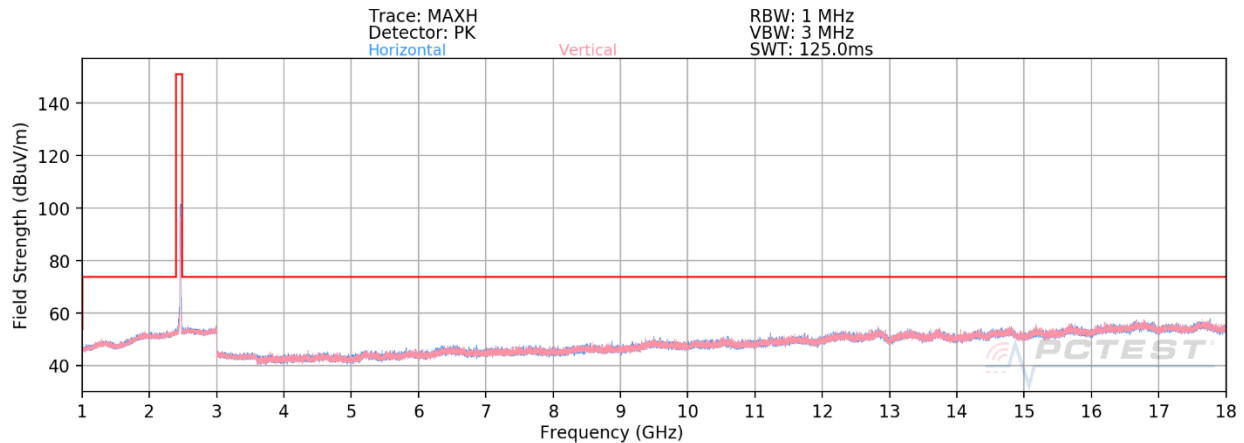
Plot 7-42. Radiated Spurious Emissions 1-18GHz (802.11b – Ch. 11)
