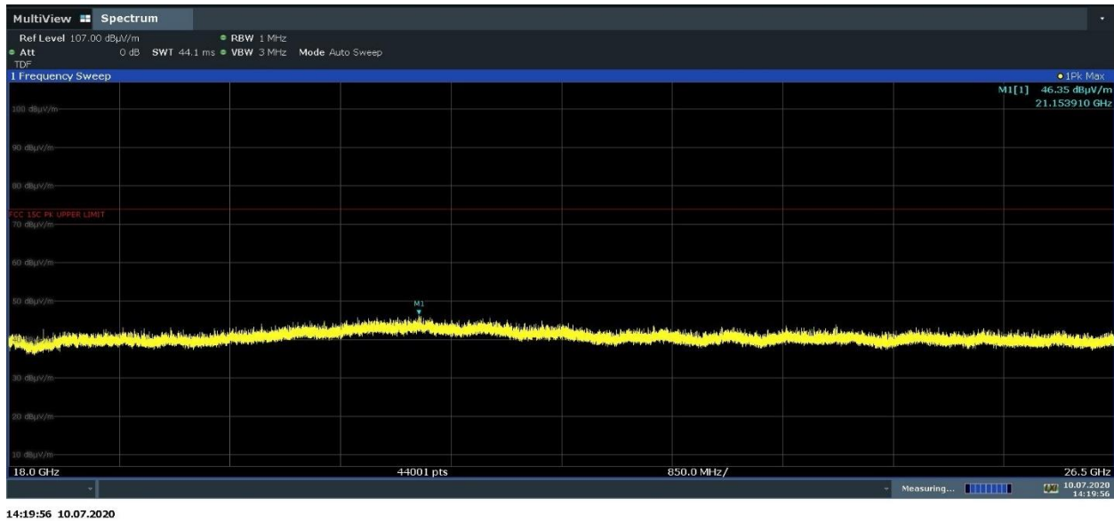
Plot 7-44. Radiated Spurious Emissions 18-26.5GHz (802.11b – Ch. 6, Ant. Pol. V)
