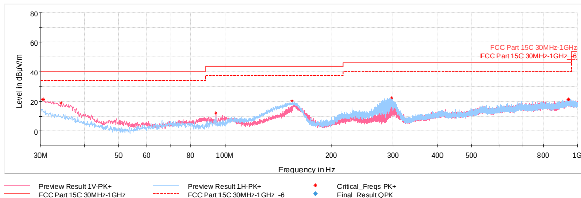
Plot 7-38. Radiated Spurious Emissions 30MHz-1GHz (1Mbps, ePA – Ch.19, with WCP + AC/DC adapter)
