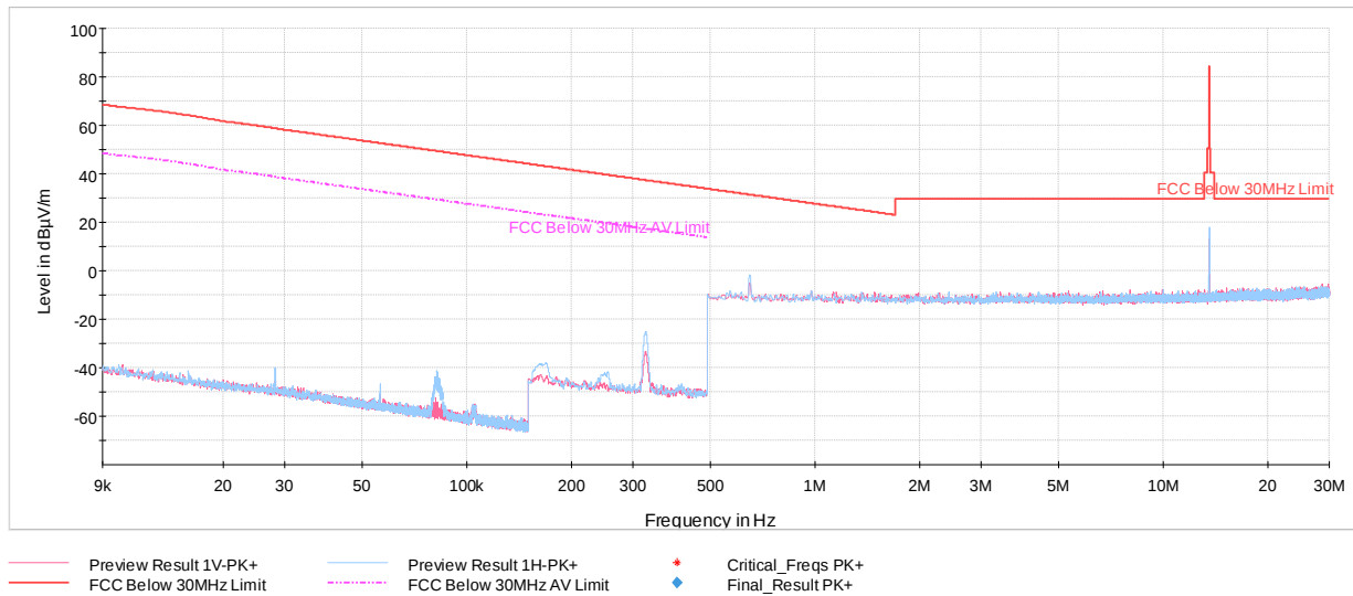
Plot 7-8. Radiated Spurious Emissions 9kHz – 30MHz (CE A 848kbps, with WCP + AC/DC Adapter)
