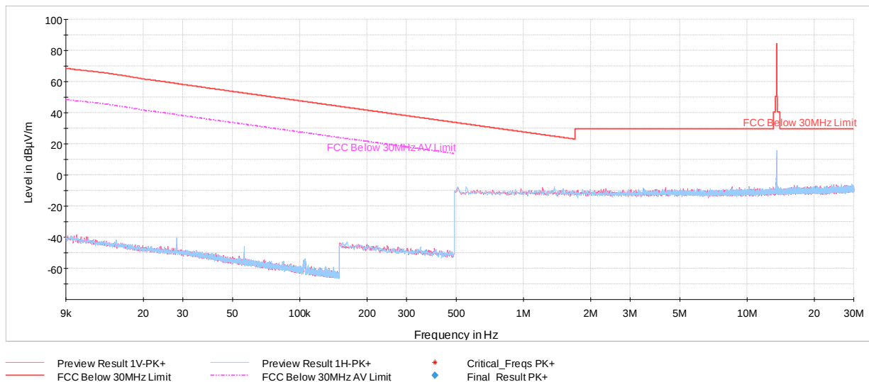
Plot 7-9. Radiated Spurious Emissions 9kHz – 30MHz (Reader 10% Ask 1 out of 256, with WCP + AC/DC Adapter)
