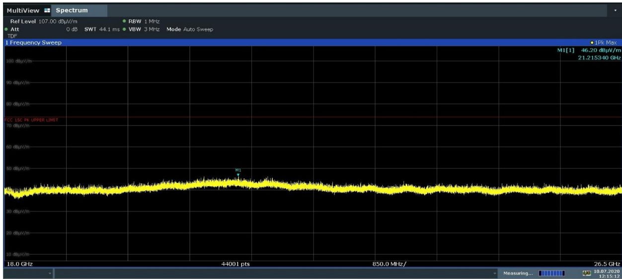
Plot 7-33. Radiated Spurious Emissions 18-26.5GHz (BT GFSK ePA – Ch.39, Pol. V)
