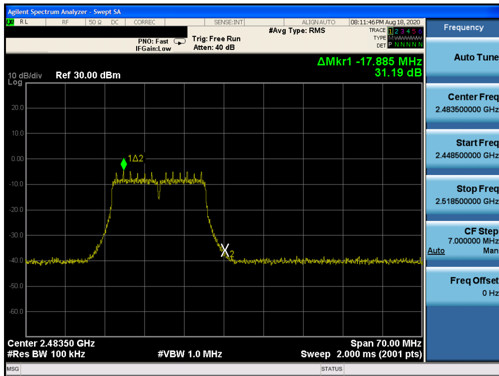
Plot 7-28. Band Edge Plot (802.11g – Ch. 13)
