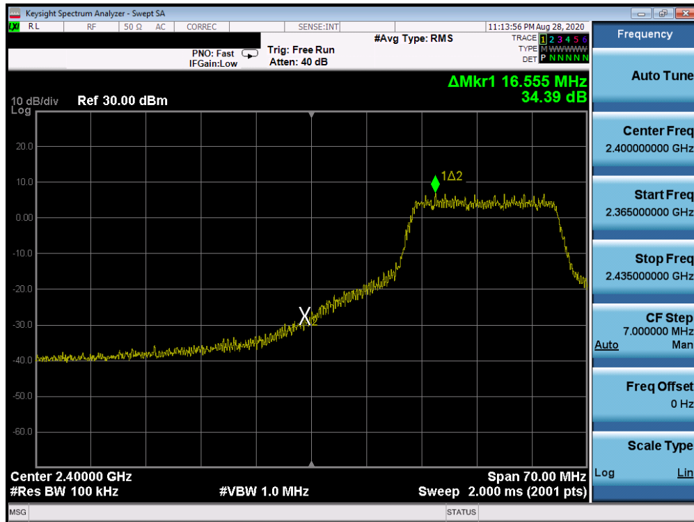
Plot 7-31. Band Edge Plot (802.11n (2.4GHz) – Ch. 3)
