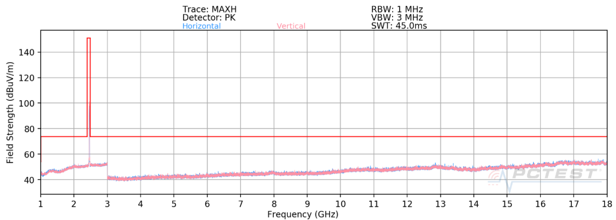
Plot 7-44. Radiated Spurious Emissions 1-18GHz (802.11b – Ch. 11)
