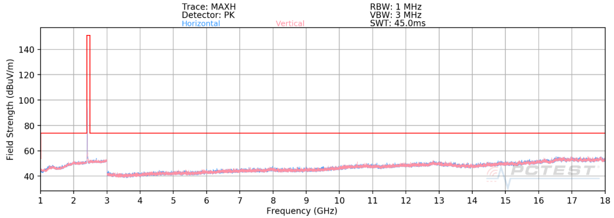
Plot 7-42. Radiated Spurious Emissions 1-18GHz (802.11b – Ch. 1)
