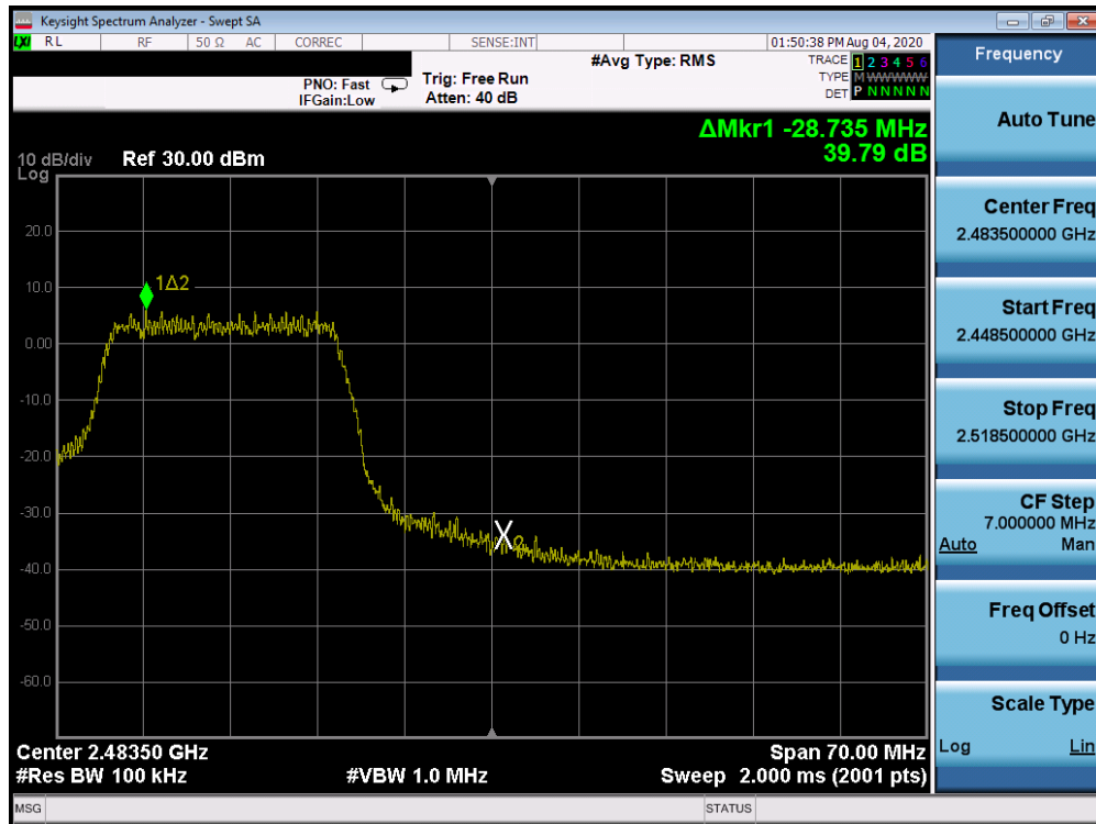
Plot 7-33. Band Edge Plot (802.11n (2.4GHz) – Ch. 11)
