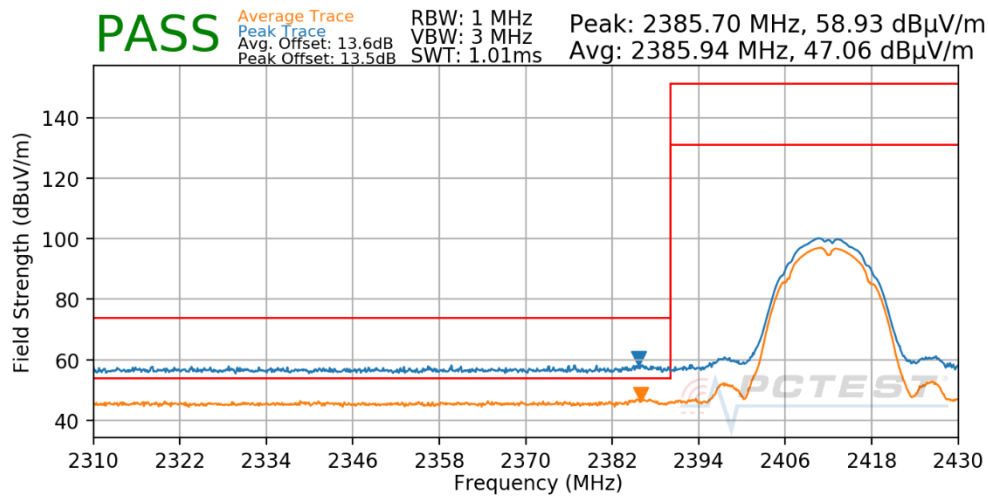
Plot 7-47. Radiated Restricted Lower Band Edge Measurement
