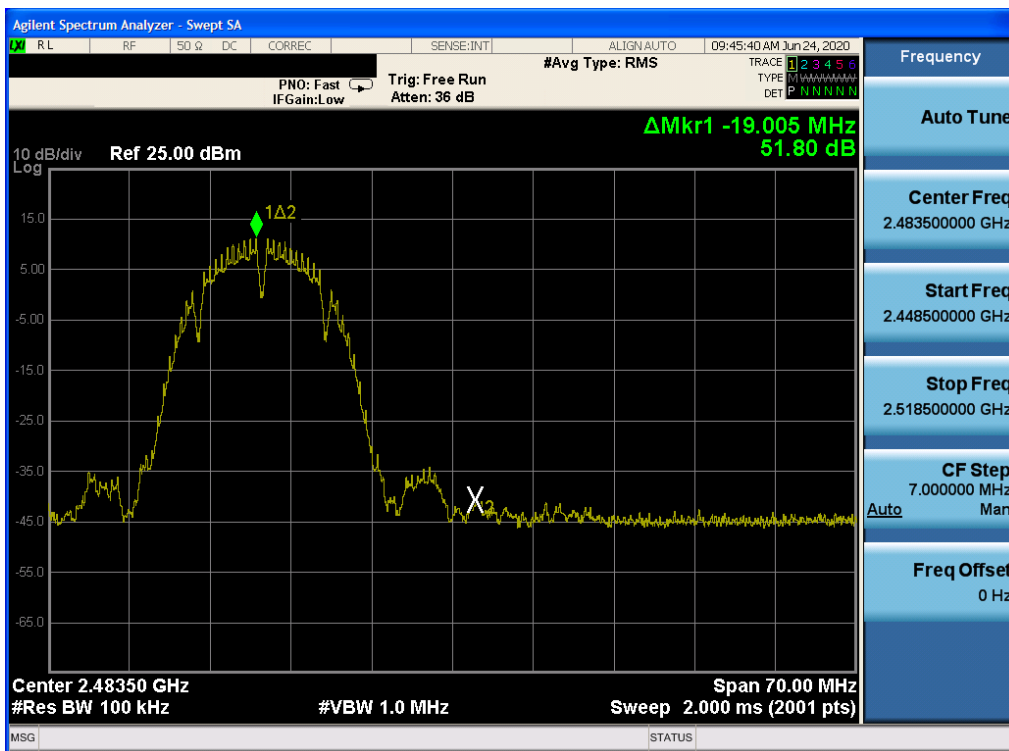
Plot 7-20. Band Edge Plot (802.11b – Ch. 12)
