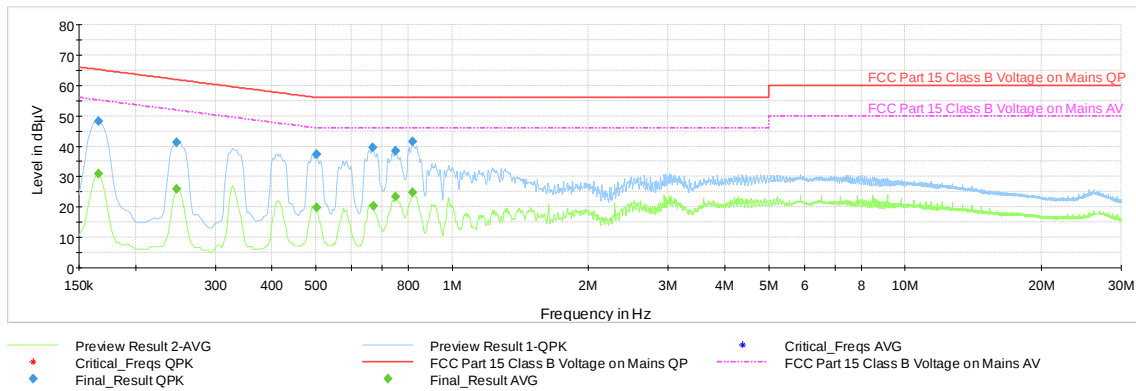
Plot 7-58. AC Line Conducted Emission with 802.11b Ch.11 (L1, with WCP + AC/DC adapter)
