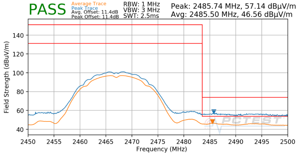
Plot 7-48. Radiated Restricted Upper Band Edge Measurement
