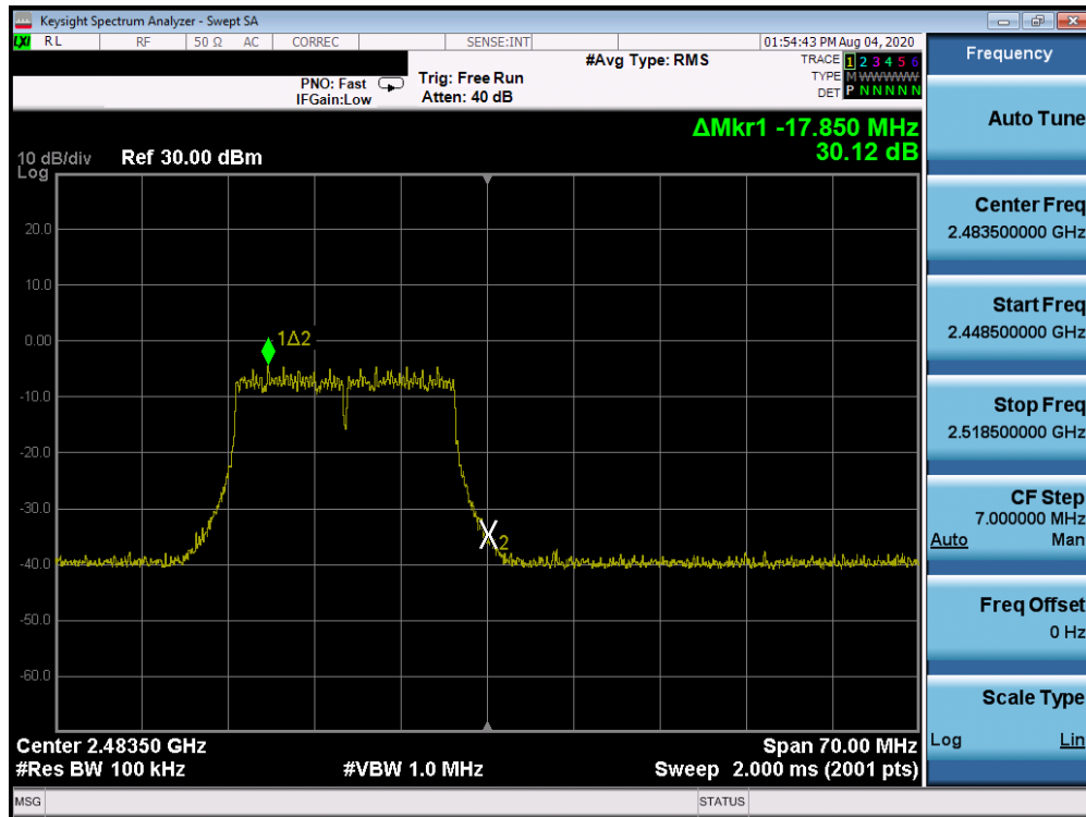
Plot 7-35. Band Edge Plot (802.11n (2.4GHz) – Ch. 13)
