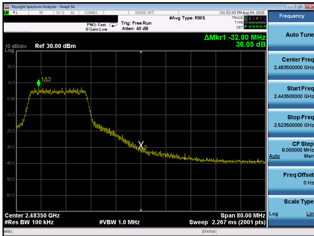
Plot 7-32. Band Edge Plot (802.11n (2.4GHz) – Ch. 10)
