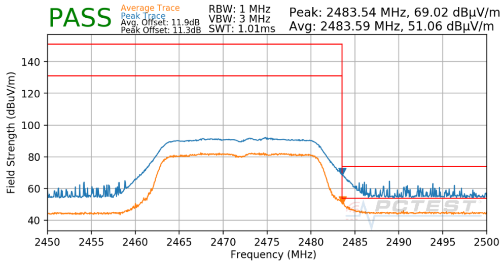
Plot 7-56. Radiated Restricted Upper Band Edge Measurement
