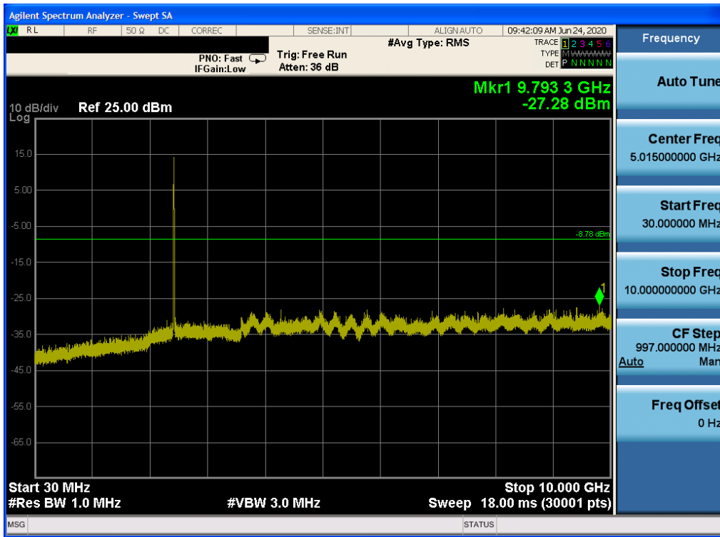
Plot 7-38. Conducted Spurious Plot (802.11b – Ch. 6)
