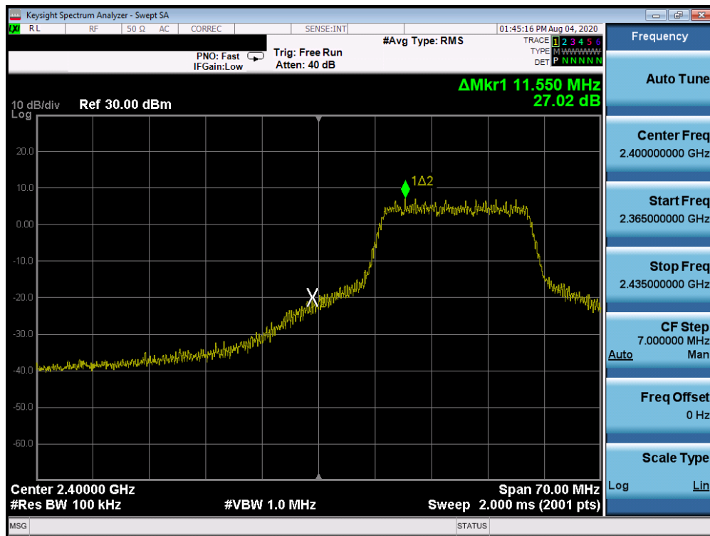
Plot 7-30. Band Edge Plot (802.11n (2.4GHz) – Ch. 2)
