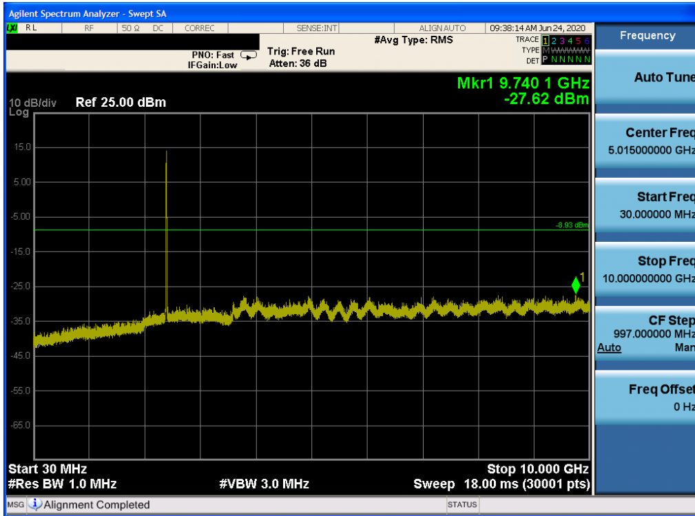
Plot 7-36. Conducted Spurious Plot (802.11b – Ch. 1)
