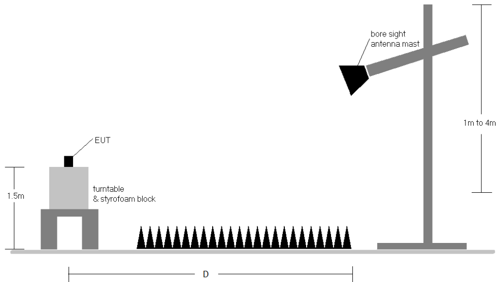
Figure 7-6. Radiated Measurement Setup
