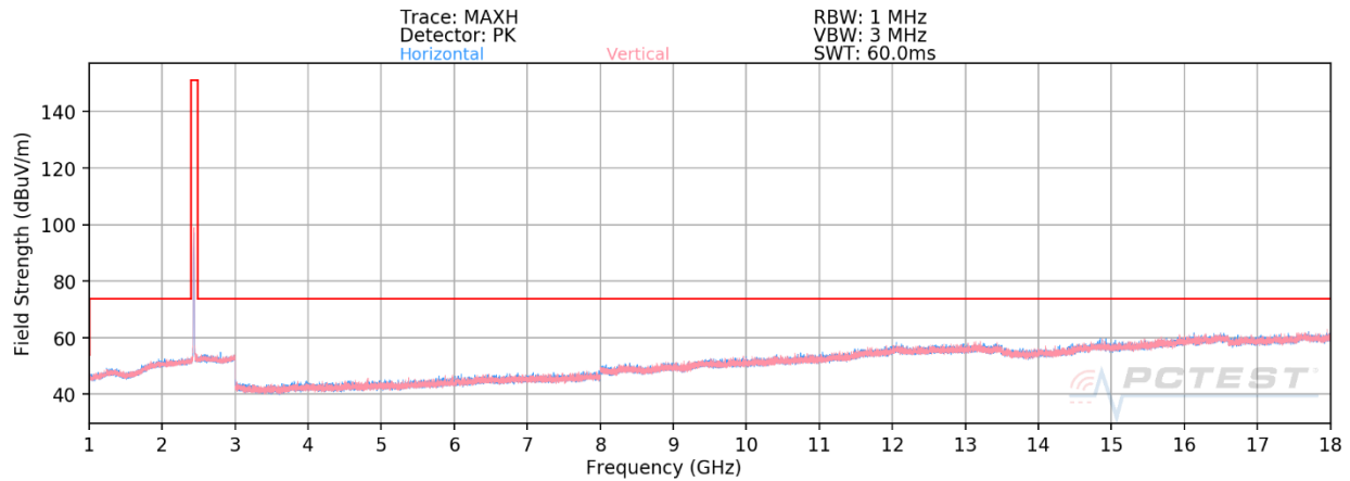
Plot 7-43. Radiated Spurious Emissions 1-18GHz (802.11b – Ch. 6)
