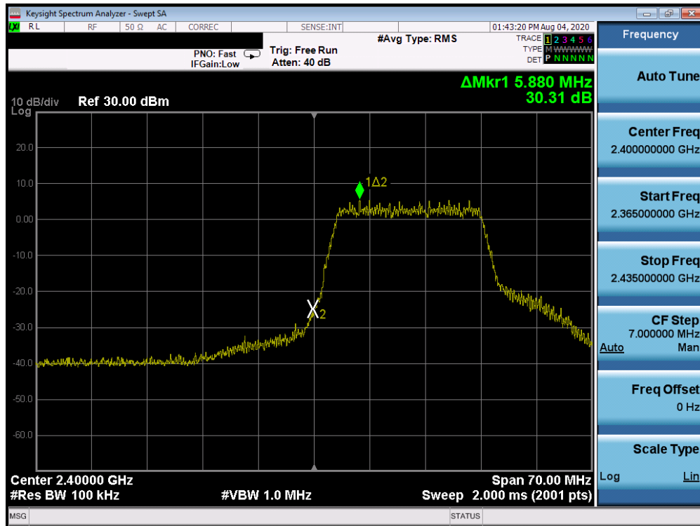
Plot 7-29. Band Edge Plot (802.11n (2.4GHz) – Ch. 1)
