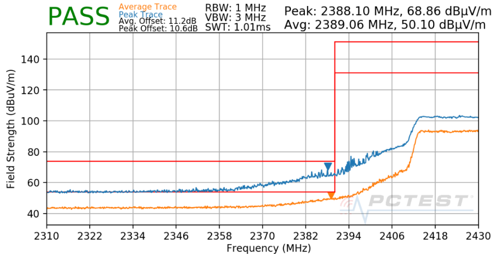
Plot 7-52. Radiated Restricted Lower Band Edge Measurement
