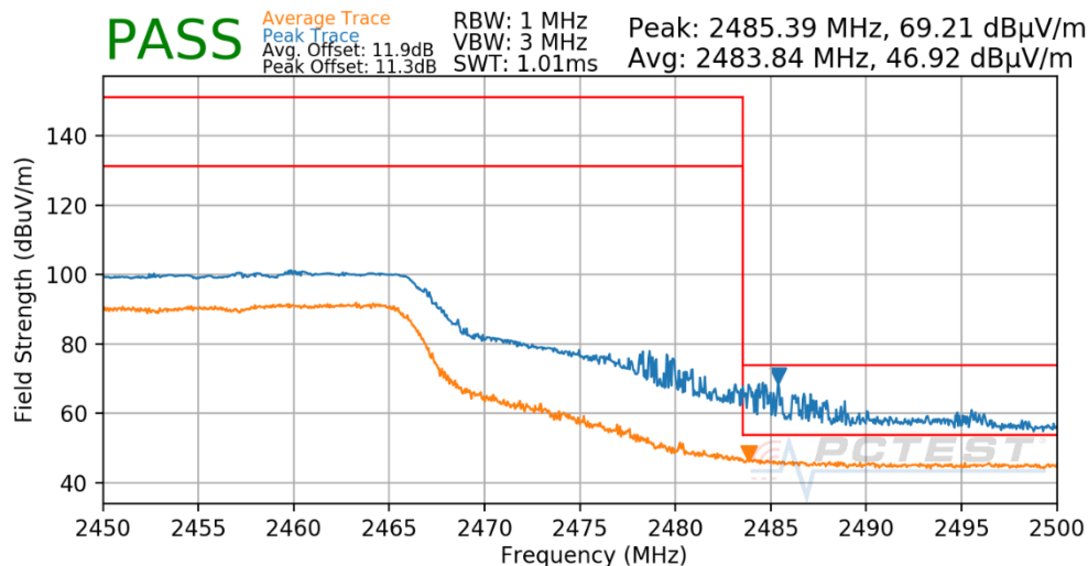
Plot 7-53. Radiated Restricted Upper Band Edge Measurement
