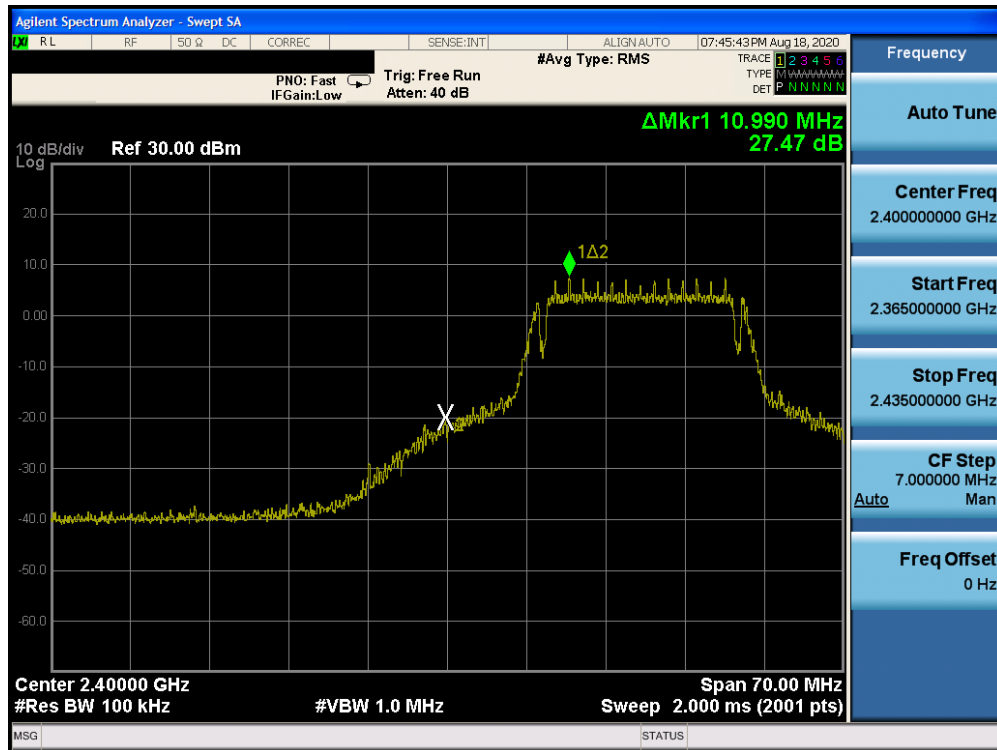
Plot 7-23. Band Edge Plot (802.11g– Ch. 2)
