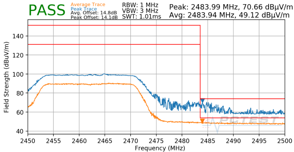
Plot 7-54. Radiated Restricted Upper Band Edge Measurement
