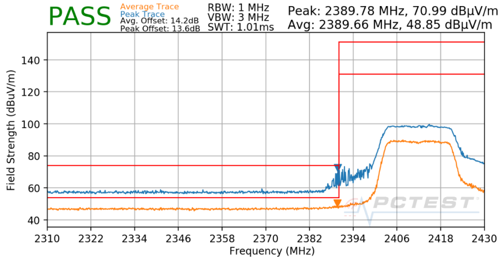
Plot 7-50. Radiated Restricted Lower Band Edge Measurement
