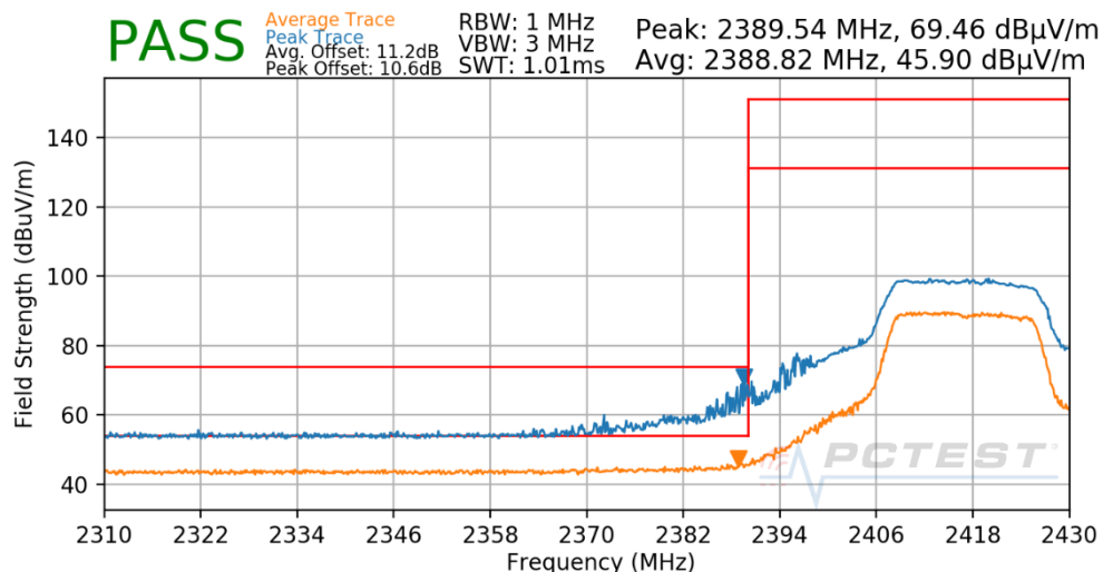
Plot 7-51. Radiated Restricted Lower Band Edge Measurement
