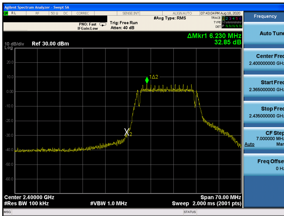
Plot 7-22. Band Edge Plot (802.11g– Ch. 1)
