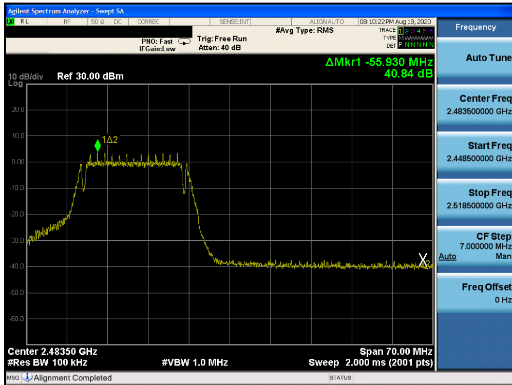
Plot 7-27. Band Edge Plot (802.11g – Ch. 12)
