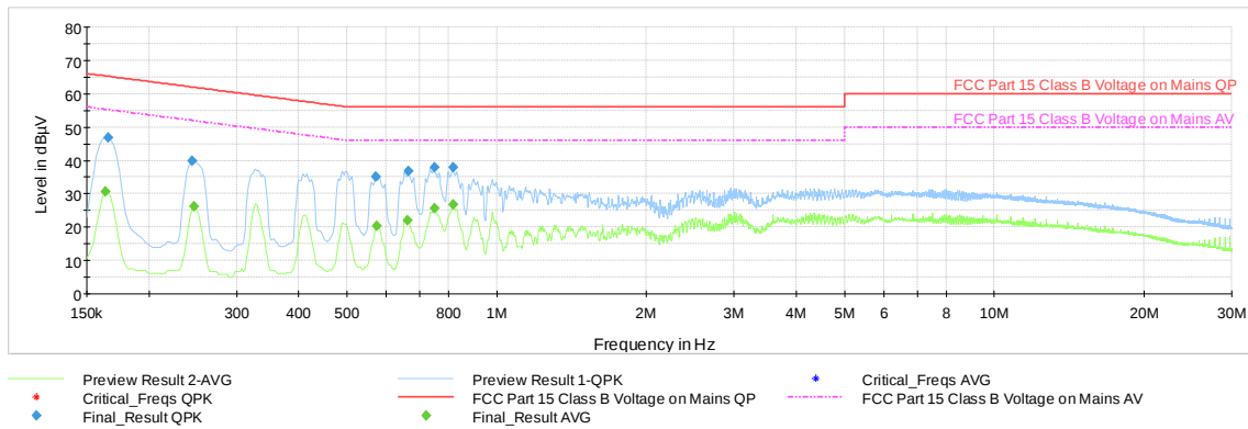
Plot 7-59. AC Line Conducted Emission with 802.11b Ch.11 (N, with WCP + AC/DC adapter)
