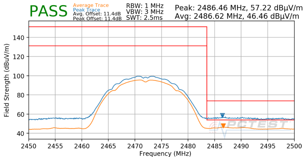
Plot 7-49. Radiated Restricted Upper Band Edge Measurement
