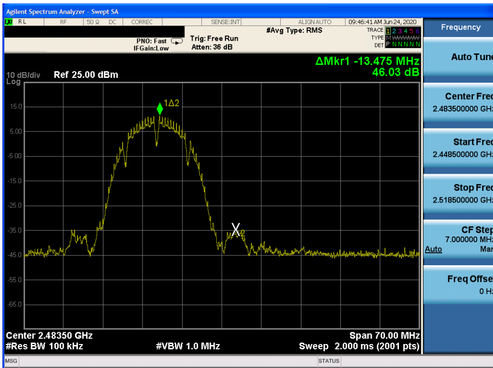
Plot 7-21. Band Edge Plot (802.11b – Ch. 13)
