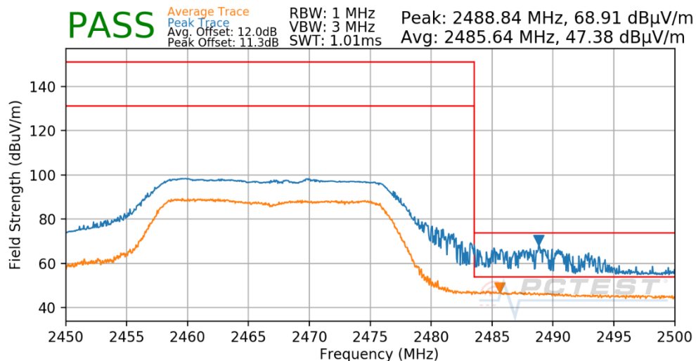
Plot 7-55. Radiated Restricted Upper Band Edge Measurement
