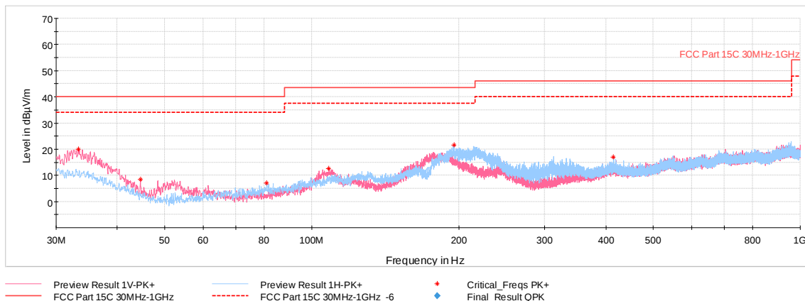
Plot 7-57. Radiated Spurious Emissions 30MHz-1GHz (802.11b – Ch.11, with WCP + AC/DC adapter)
