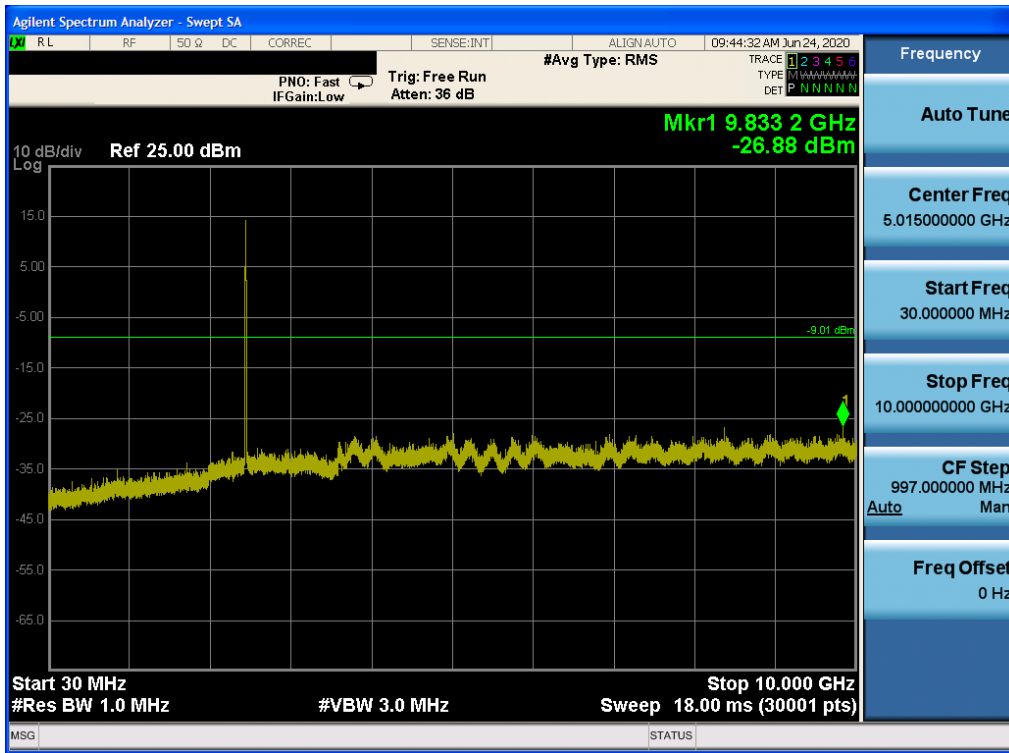
Plot 7-40. Conducted Spurious Plot (802.11b – Ch. 11)
