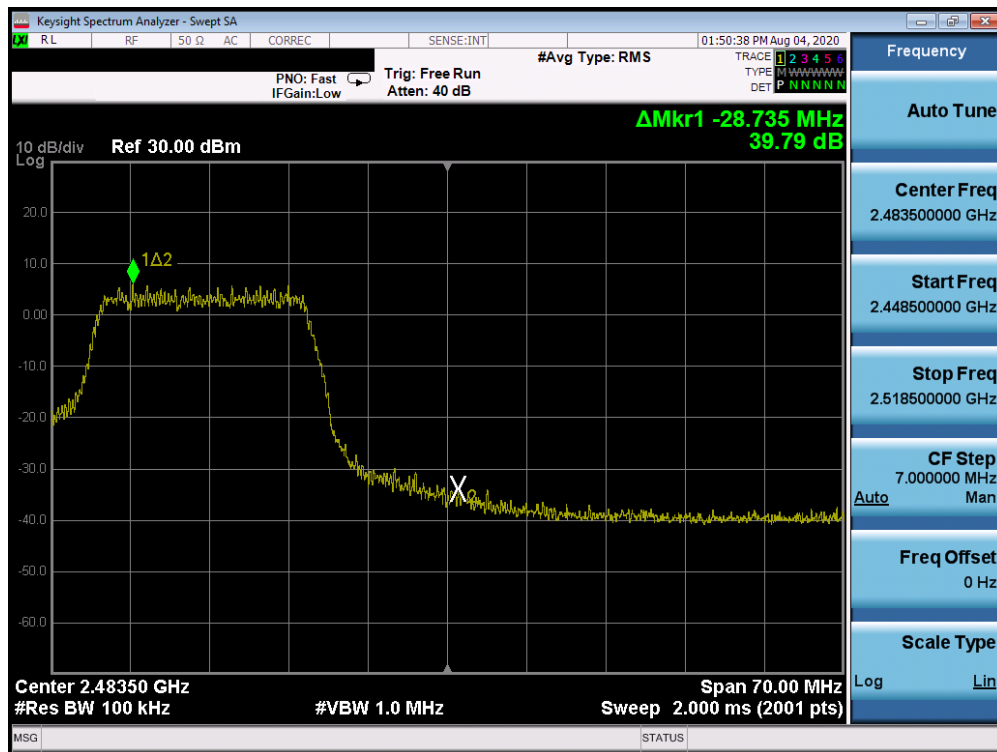
Plot 7-34. Band Edge Plot (802.11n (2.4GHz) – Ch. 12)
