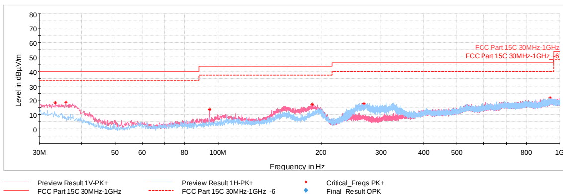
Plot 7-38. Radiated Spurious Emissions 30MHz-1GHz (1Mbps, ePA – Ch.39, with WCP + AC/DC adapter)
