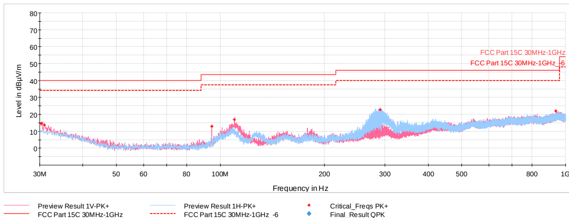
Plot 7-38. Radiated Spurious Emissions 30MHz-1GHz (4Mbps, ePA – Ch.38, with WCP + AC/DC adapter)
