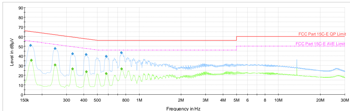
Plot 7-13. AC Line-Conducted Test Plot (N, CE A 848kbps, with WCP + AC/DC Adapter)
