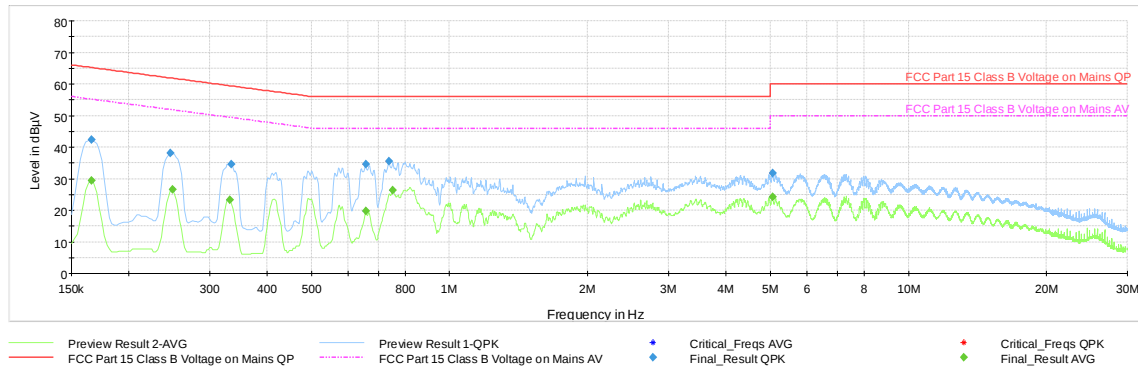
Plot 7-39. AC Line Conducted Emission with GFSK ePA Ch.39 (L1, with WCP + AC/DC adapter)
