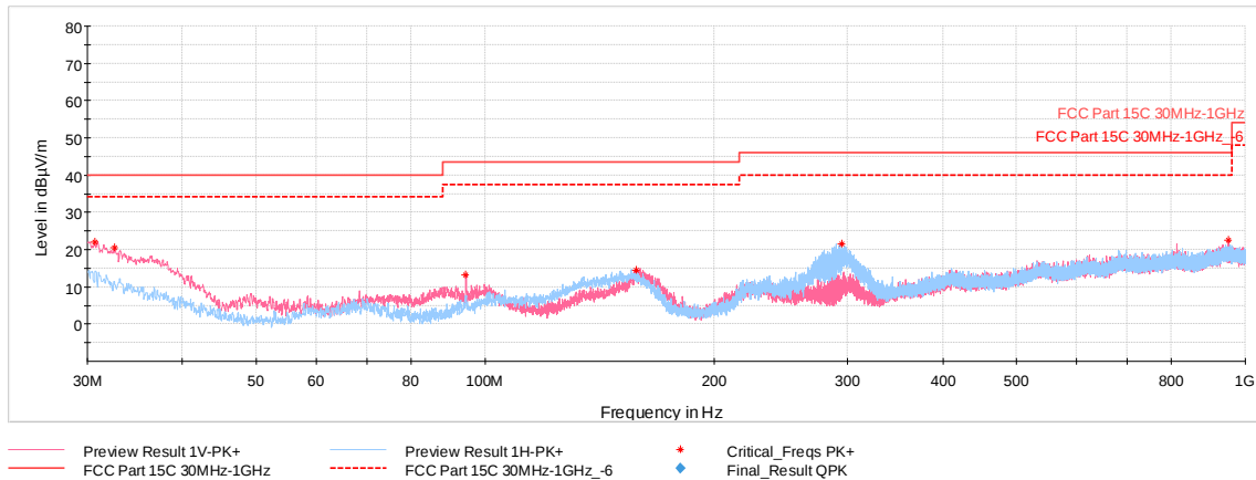
Plot 7-38. Radiated Spurious Emissions 30MHz-1GHz (GFSK ePA – Ch.39, with WCP + AC/DC adapter)
