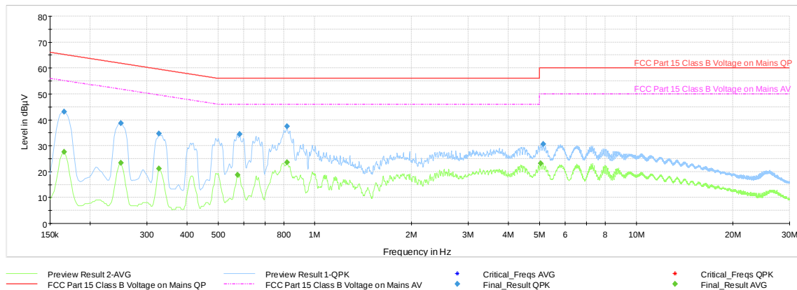
Plot 7-40. AC Line Conducted Emission with GFSK ePA Ch.39 (N, with WCP + AC/DC adapter)
