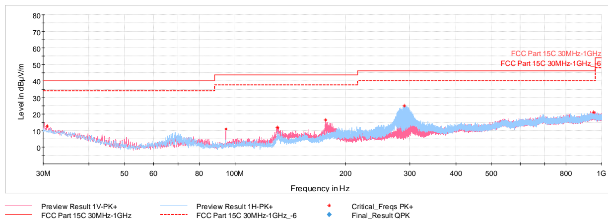
Plot 7-57. Radiated Spurious Emissions 30MHz-1GHz (802.11b – Ch.11, with WCP + laptop)
