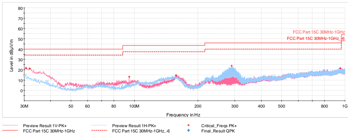
Plot 7-38. Radiated Spurious Emissions 30MHz-1GHz (1Mbps, ePA – Ch.39, with WCP + AC/DC adapter)
