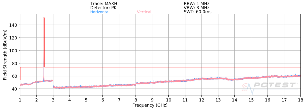
Plot 7-46. Radiated Spurious Emissions 1-18GHz (802.11b – Ch. 6)
