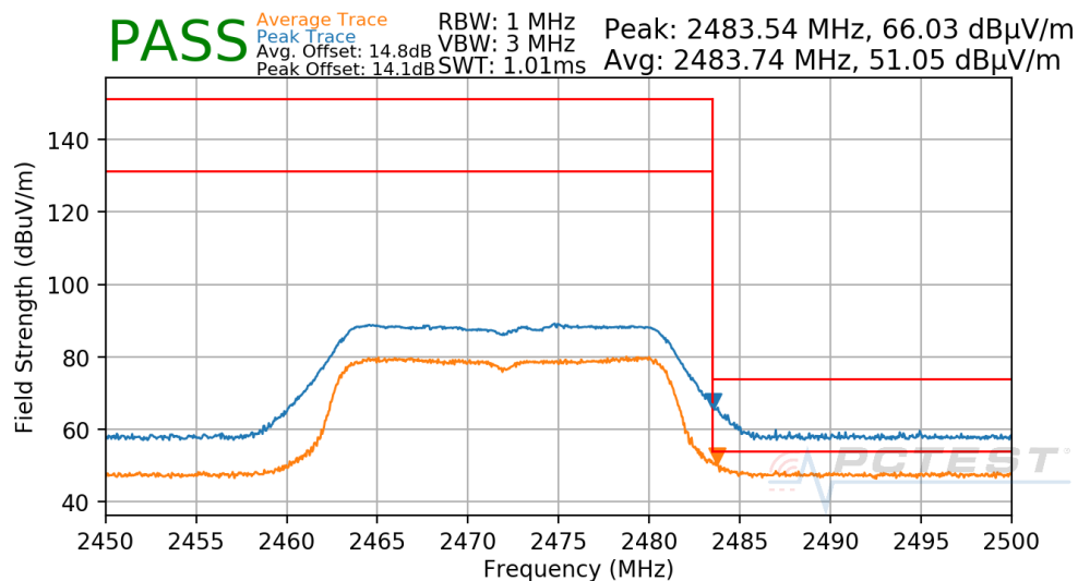
Plot 7-61. Radiated Restricted Upper Band Edge Measurement
