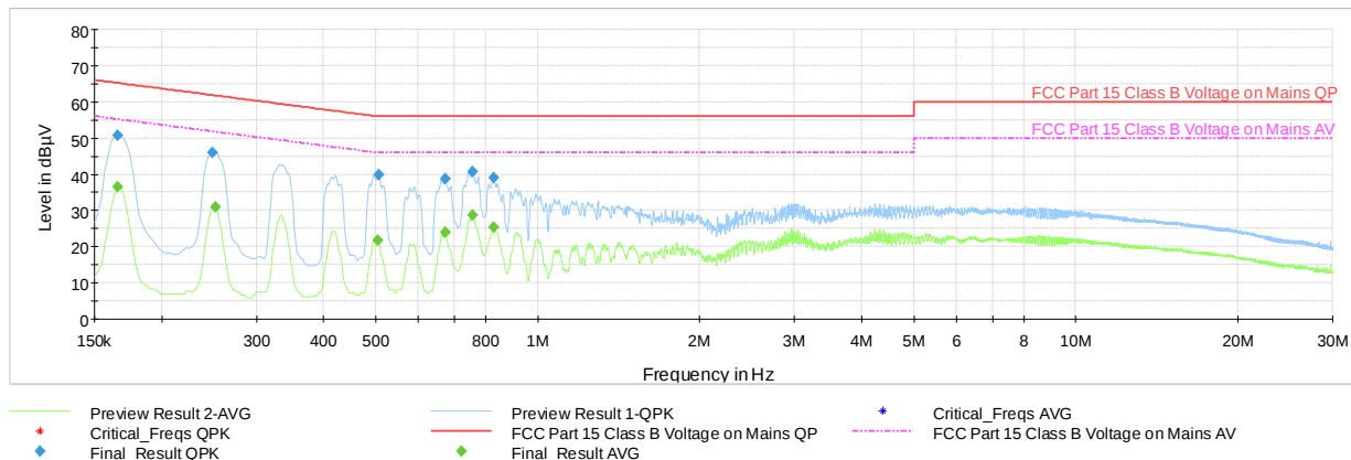
Plot 7-64. AC Line Conducted Plot with 802.11b Ch.6 (N, with WCP + AC/DC Adapter)
