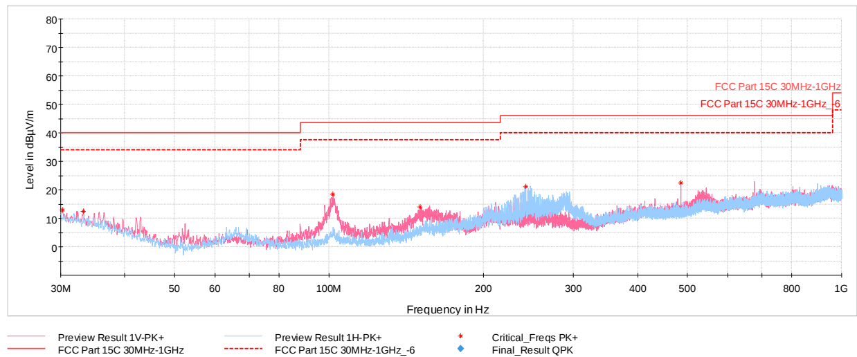
Plot 7-62. Radiated Spurious Emissions 30MHz-1GHz (802.11b – Ch.6, with WCP + laptop)
