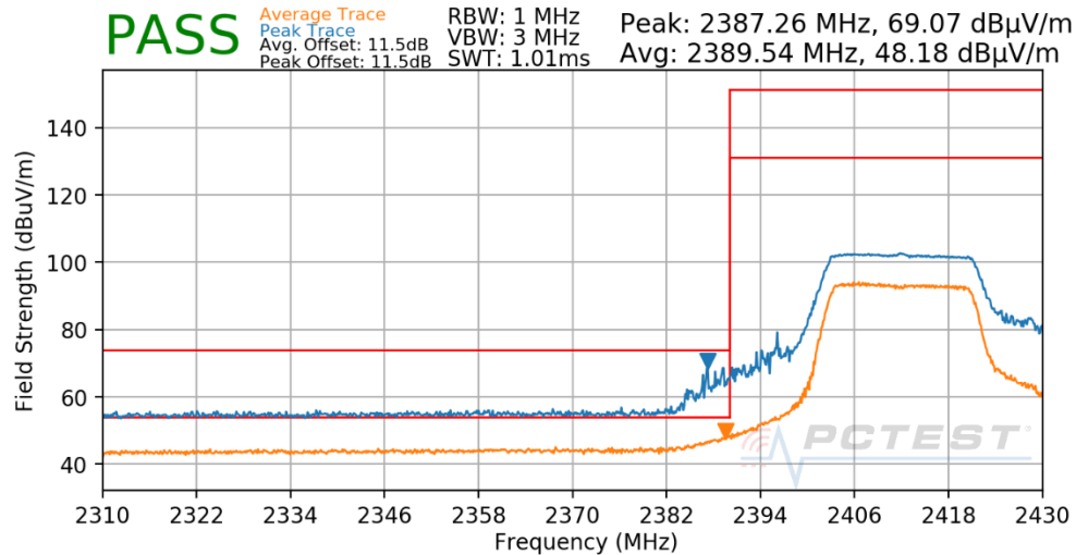
Plot 7-54. Radiated Restricted Lower Band Edge Measurement
