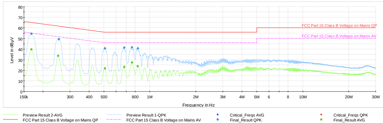
Plot 7-63. AC Line Conducted Plot with 802.11b Ch.6 (L1, with WCP + AC/DC Adapter)
