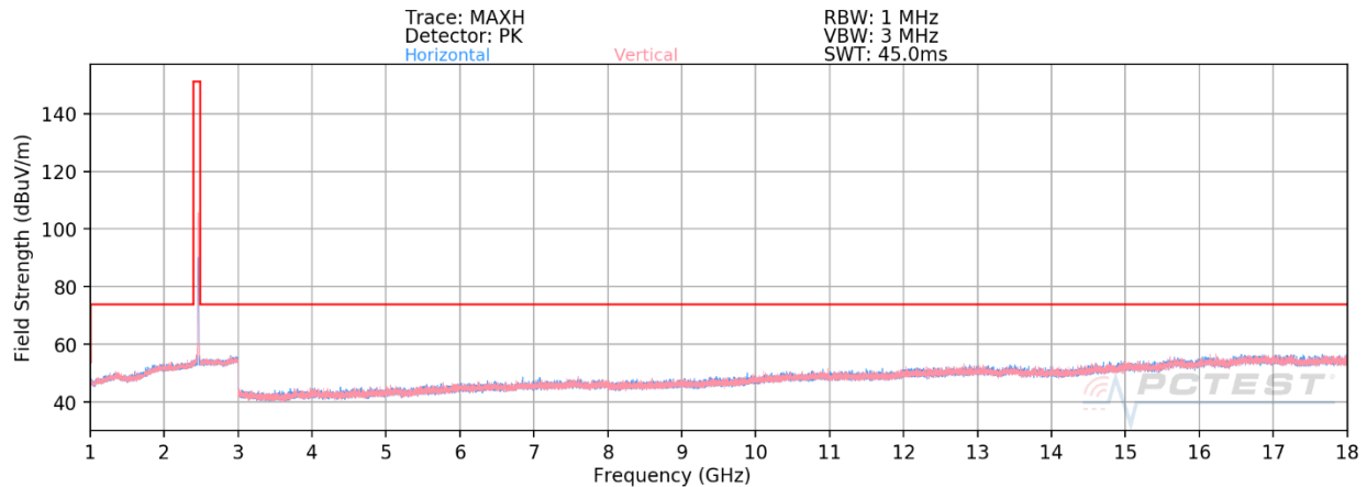
Plot 7-47. Radiated Spurious Emissions 1-18GHz (802.11b – Ch. 11)
