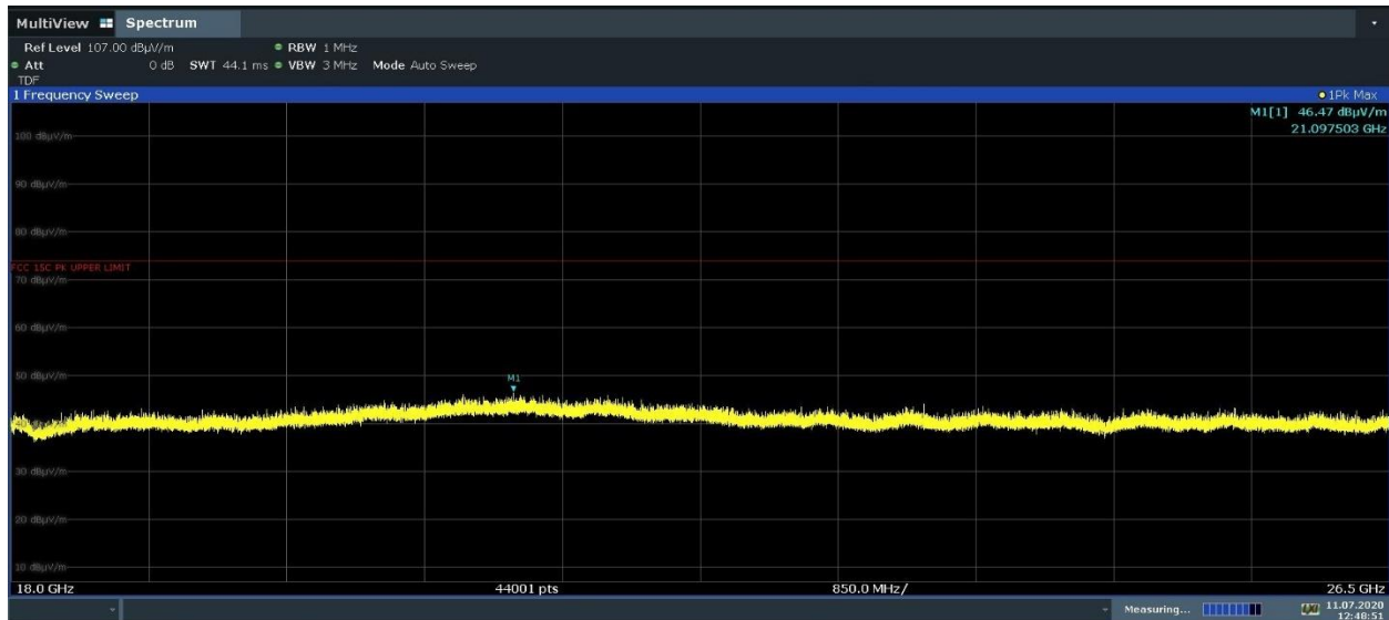
Plot 7-49. Radiated Spurious Emissions 18-26.5GHz (802.11b – Ch. 6, Ant. Pol. V)
