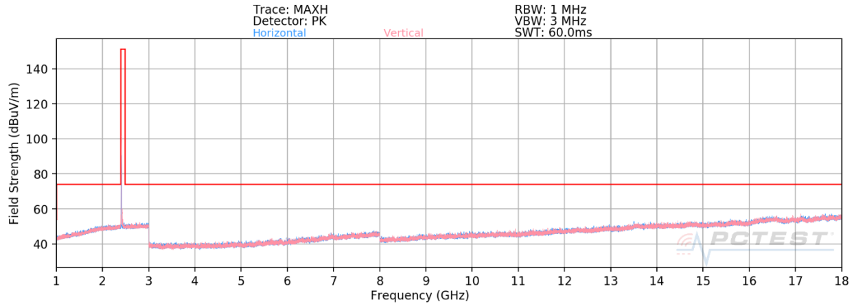
Plot 7-45. Radiated Spurious Emissions 1-18GHz (802.11b – Ch. 1)
