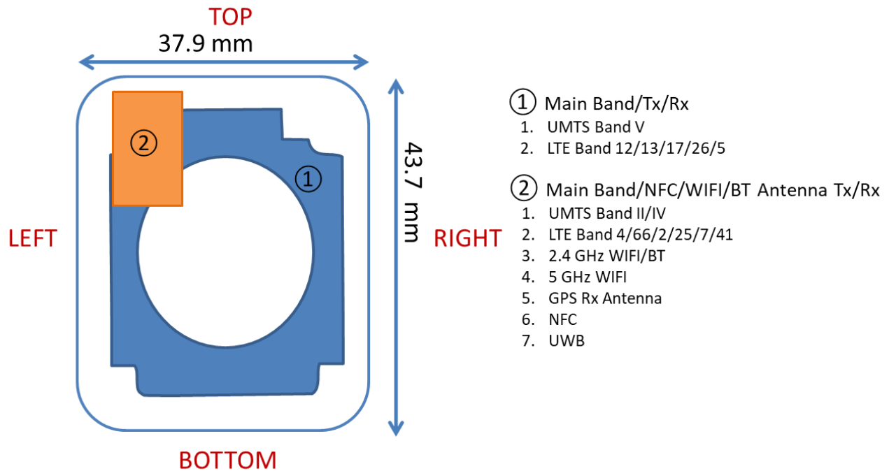
Figure E-1 DUT Antenna Locations
