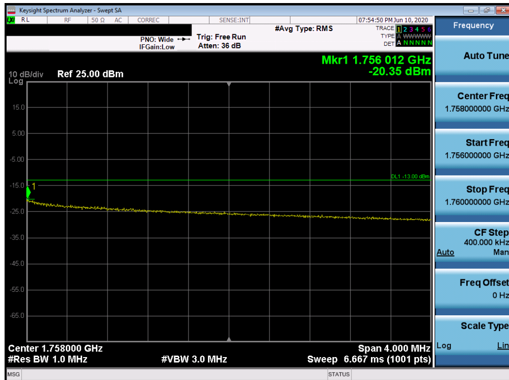
Plot 7-199. Upper Extended Band Edge Plot (Band 4 - 10.0MHz QPSK - Full RB Configuration)
